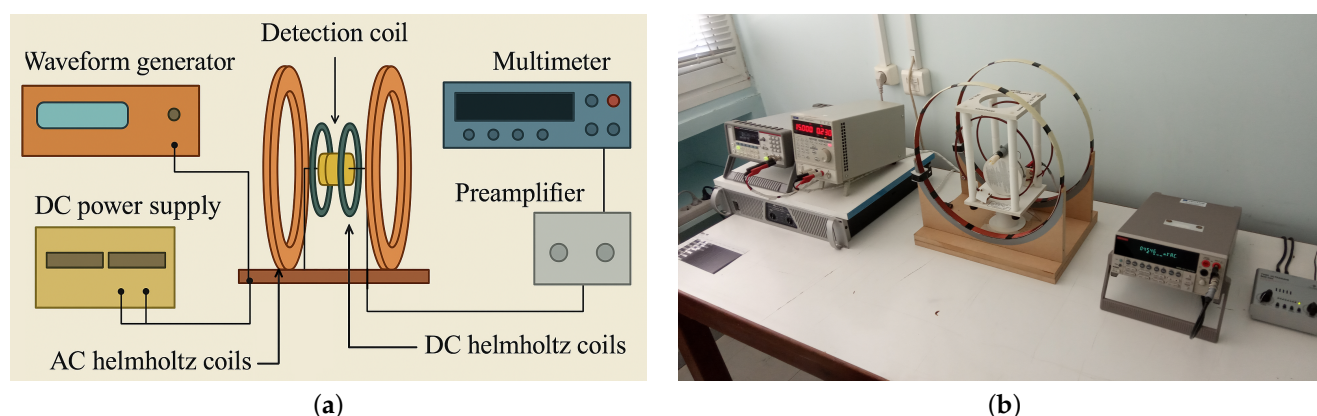
Figure 3. Experimental setup used for magnetoelastic signal measurement: (a) schematic diagram and (b) actual setup.
