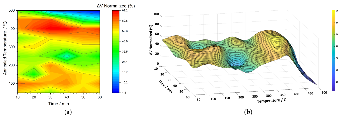
Figure 6. (a) a 2D color map and (b) a 3D surface plot of normalized \Delta V (%) for 2605SA1 ribbons as a function of annealing temperature and time.
