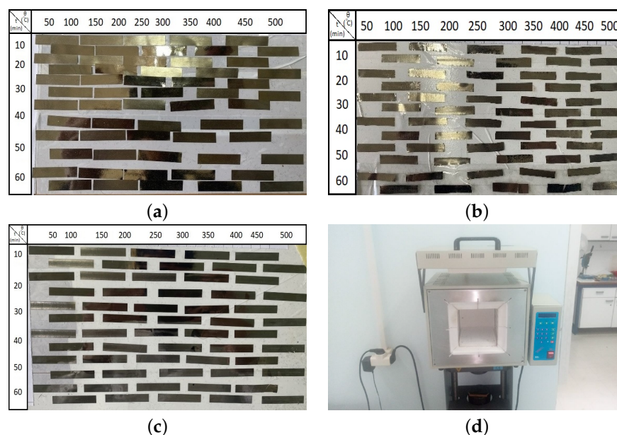
Figure 2. All ribbon specimens prepared for thermal annealing for each Metglas material: (a) Metglas 2826MB3, (b) Metglas 2605SA1, and (c) Metglas 2714A. (d) The furnace used for the annealing process.
