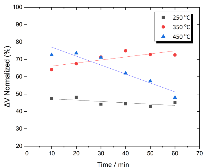
Figure 5. \Delta V as a function of time for Metglas 2826MB3 annealed at three different temperatures.
