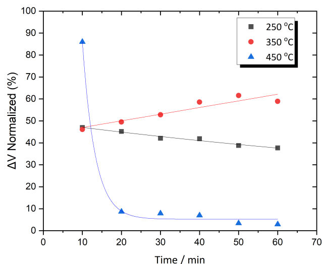
Figure 9. \Delta V as a function of time for Metglas 2714A annealed at three different temperatures.
