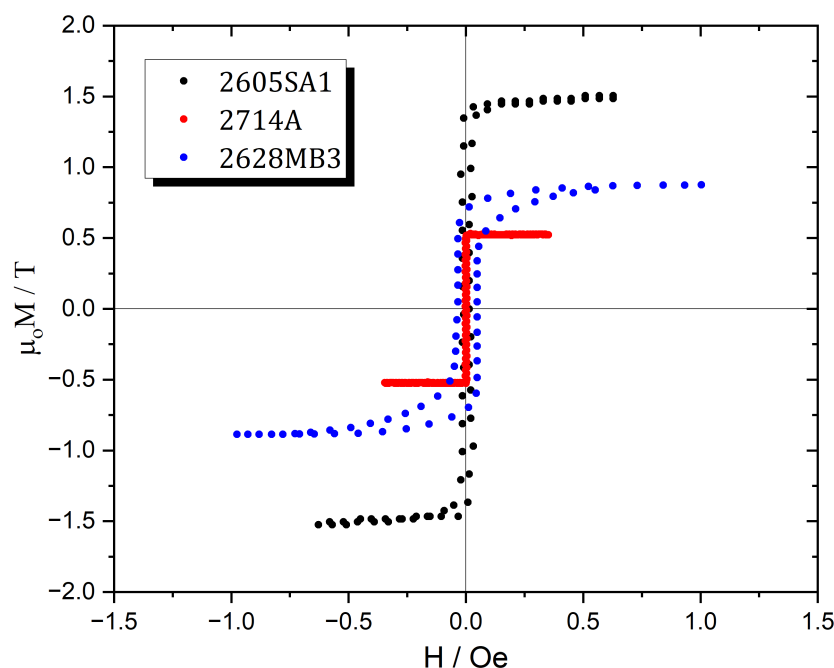
Figure 1. Magnetic hysteresis curves for all tested Metglas materials are presented. These curves correspond to the samples in their as-received state, prior to the annealing process.
