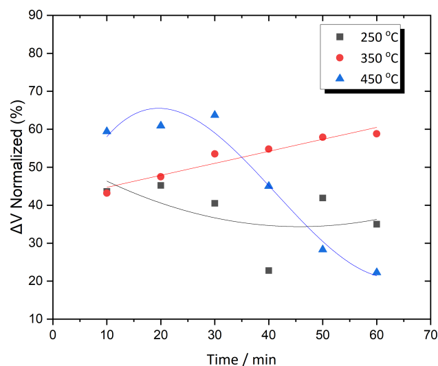
Figure 7. \Delta V as a function of time for Metglas 2605SA1 annealed at three different temperatures.
