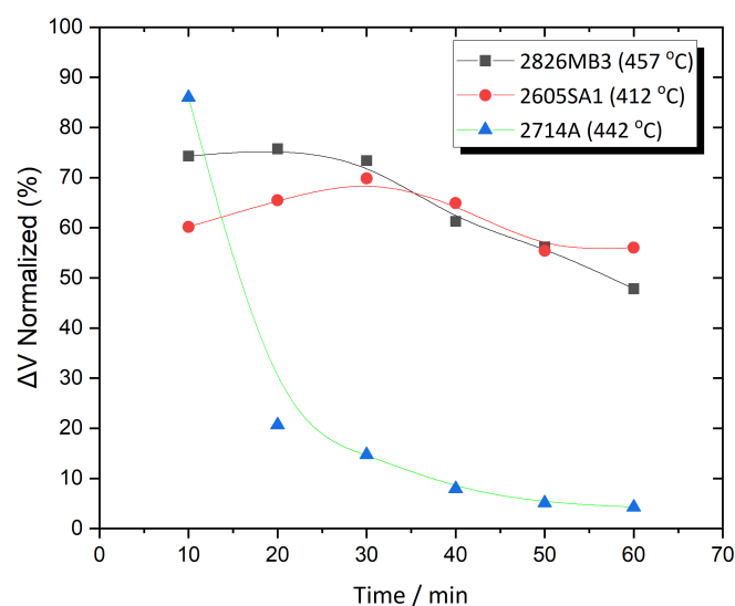
Figure 10. Comparison results: \Delta V as a function of time for all alloys annealed at their respective optimum temperatures.
