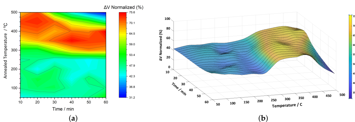
Figure 4. (a) a 2D color map and (b) a 3D surface plot of normalized \Delta V (%) for 2826MB3 ribbons as a function of annealing temperature and time.
