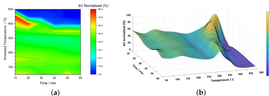
Figure 8. (a) a 2D color map and (b) a 3D surface plot of normalized \Delta V (%) for 2714A ribbons as a function of annealing temperature and time.
