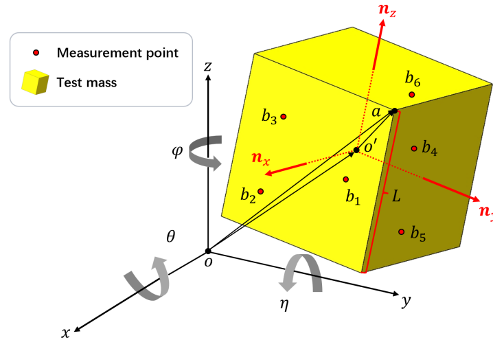
Figure 1. Schematic of the measuring principle. The coordinate system is fixed: the origin o coincides with the geometric center o' of the TM in the initial state and the three axes are perpendicular to the three planes of the TM in the initial state. The deviation between o' and o is the translational displacement of the TM and (\theta, \eta, \varphi) represent the rotational displacement of the TM along the x -, y -, and z -axes.
