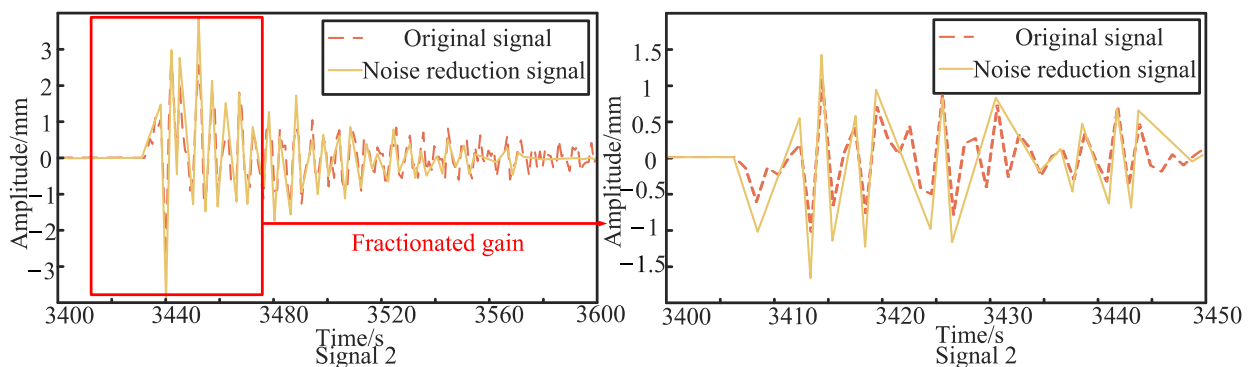
Figure 8. The original signal and noise reduction signal for the asymmetrically arranged signal 2 under the first excitation.
