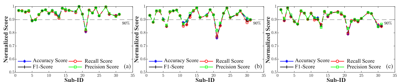
Figure 8. Evaluation metrics computed for each individual employing a fraction of the target subject data set equal to 30% and a diverse number of source subjects (N). A 90% threshold (indicated by the gray dashed line) is used to identify subjects whose performance drops by more than 10% compared to the training phase. (a) N = 5. (b) N = 10. (c) N = 15.
