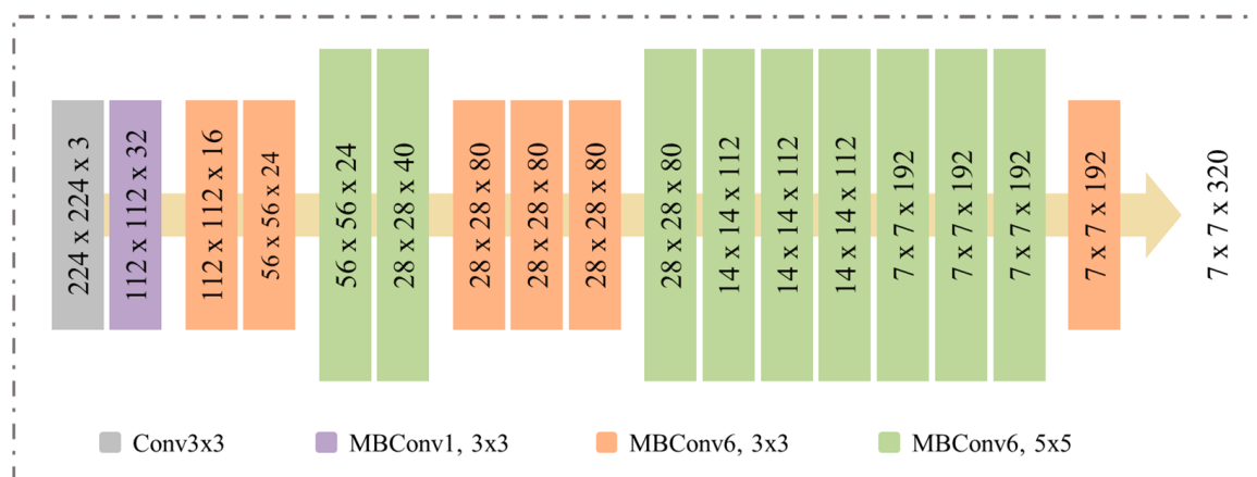
Figure 2. EfficientNetB0 architecture.
