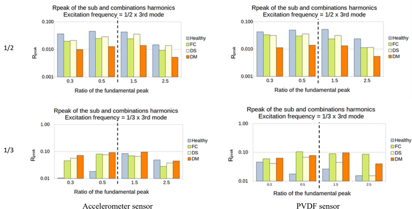
Figure 18. Third natural frequency and its ratio of 1, 1/2 , and 1/3 as the frequency of excitation.
