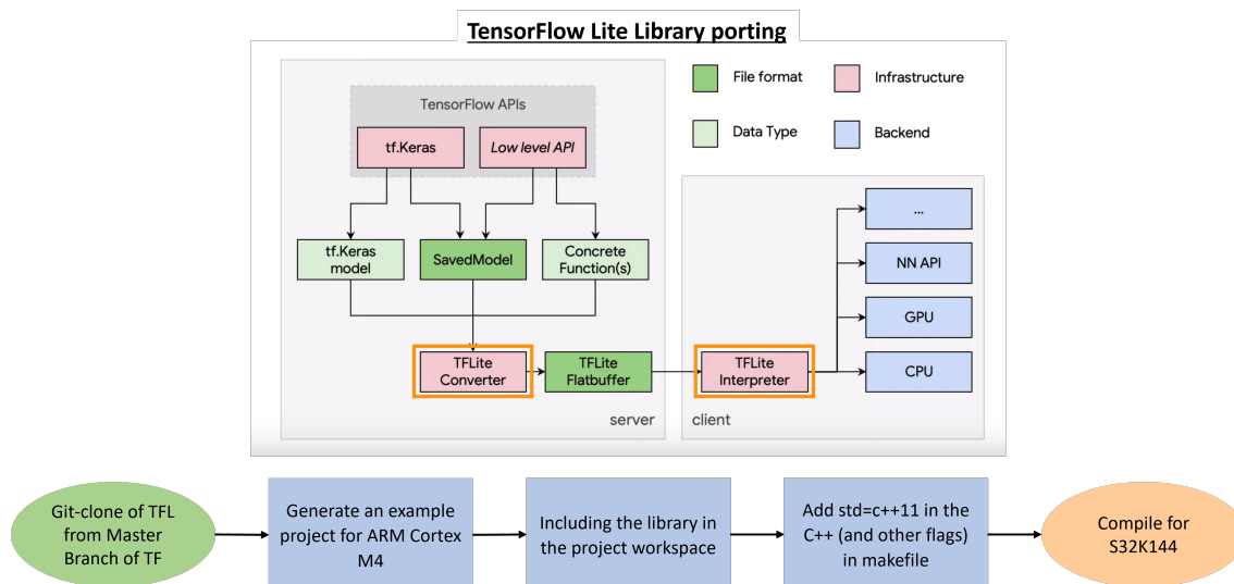
Figure 9. Flow chart of TensorFlow Lite porting Library.
