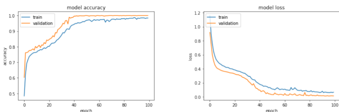
Figure 14. Learning curve of accuracy (left) + Learning curve of loss (right) for the Second Test.
