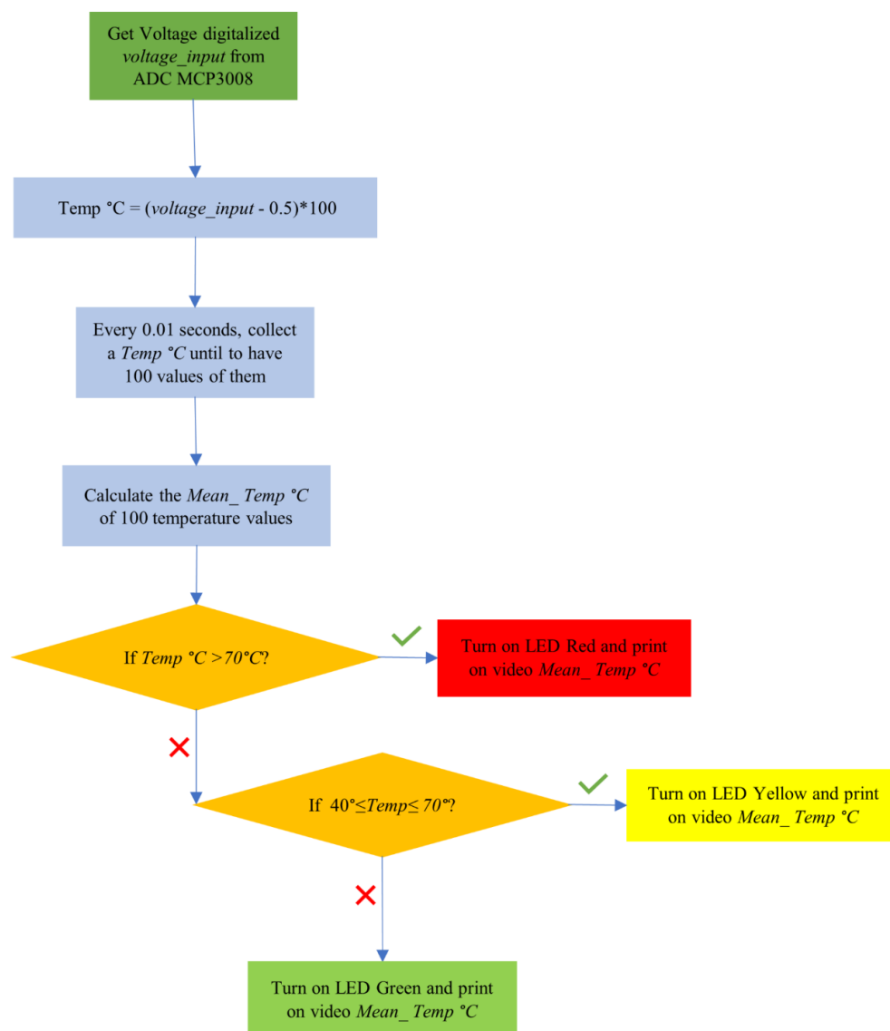
Figure 18. Thermal test procedure deployed on RaspberryPi3B+.
