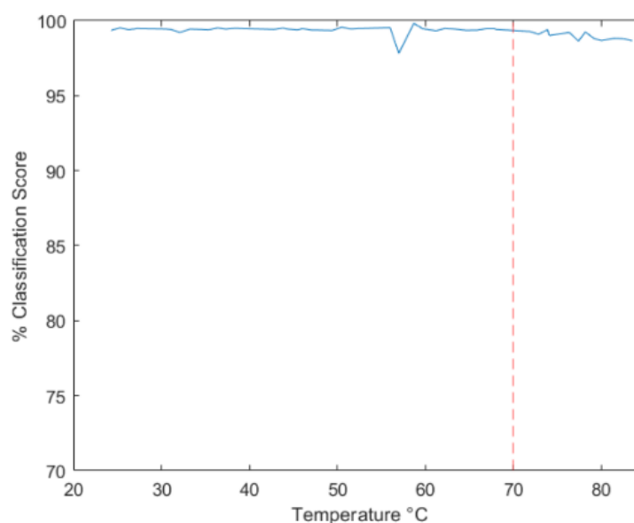
Figure 20. Classification result as a function of temperature.
