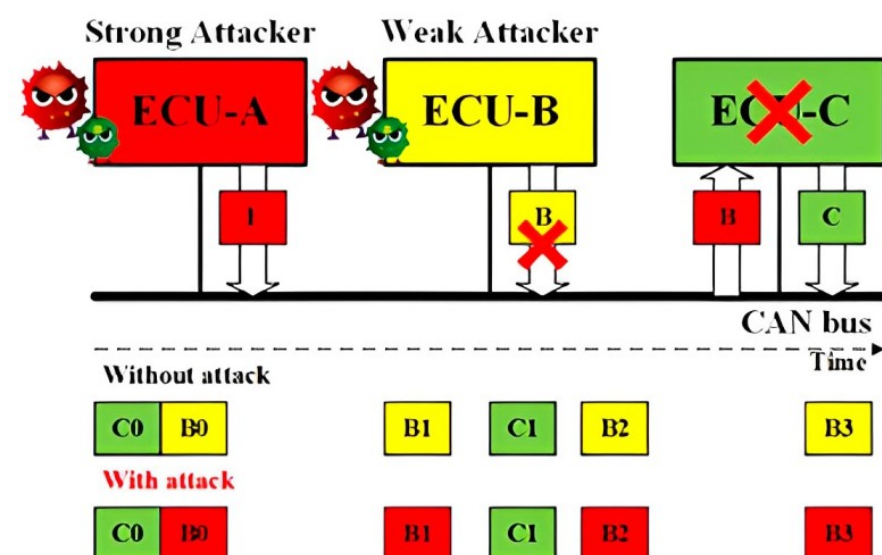
Figure 2. Schematic representation of the Impersonation attack concept.
