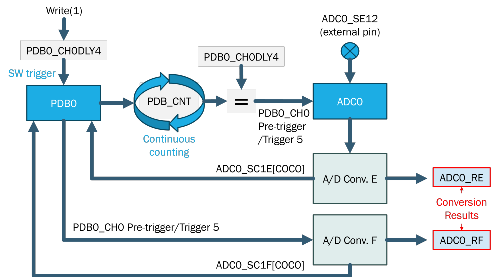
Figure 4. ADC Hardware Trigger with PDB in back-to-back mode.
