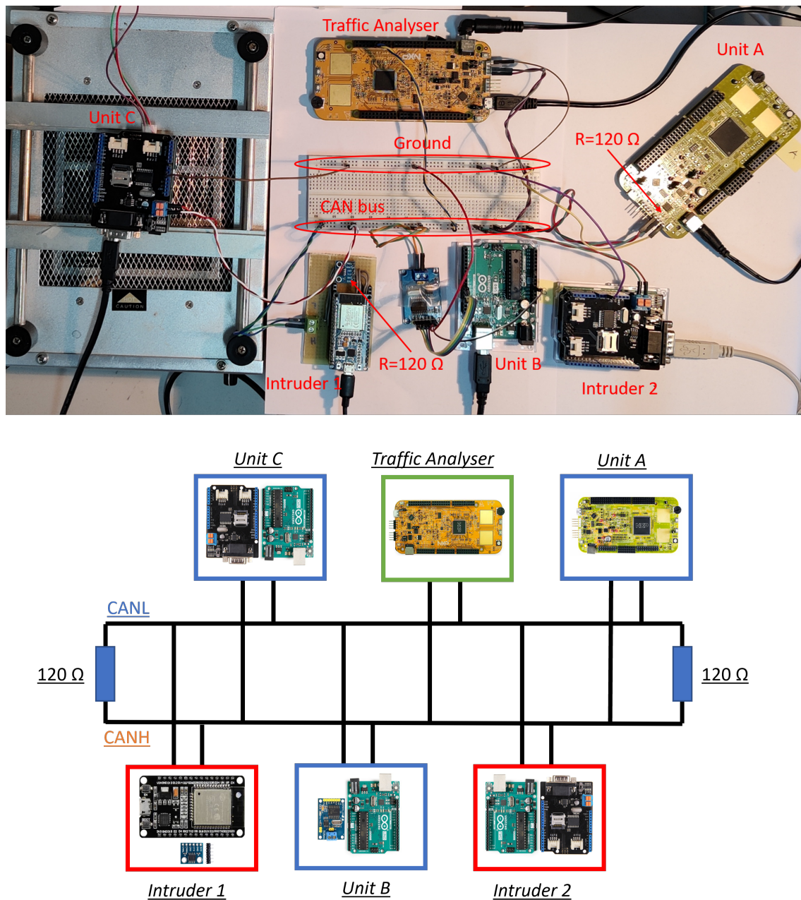
Figure 10. Experimental Setup CAN circuit.
