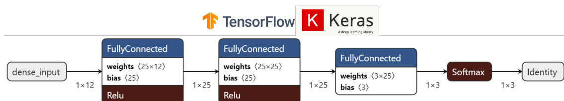
Figure 8. Neural Network with two hidden neural layers of 25 neurons each.
