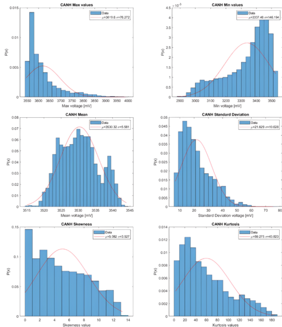
Figure 7. Estimation of Probability Density function of Unit A CANH features compared with the Normal Distribution.
