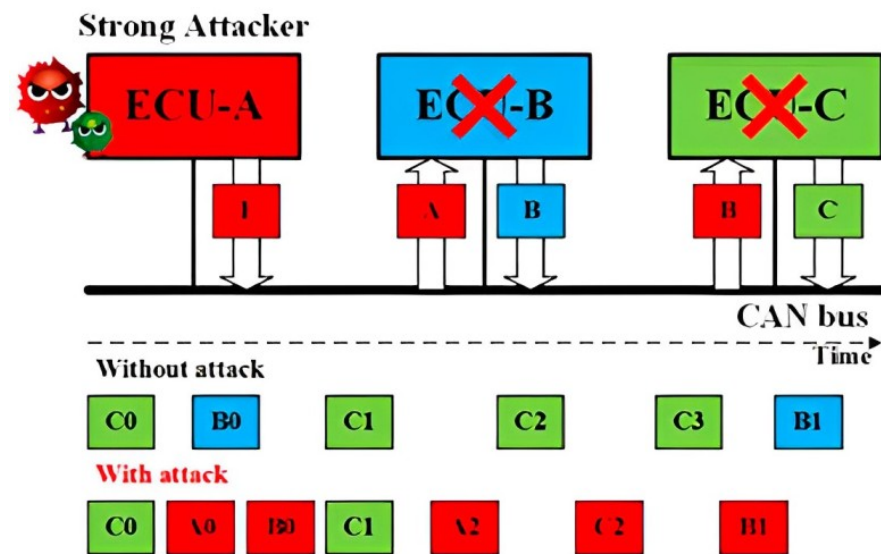
Figure 3. Schematic representation of the Injection attack concept.
