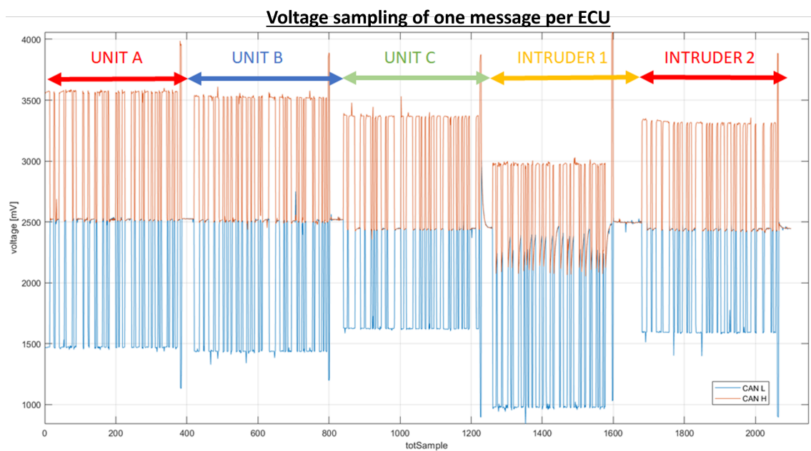
Figure 11. Voltage sampling of one message per unit.
