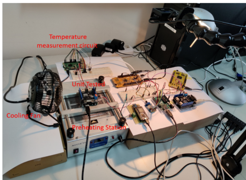
Figure 19. Final Setup for Thermal Test.
