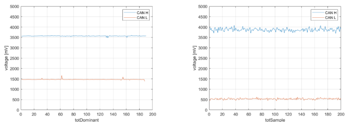
Figure 13. Example of Dominant Real Value (left) + Example of Dominant Fictitious Values (right).
