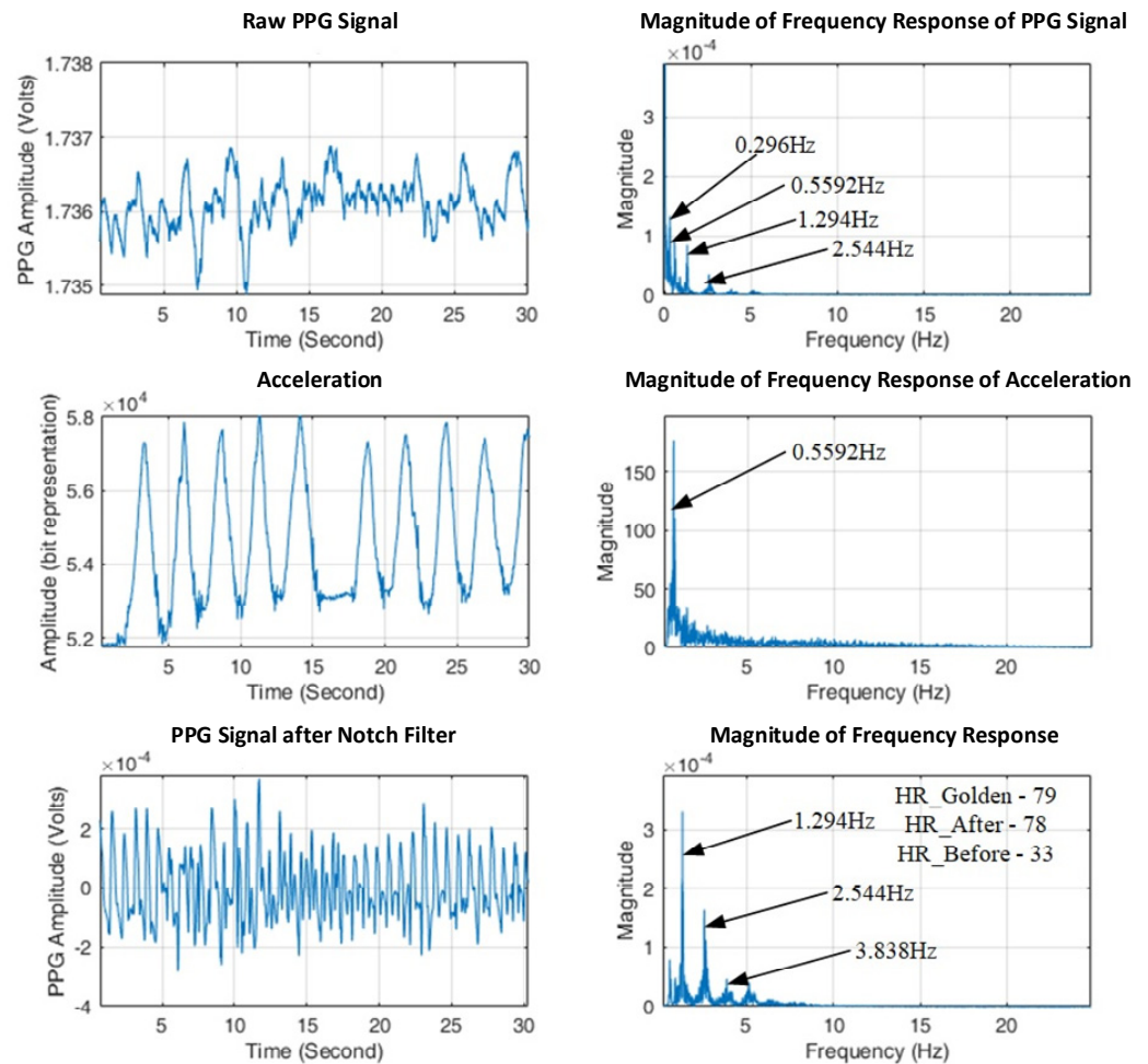
Figure 9. Estimating heart rate for hand movement using the proposed algorithms.
