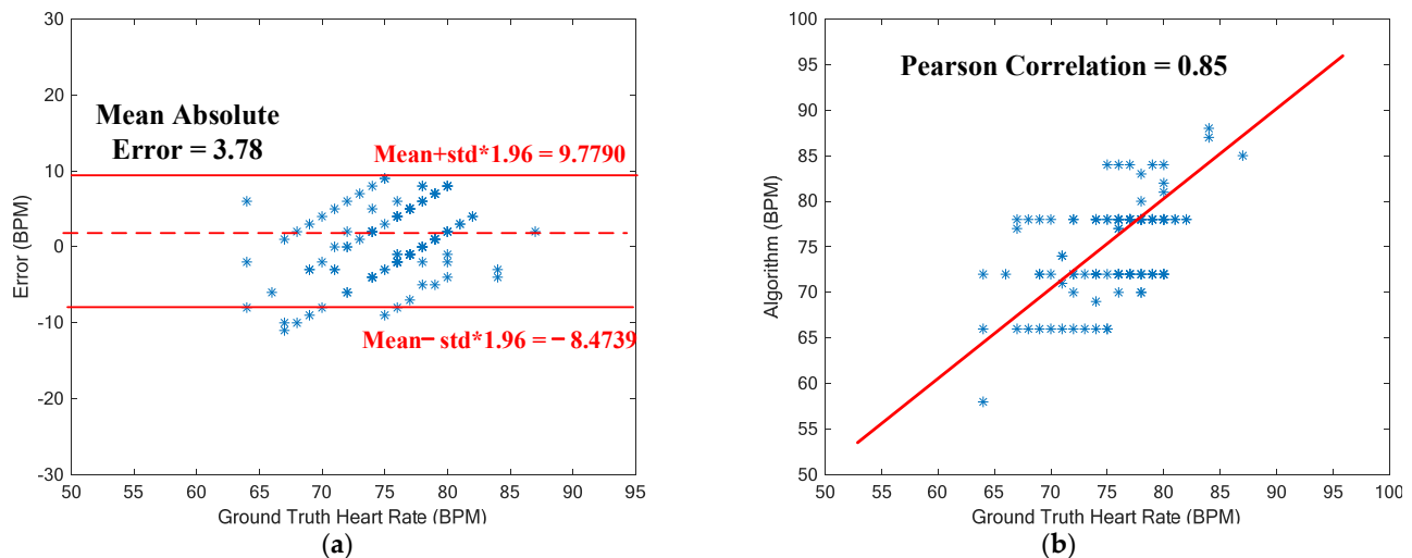
Figure 12. (a) Bland–Altman plot for heart rate estimation. (b) Correlation plot of estimated HRs vs. ground-truth HRs for the case of hand movement.
