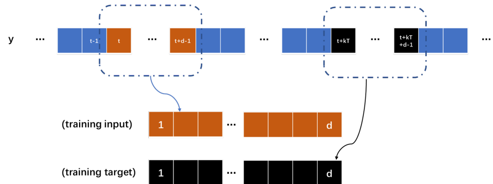
Figure 4. The period sub-sampler module in framework.
