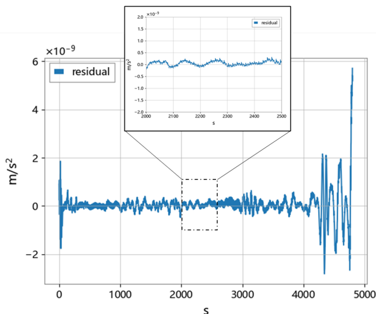
Figure 22. Residual between N2N method and Level-1B.
