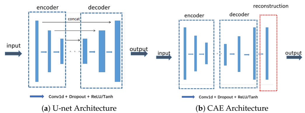
Figure 6. Network model under N2N framework for signal denoising.
