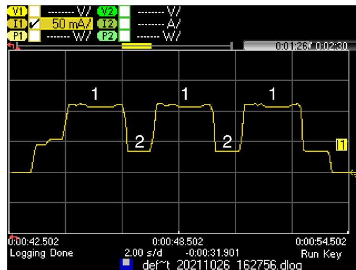
Figure 11. Current consumption profile of a LoPy4 device performing a U-Proc. In this measurement, the Sigfox UL frame payload size is 12 bytes, equivalent to a Regular (not All-0) SCHC Fragment carrying one tile.
