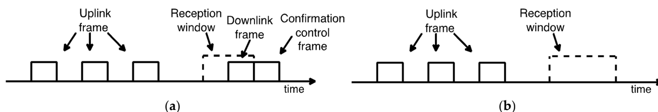
Figure 3. B-Proc examples: (a) a DL frame is received, and a confirmation control frame is sent; (b) no DL frame is received by the device.
