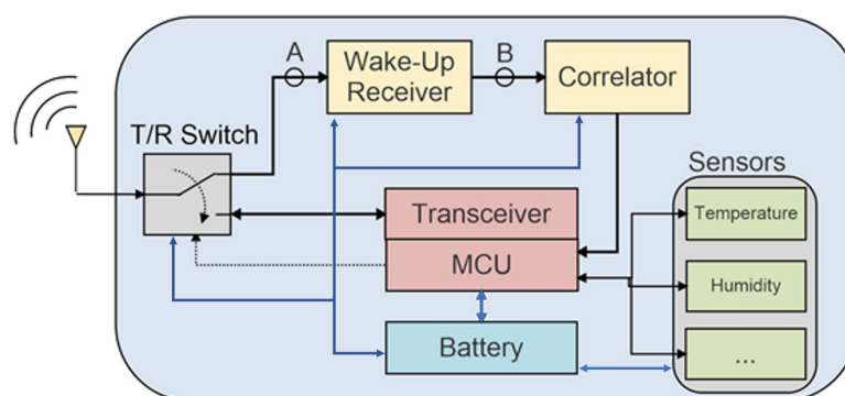
Figure 1. Block diagram of a sensor node integrating a WuR [3].
