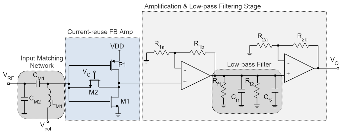
Figure 9. RFED WuR with current-reuse amplifier [8].
