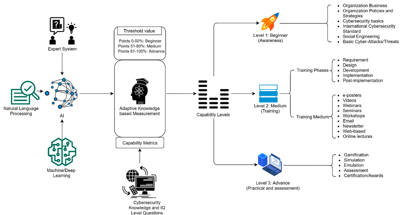
Figure 3. Entire structure of the CAT framework.
