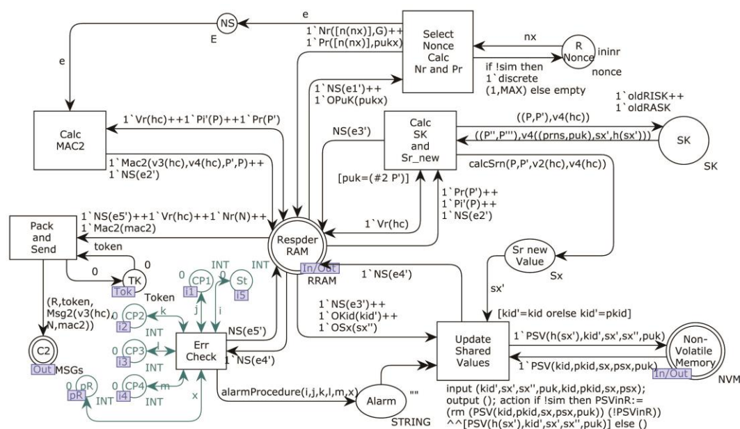
Figure 10. Responder model sub-page OP2_2.
