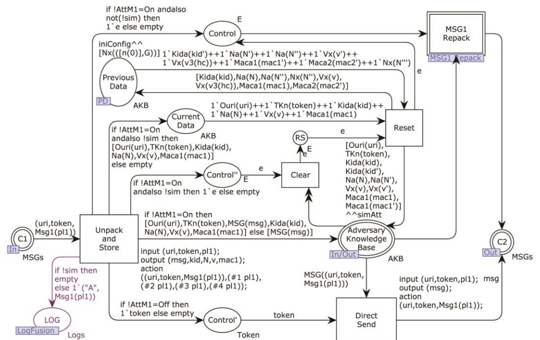
Figure 13. Adversary model sub-page MSG1_Hacking.
