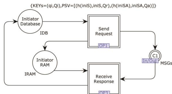
Figure 6. The second-layer model of Initiator.
