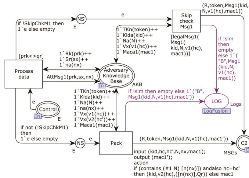
Figure 14. Adversary model sub-page MSG1_Repack.
