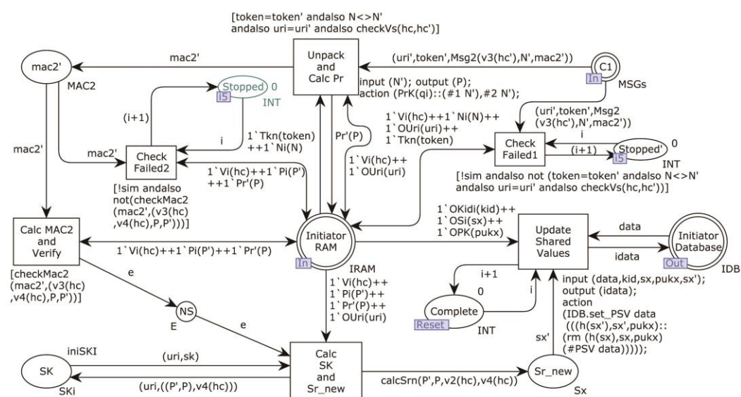
Figure 11. Initiator model sub-page OP 3.
