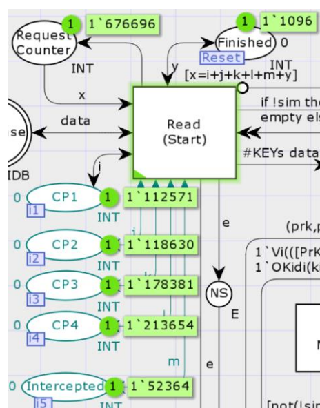
Figure 18. The simulation results in observation places.
