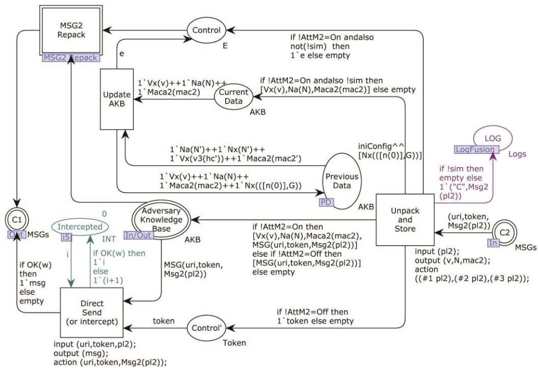
Figure 15. Adversary model sub-page MSG2_Hacking.
