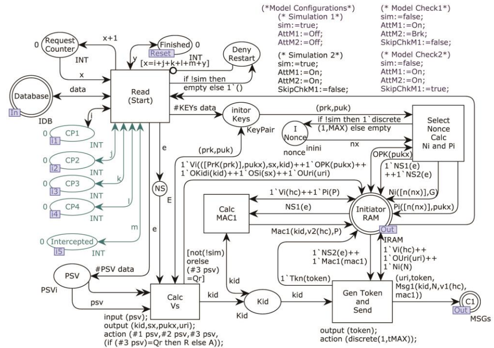
Figure 8. Initiator model sub-page OP1.
