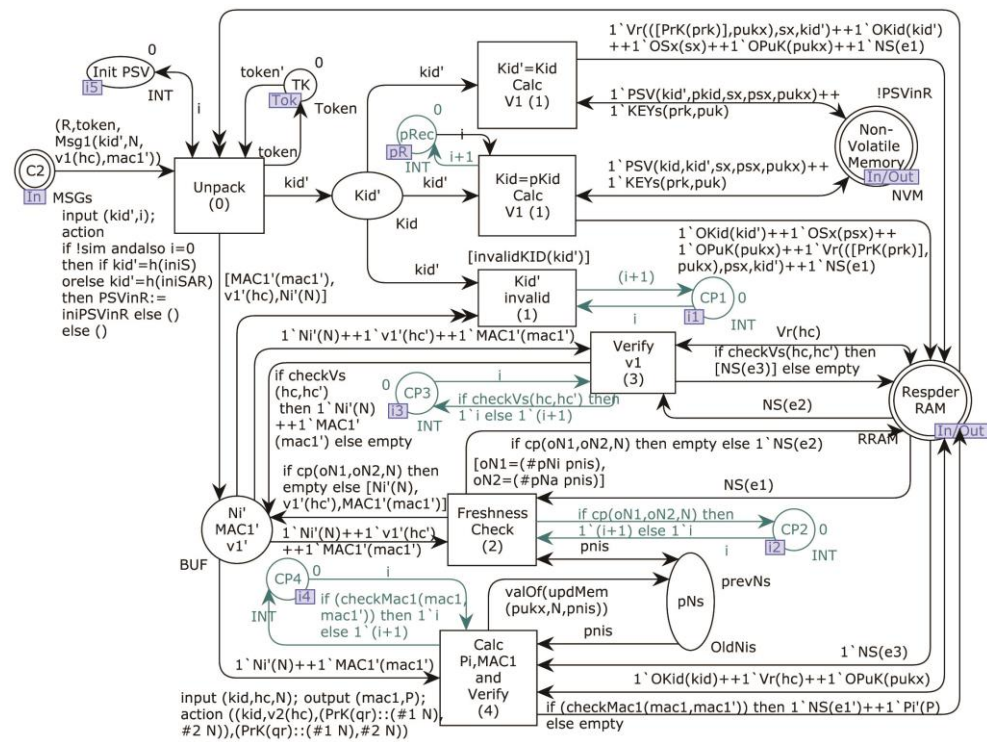
Figure 9. Responder model sub-page OP2_1.
