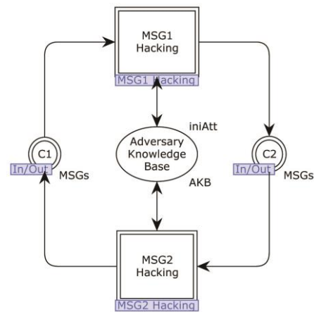
Figure 12. The second-layer page of the network (Adversary).
