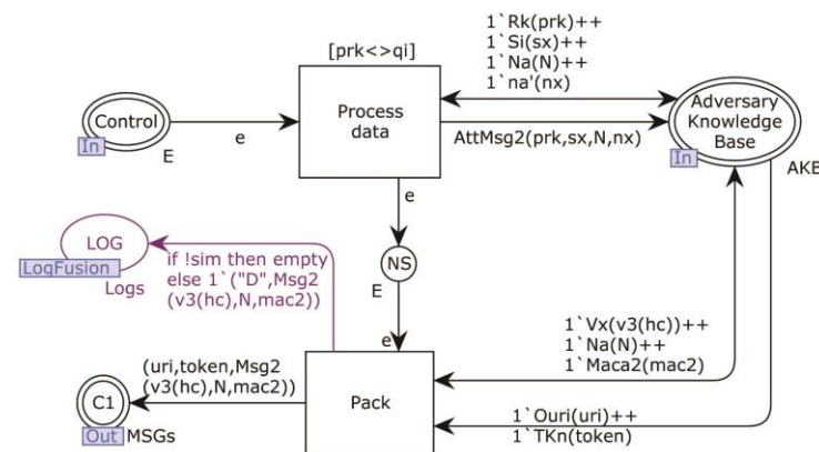
Figure 16. Adversary model sub-page MSG2_Repack.
