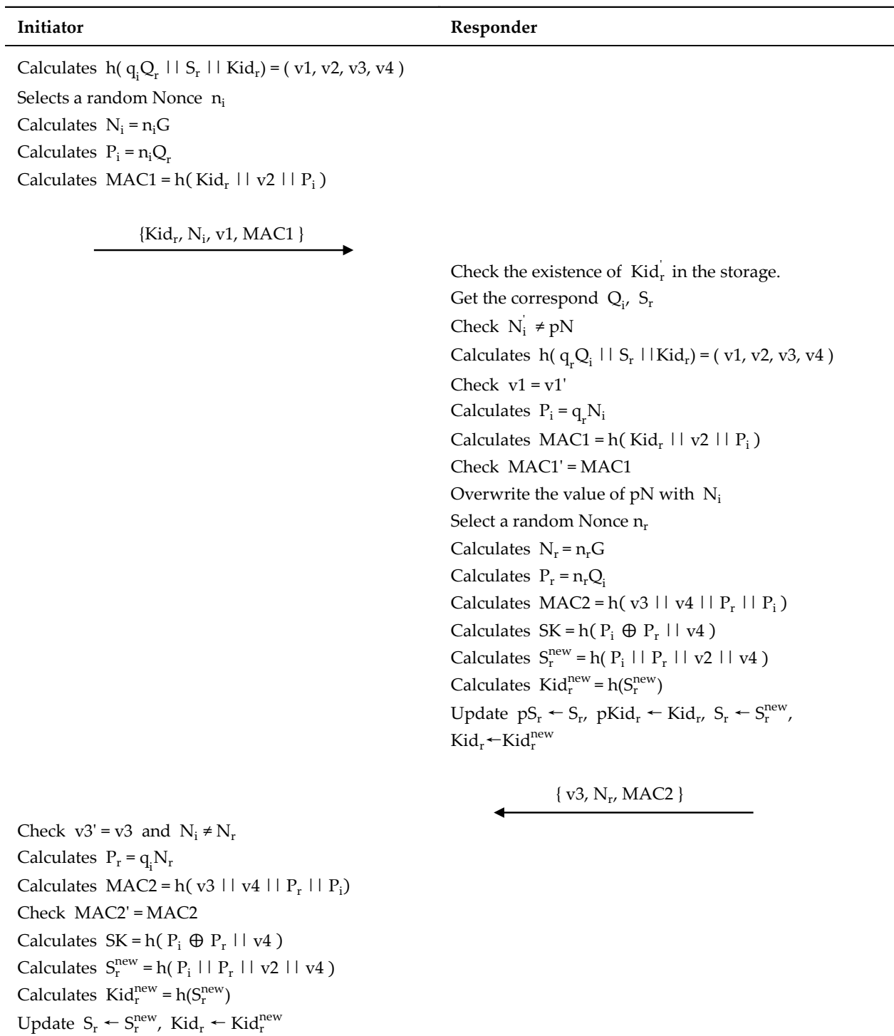
Figure 3. Identity authentication and key agreement phase.
