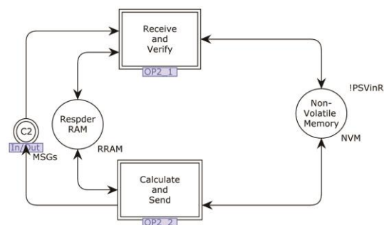
Figure 7. The second-layer model of Responder.
