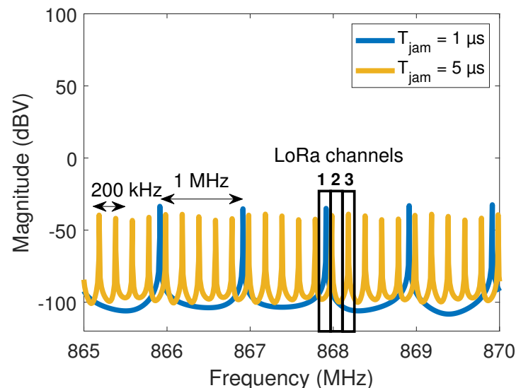
Figure 5. Jamming signal spectra ( T_{jam} = 1 \mu s , T_{jam} = 5 \mu s and amplitude equal to 250 mV) seen through a 1.024 ms window of a LoRa demodulator ( SF = 7 ). The spectrum spans from 840 MHz to 980 MHz, but in this figure, we only show the range from 865 MHz to 870 MHz.
