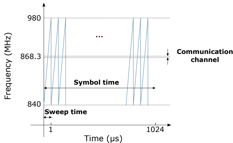
Figure 4. Time–frequency representation of a 1 \mu s jamming signal. This graph shows that, during T_{sym} = 1.024 \text{ ms} , a SF = 7 LoRa receiver is subject to 1024 jamming signal cycles.
