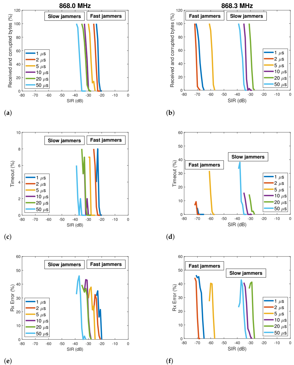
Figure 8. Three different indicators related to the reliability of a LoRa communication link ( SF = 7 , CR = 4/5 , B = 125 \text{ kHz} ) under jamming attack. Six different jamming signals were generated, each of them with a particular sweep period. LoRa transmission frequency: 868.0 MHz (a,c,e) and 868.3 MHz (b,d,f).
