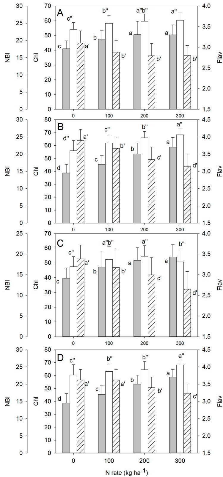
Figure S1. Average values (±SD) of the NBI (grey bars), Chl (white bars) and Flav (striped bars) Duallex indices as function of the N rates (n=90) indices in 2018: July (A) at 39 DAT, October (B) at 136 DAT and 2019: July (C) at 49 DAT, October (D) at 126 DAT. For each index, means followed by the same letter do not differ significantly at p=0.05 according to the Holm-SidakTukey test.
