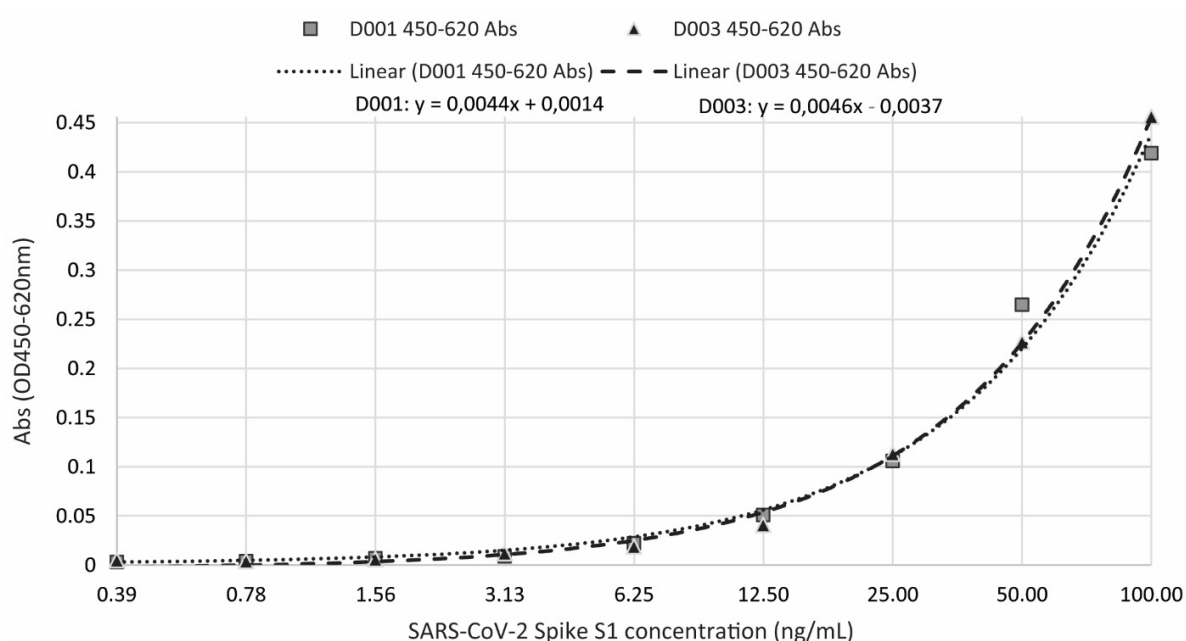
Figure S1 ELISA for validating the binding of anti-SARS-CoV-2 Spike S1 antibodies (#45150-D003 and #45150-D001) to varying concentrations of Sars-Cov-2 Spike S1 protein (#40591-V08B1).
