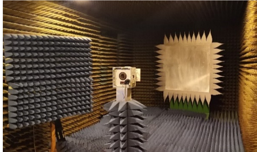
Figure 15. CATR anechoic chamber with reflector and serrations, Rx antenna on rotating mast and Tx antenna (behind absorbing wall cones).
