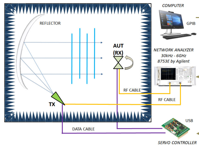
Figure 16. Layout of the anechoic chamber used for the antenna measurement, including interconnection details.
