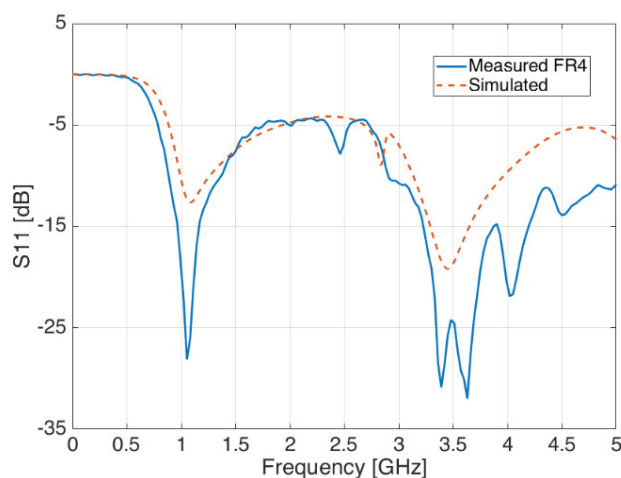
Figure 25. Reflection coefficient S_{11} of simulated antennas (red dashed line) and measured (blue continuous line) in FR-4 material.
