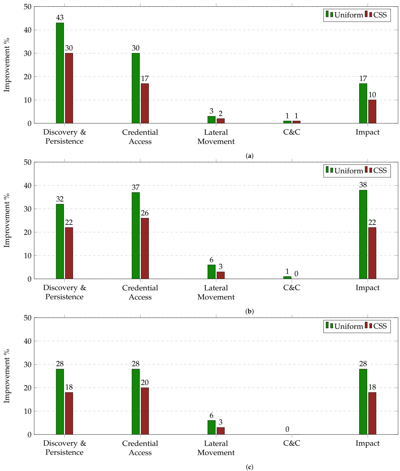
Figure 5. Average improvement of IRP on Uniform and CSS per TTP Tactic on N=8000 simulated incidents. (a) Percentage of IRP improvement per TTP category for Strategic Attacker, (b) Percentage of IRP improvement per TTP category for CSS Attacker, (c) Percentage of IRP improvement per TTP category for Uniform Attacker.
