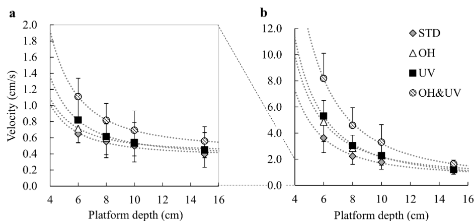
Figure 6. Translational velocity of the (a) center of mass and (b) center of pressure. Dotted lines show the approximate curves for the negative square of the platform depth ( y = a/d^2 + b ). For coefficients of the fitting functions and the significance test of the regression model, see Appendix A.
