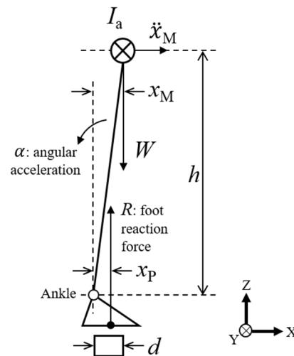
Figure 1. The inverted pendulum model of the human body on a restricted platform in the sagittal plane.
