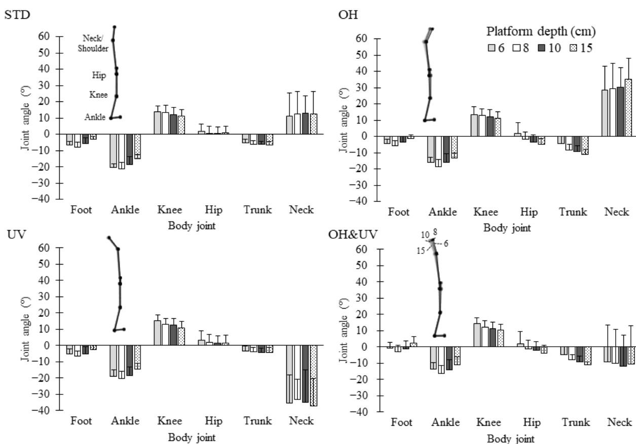
Figure 7. Body joint angle for the trunk and lower limbs and the stick diagram in the sagittal plane. For clarity, the upper limbs are not shown.
