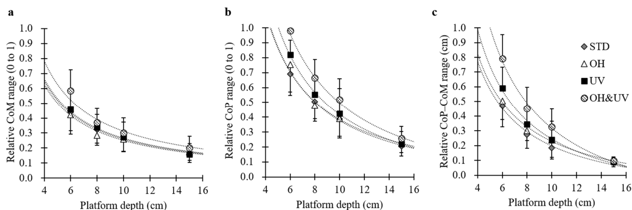
Figure 5. Relative ranges against the platform depth: (a) center of mass (CoM), (b) center of pressure (CoP), and (c) CoP–CoM displacement. Dotted lines show the approximate curves for the reciprocal of the platform depth ( y = a/d + b ). For coefficients of the fitting functions and the significance test of the regression model, see Appendix A.
