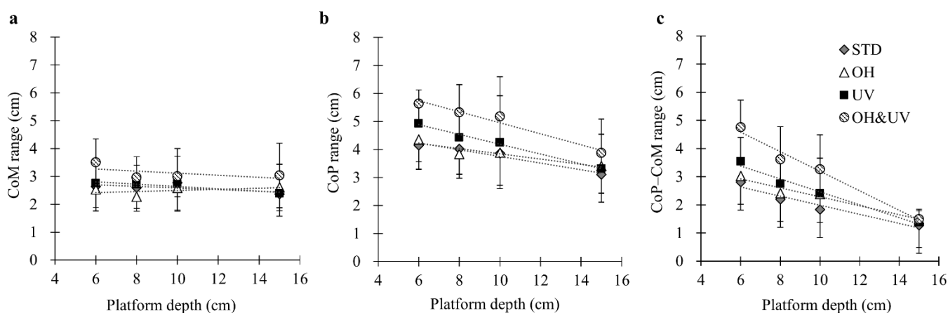
Figure 4. Absolute maximum ranges in the sagittal plane: (a) center of mass (CoM), (b) center of pressure (CoP), and (c) CoP–CoM displacement. Dotted lines show the linear approximate curves for the platform depth ( y = a \times d + b ). For coefficients of the fitting functions and the significance test of the regression model, see Appendix A.
