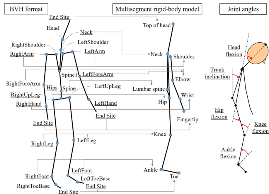
Figure 3. The model of the BVH format and the nodes used for calculating the joint positions and the definitions of the joint angles. The underlined nodes in the BVH model are adopted as the body joints in the multisegment rigid-body model.
