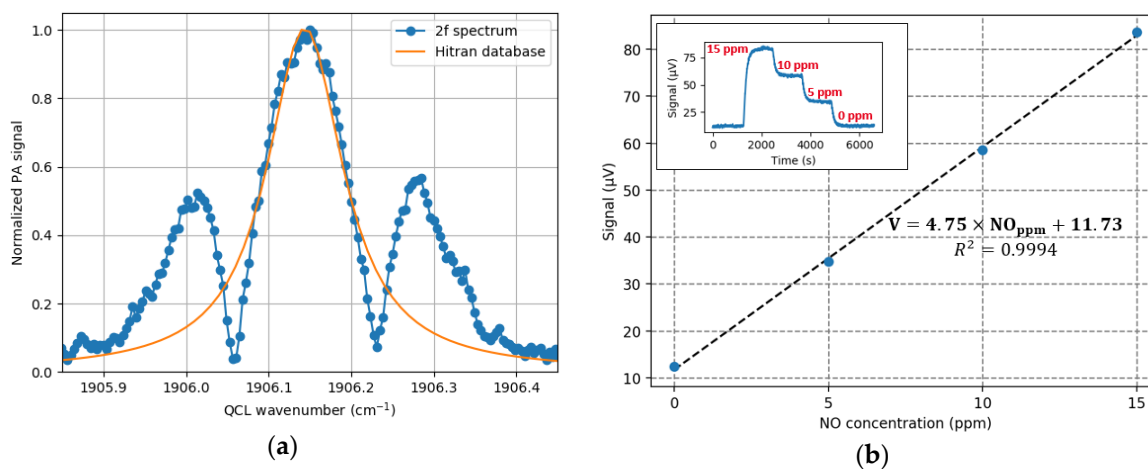
Figure 15. (a) 2f scan of the NO absorption line (blue) compared with the Hitran database (orange); (b) Calibration of the PA sensor for a measurement of 6600 s.
