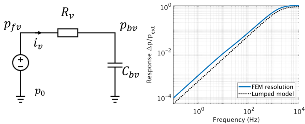
Figure 7. On the left, equivalent electrical circuit responsible for the pressure differential across the slit, given an applied pressure p_{\text{ext}} . On the right, transfer function of the circuit and comparison with the FEM simulation using the FLNS model.
