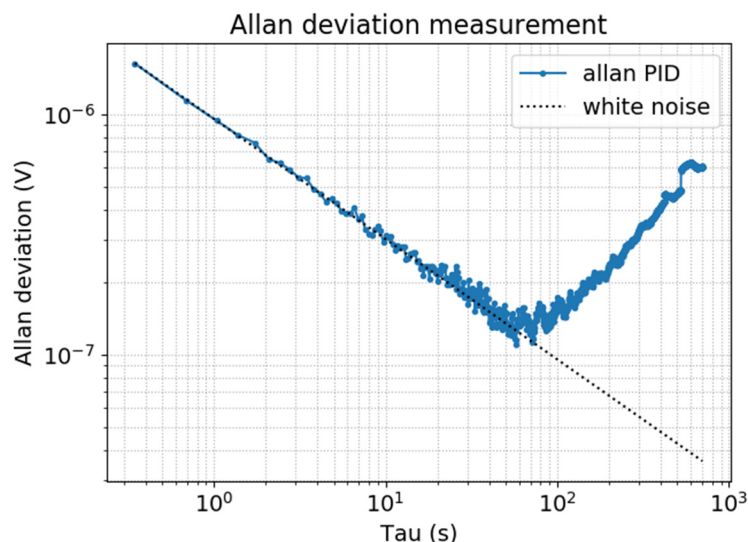
Figure 16. Allan deviation of the PA sensor in presence of a 5 ppm of NO in \text{N}_2 (blue curve) and theoretical white noise curve in 1/\sqrt{t} (dotted black).
