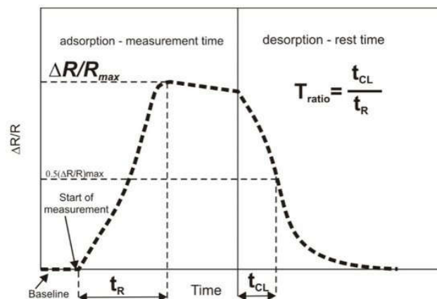
Figure S3. Scheme of a typical sensorgram with three-parameters for metal oxide semiconductor (MOS).
