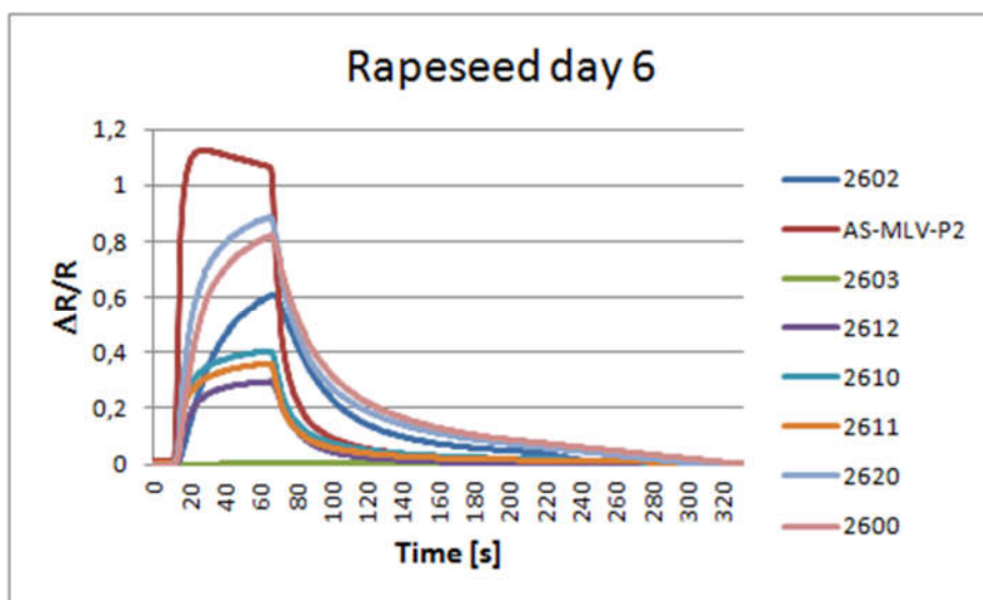
Figure S4. Typical response graph for metal oxide semiconductor (MOS).
