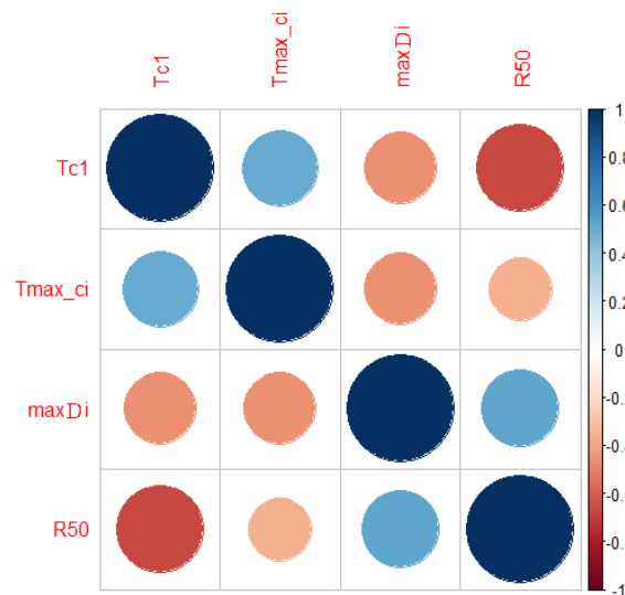
Figure 3. Correlation plot between the four features.
