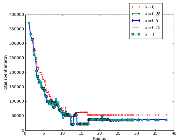
Figure 13. Impact of the cluster-head selection policy.
