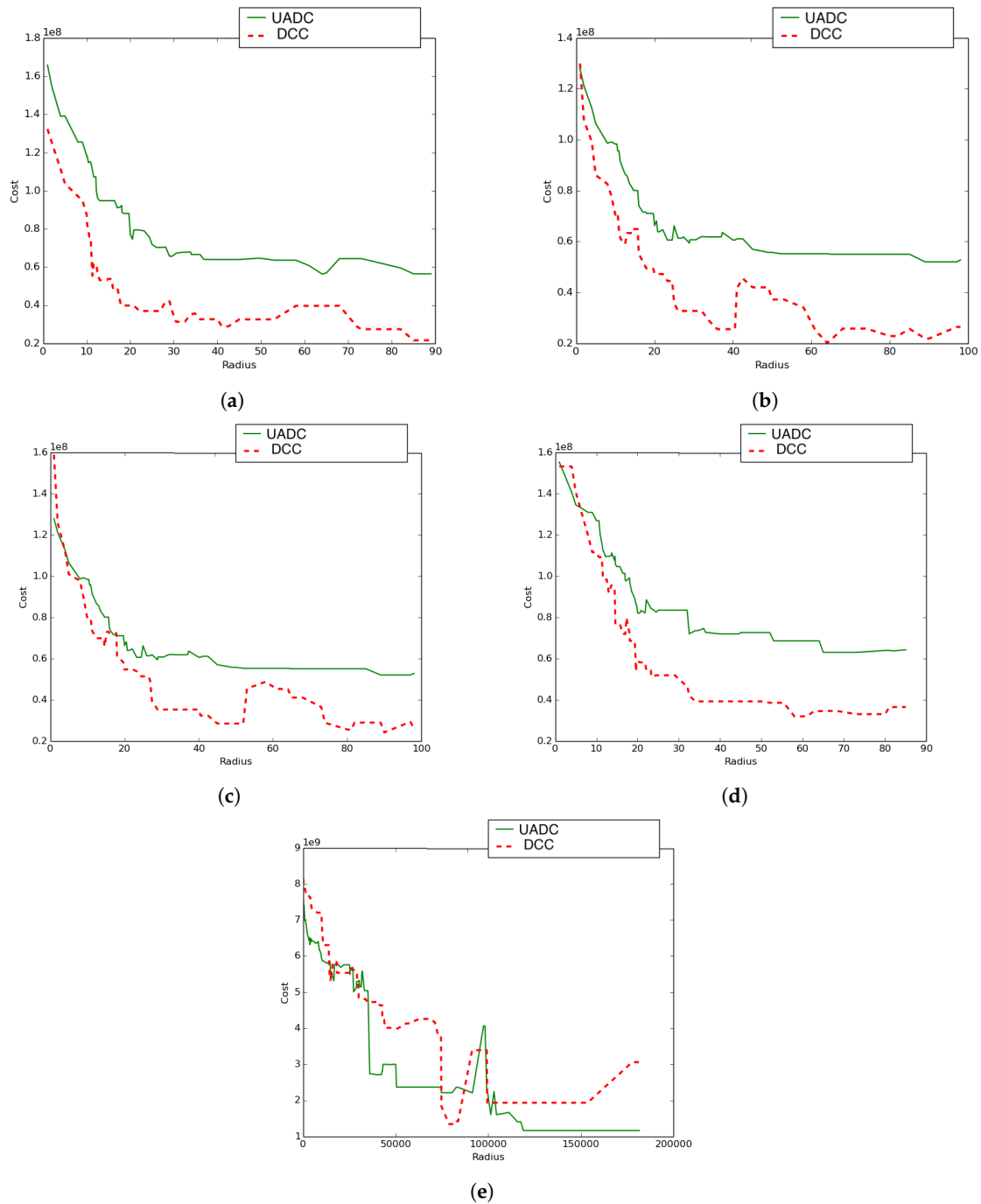
Figure 14. Algorithms comparison on different topologies. (a) Case 1; (b) Case 2; (c) Case 3; (d) Case 4; (e) Case 5. UADC, UAV-Aware DCC.
