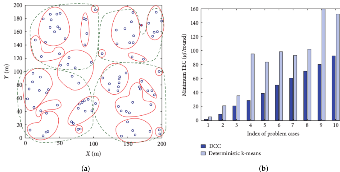
Figure 1. Comparison between Distance-based Crowdedness Clustering (DCC) and deterministic k-means [7]. (a) Clustered nodes; (b) minimum energy per round. TEC, Total Energy Consumption.
