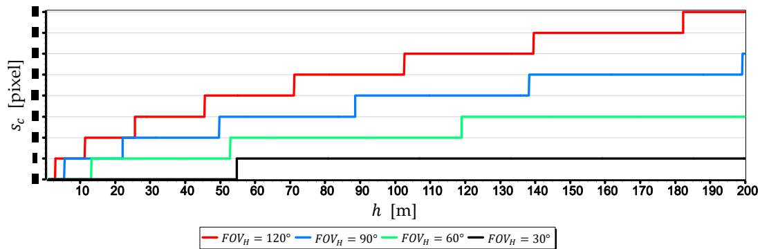
Figure 6. Horizon sagitta s_c as a function of the height of the camera a.s.l. h (for FOV_H equals 30°, 60°, 90° and 120°, R = 6378000.0 m, k = 0.16 , p_H = 4000 pixels).
