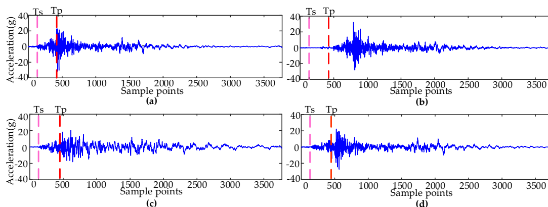
Figure 3. Measured vibration signals and the time domain segmentation unit: (a) The normal condition; (b) The iron core stagnation; (c) The screw loosening condition; (d) The poor lubrication condition.
