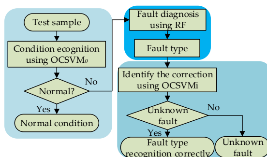
Figure 1. Diagnosis process of the hybrid classifier.
