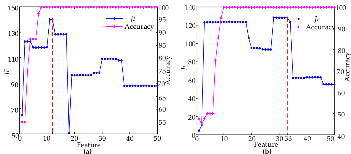
Figure 8. J_F and classification accuracy of different feature sets: (a) 29 segments of time domain segmentation; (b) nine segments of time domain segmentation.
