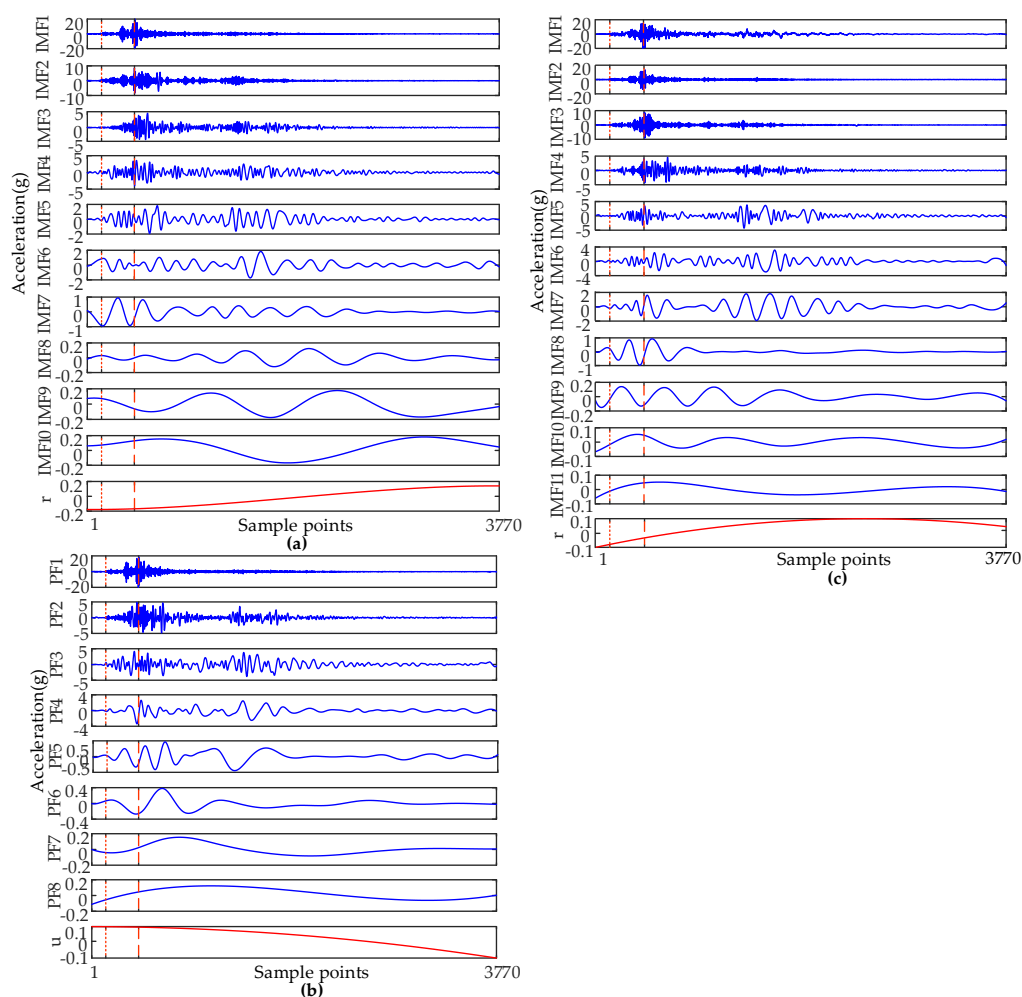
Figure 4. The time domain segmentation of EMD, LMD, and EEMD: (a) IMFs decomposed by EMD method; (b) PFs decomposed by the LMD method; (c) IMFs decomposed by the EEMD method.
