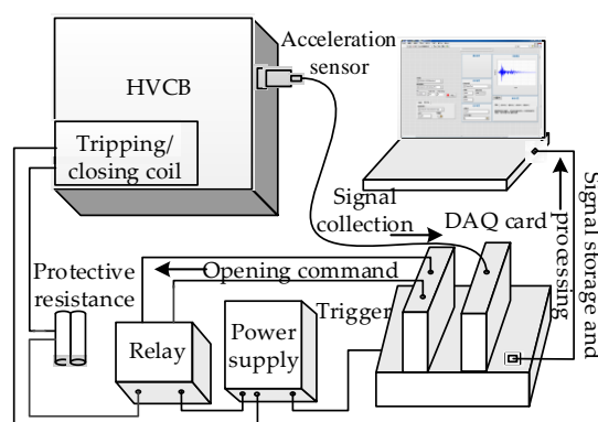
Figure 2. Vibration signal acquisition system.
