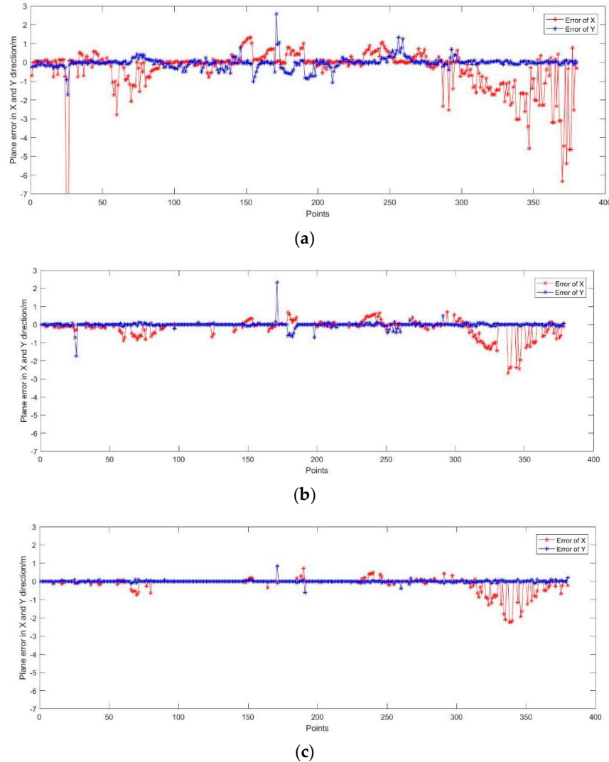
Figure 14. Plane error calculated based on three filtering algorithm. (a) Plane error calculated based on least square algorithm; (b) Plane error calculated based on Extended Kalman Filter (EKF) algorithm; (c) Plane error calculated based on Robust-EKF algorithm.
