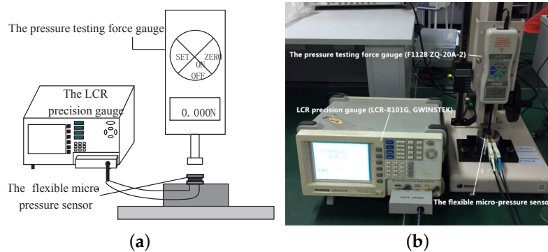
Figure 8. The sensor was tested by a pressure simulation experiment system. (a) The diagram of the experiment setup. (b) The photograph of the experiment setup.
