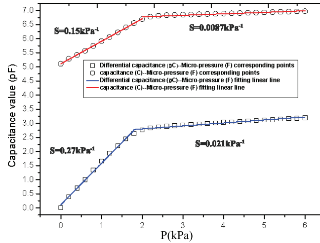
Figure 9. The static characteristic of the sensor without sensitivity compensation and with sensitivity compensation structure.
