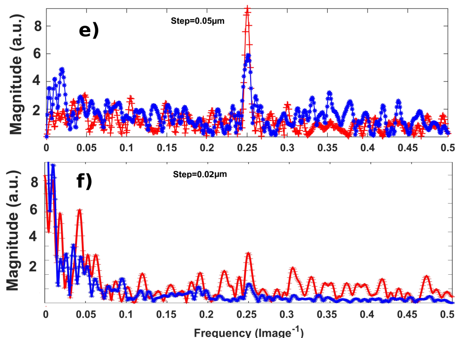
Figure 9. Results of resolution test along X (red) and Y (blue) directions at a median distance z = 151 mm. Steps of (a) 0.15\ \mu\text{m} ; (b) 0.10\ \mu\text{m} ; (c) 0.05\ \mu\text{m} , (d) 0.02\ \mu\text{m} ; (e,f) power spectrum of the data series with steps of (e) 0.05\ \mu\text{m} and (f) 0.02\ \mu\text{m} . The frequency of the input command applied is of 0.25\ \text{frame}^{-1} .
