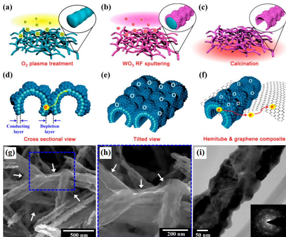
Figure 1. (a–e) Schematic illustration of formation of 3D graphene-WO 3 hemitube architectures; (g–i) SEM and TEM image with SAED pattern in the inset of graphene-WO 3 hemitube composite. Reproduced with permission from [57], © 2012 American Chemical Society
