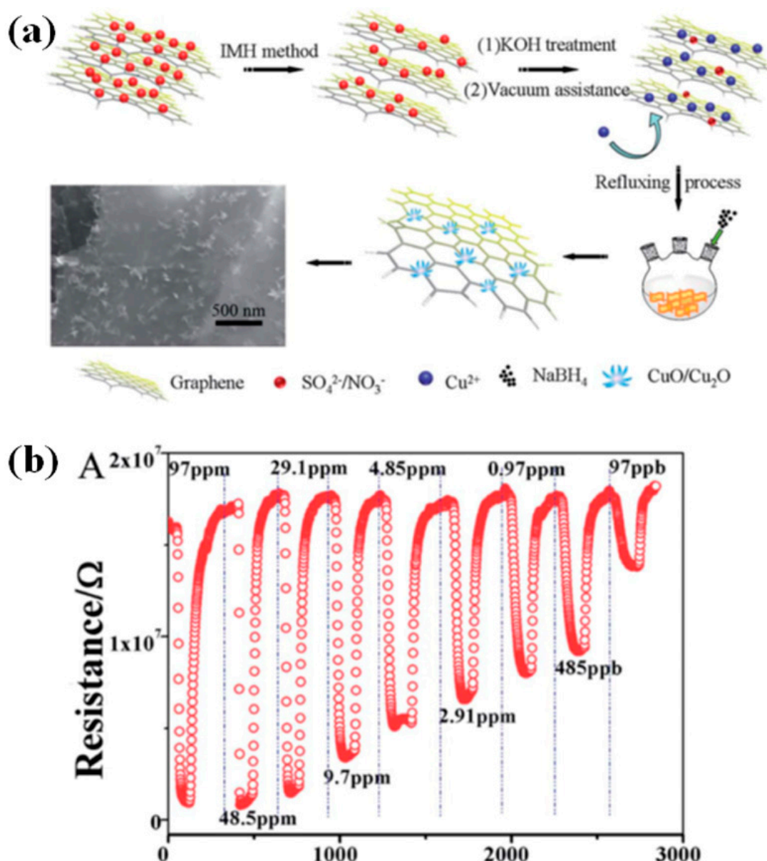
Figure 10. (a) Schematic illustration of formation of 3D nanoflower-like Cu x O/multilayer graphene; (b) Dynamic sensing property of CuMGC at room temperature. Reproduced with permission from [92] © 2014 Royal Society of Chemistry.
