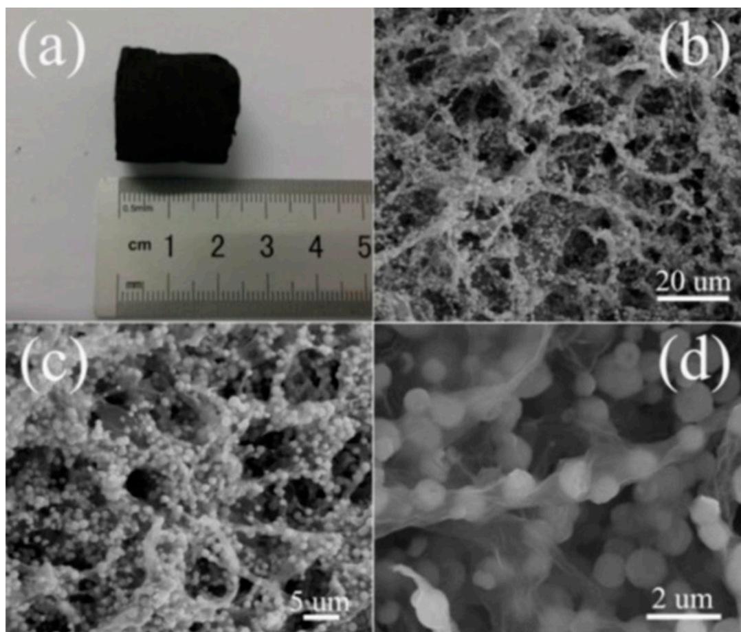
Figure 9. Morphology of 3D rGO aerogel/ZnO spheres composite. (a) A photograph of composite. (b–d) SEM images with different magnifications of rGO aerogel/ZnO spheres composite. Reproduced with permission from [43], © 2015 Elsevier.
