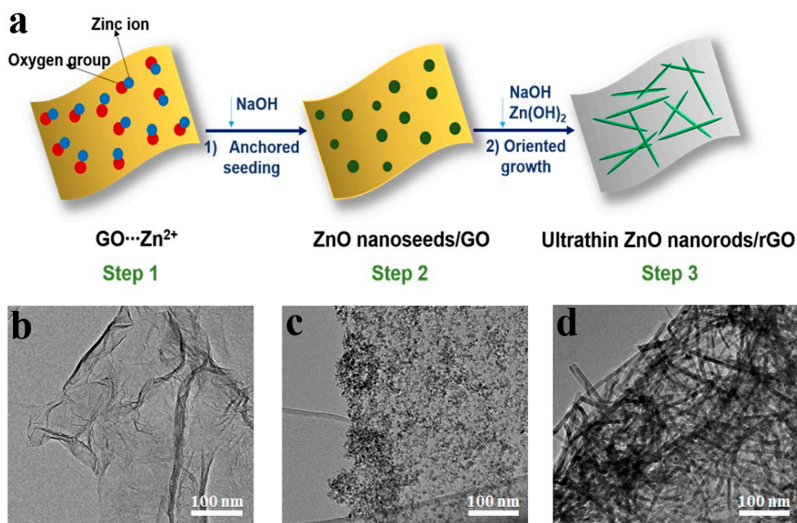
Figure 4. (a) Schematic illustration of fabrication of rGO/UT-ZNR; (b–d) TEM images of GO, GO/ZnO nanoseeds and rGO/UT-ZNR. Reproduced with permission from [65], © 2016 American Chemical Society.
