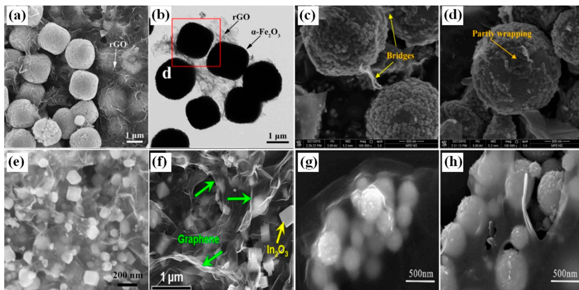
Figure 6. Morphology of (a–b) rGO/ \alpha -Fe 2 O 3 cubic nanostructure [74]; (c–d) rGO decorated TiO 2 microspheres [78]; (e) N-rGO/NiO cube [75]; (f) rGO/In 2 O 3 cube nanocomposites [76]; (g–h) graphene-wrapped WO 3 nanospheres [79]. (a–b), (c–d) and (g–h) were reproduced with permission from [74,78,79], © Elsevier. (e) and (f) were reproduced with permission from [75,76] © American Chemical Society.
