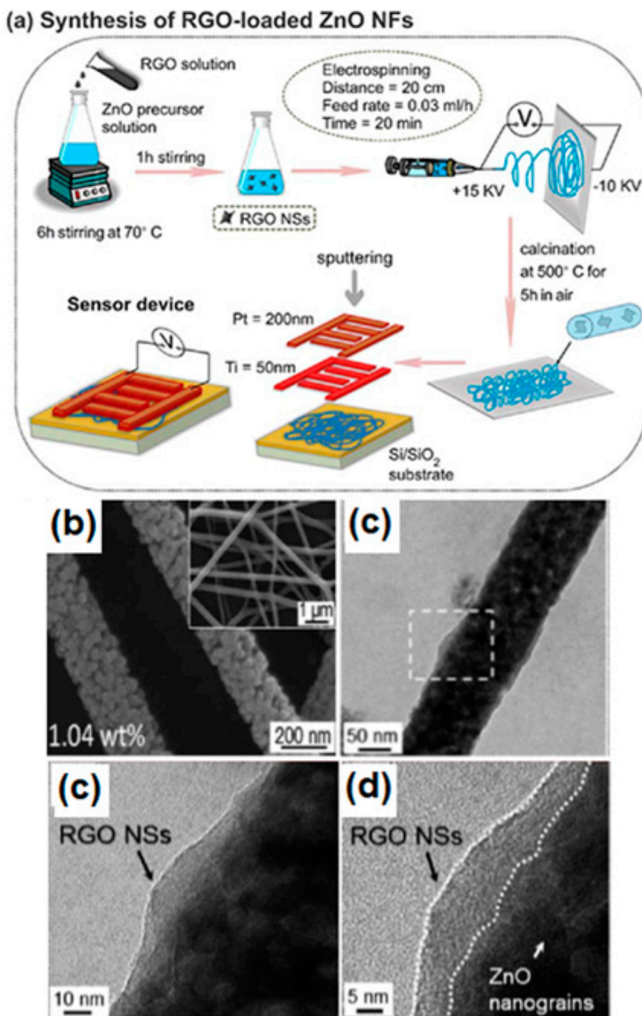
Figure 3. (a) Schematic illustration of formation of rGO nanosheet-loaded ZnO core-shell nanofibers; (b–d) SEM and TEM pictures of samples. Reproduced with permission from [61], © 2015 Elsevier.
