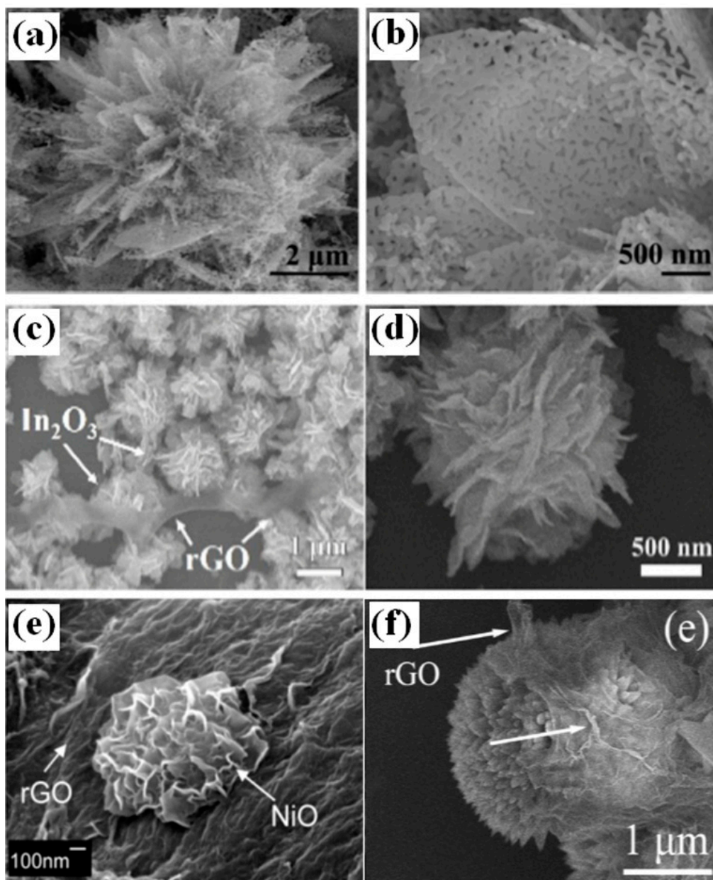
Figure 7. Morphology of (a–b) 3D hierarchical porous ZnO nanoflowers modified with rGO [83]; (c–d) 3D rGO-In 2 O 3 composite [84]; (e) rGO/NiO nanoflowers [85]; (f) urchinlike CuO 3D structures modified by rGO [86]. (a–e) were reproduced with permission from [83–85], © Elsevier. (f) were reproduced with permission from [86] © 2014 American Chemical Society.
