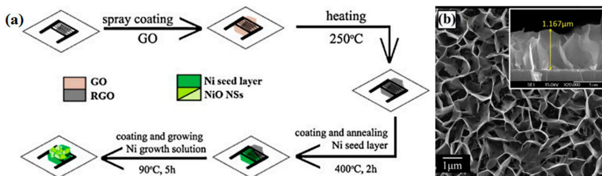
Figure 5. (a) Schematic illustration of formation of 3D porous rGO/NiO nanosheets hybrids; (b) SEM pictures of samples. Reproduced with permission from [71], © 2013 Elsevier.
