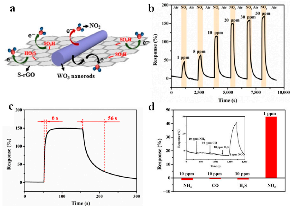
Figure 12. (a) Schematic illustration of NO 2 adsorption on S-rGO/WO 3 surface; (b,c) Dynamic response of the 3D S-rGO/WO 3 hybrids of NO 2 at room temperature.; (d) Selectivity of 3D S-rGO/WO 3 . Reproduced with permission from [106] © 2018 Springer.
