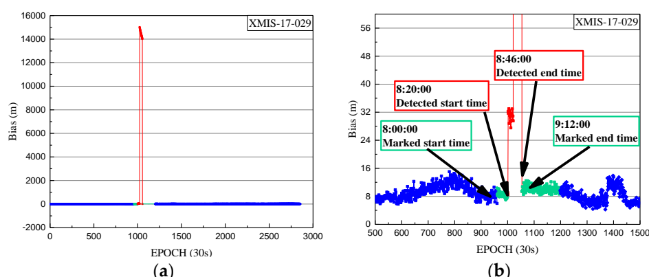
Figure 11. (a) The deviations of SPP on doy 029 of 2017 from epoch 0 to 2880. (b) The deviations of SPP on doy 029 of 2017 from epoch 500 to 1500, with a smaller range for the vertical axis. The deviations of SPP results in three-dimensional space corresponding to the healthy period in the broadcast ephemeris are indicated by the blue dots. The SPP deviations corresponding to the unhealthy period in the broadcast ephemeris with a weak anomaly detection factor of less than 0 are indicated by green dots. The SPP deviations corresponding to the unhealthy period in the broadcast ephemeris during the detected period are indicated by red dots.
