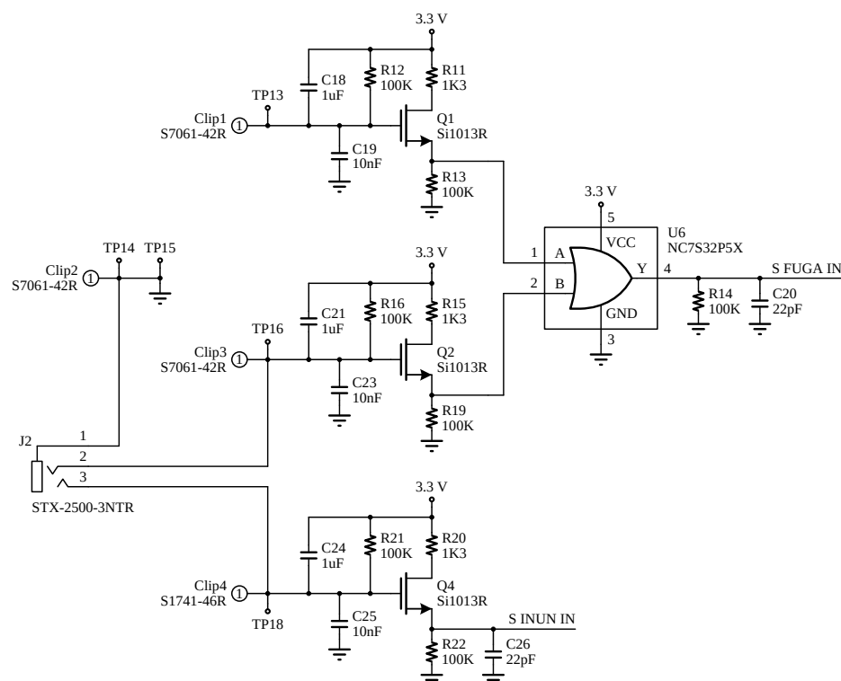
Figure 3. Simplified circuit schematic for the flood sensor.
