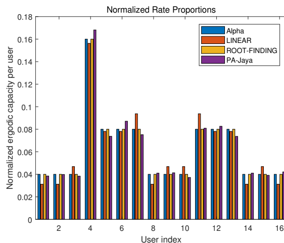
Figure 7. Comparison of different algorithm effects under normalized rate proportional constraint.
