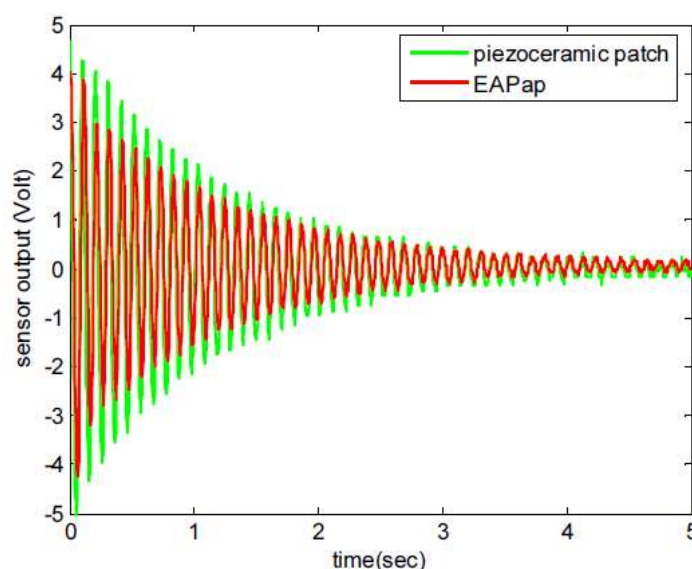
Figure 4. Impulsive response of the beam measured by EAPap and piezoceramic patch [29].
