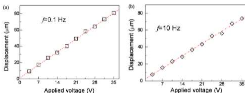
Figure 7. Plots of the bending displacement versus the applied voltage ( V_{amp} ) at the frequencies of (a) f = 0.1 \text{ Hz} and (b) f = 10 \text{ Hz} [47].
