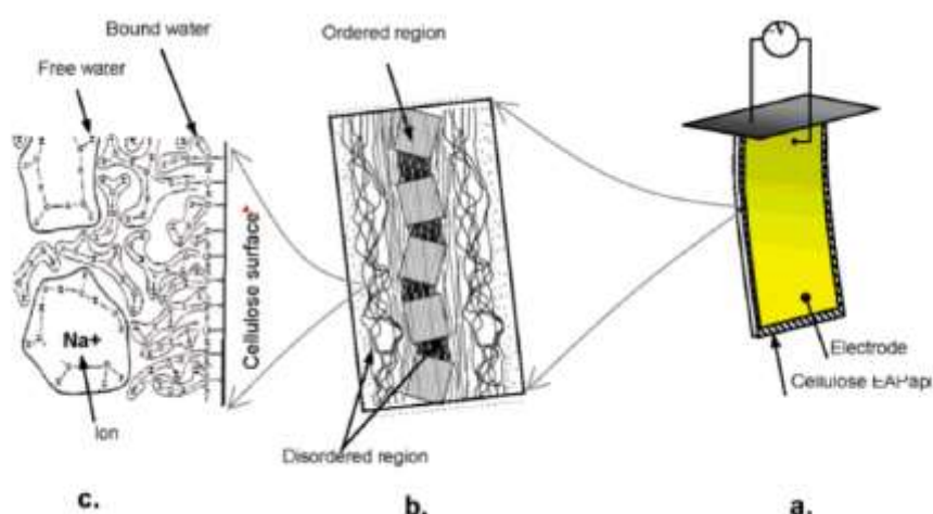
Figure 1. Concept of electro-active paper (EAPap) actuator: (a) EAPap is made from cellulose paper on which gold electrodes are deposited on both sides; (b) cellulose microfibril has ordered crystalline regions and disordered regions; (c) water molecules are bonded with hydroxyls on the cellulose surface (bound water) or clustered in free (free water) [21].
