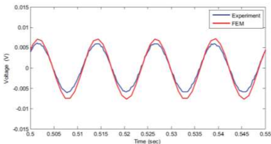
Figure 19. Voltage output produced by EH100 (energy harvester of length 100 mm) when excited by a sinusoidal force at 18 mm from the free end [82]. FEM—finite element model.
