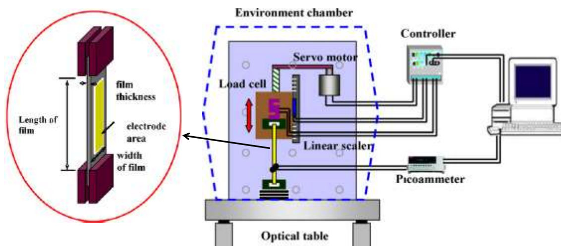
Figure 2. Schematic of piezoelectric charge constant measurement based on direct piezoelectricity [31].
