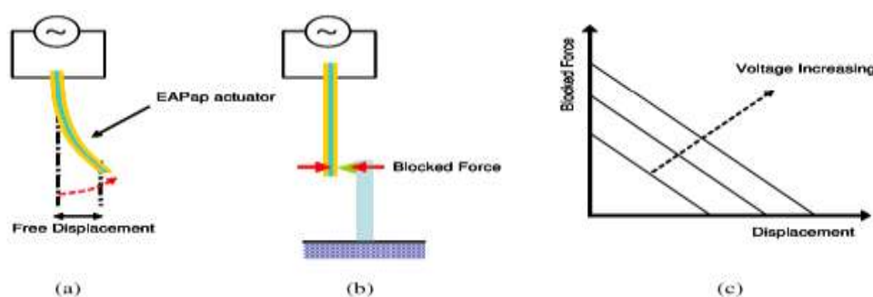
Figure 10. Schematic diagram of performance parameters: (a) free displacement, (b) blocked force, (c) force–displacement relation with increasing voltage [52].
