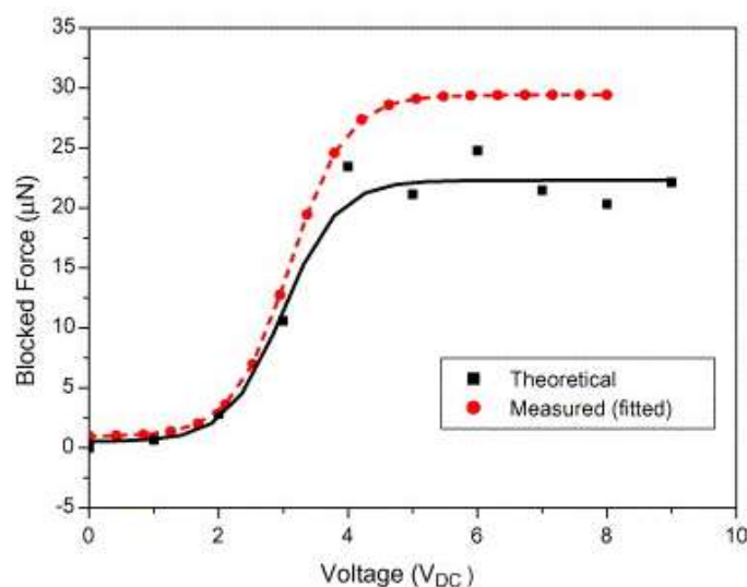
Figure 11. Comparison of measured and calculated blocked forces on DC electric field [53].
