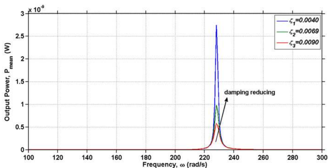
Figure 15. Mean power output of the EAPap-based energy harvester for a range of frequencies in different damping ratios [79].
