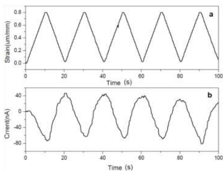
Figure 6. Stretching mode strain sensor: (a) stretching strain and (b) sensor signal [38].
