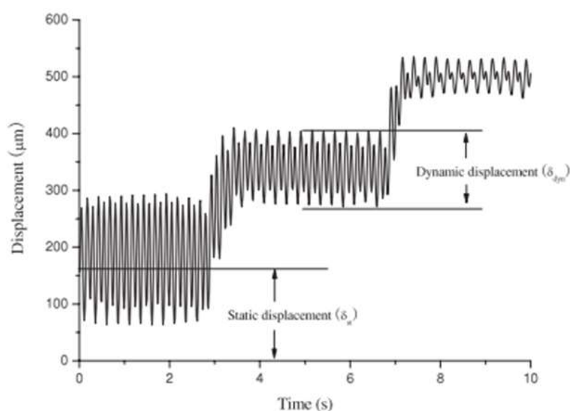
Figure 12. Static and dynamic tip deflection of the force transducer under 350 \text{V mm}^{-1} and 80% relative humidity condition [52].
