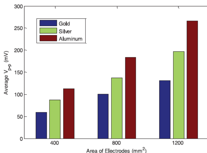
Figure 17. Average peak to peak open circuit voltage output for 400, 800, and 1200 mm 2 gold, silver, and aluminum electrode-coated EAPap [81].
