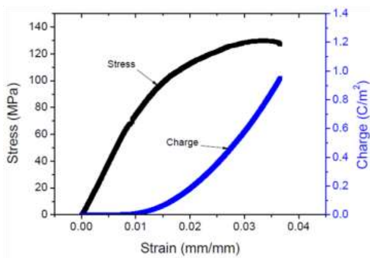
Figure 5. Stress–strain and charge curves of cellulose ZnO hybrid nanocomposite (CEZOHN) [38].
