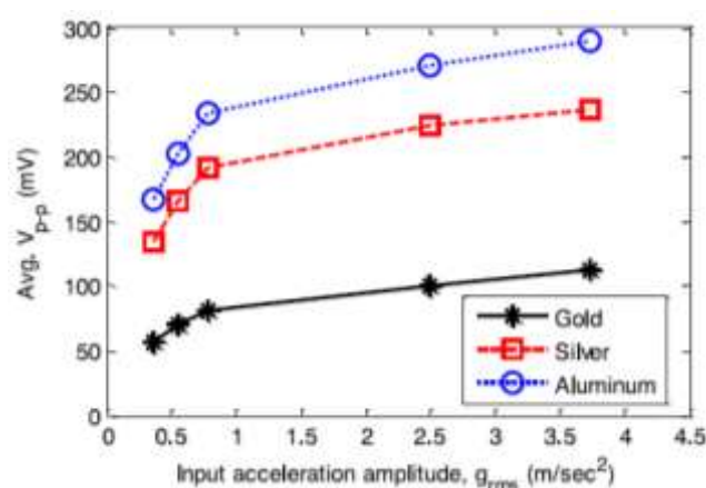
Figure 18. Variation of the average V_{pp} against the input acceleration amplitude ( g_{rms} ) for three parallel connected electrodes with an area of 1200 mm 2 [81].
