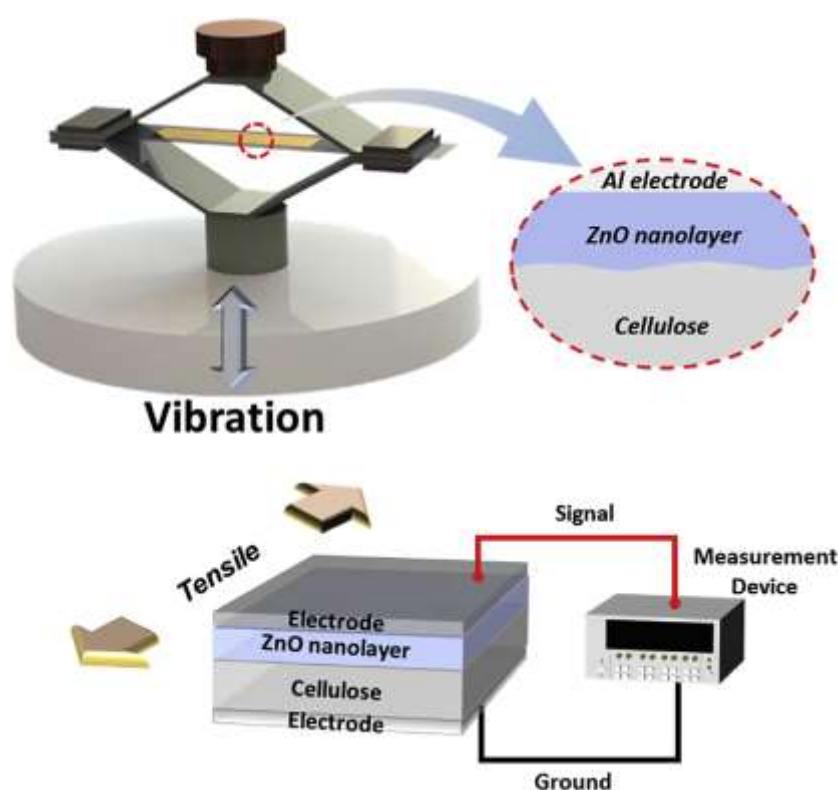
Figure 20. Cymbal type vibration energy harvester [27].
