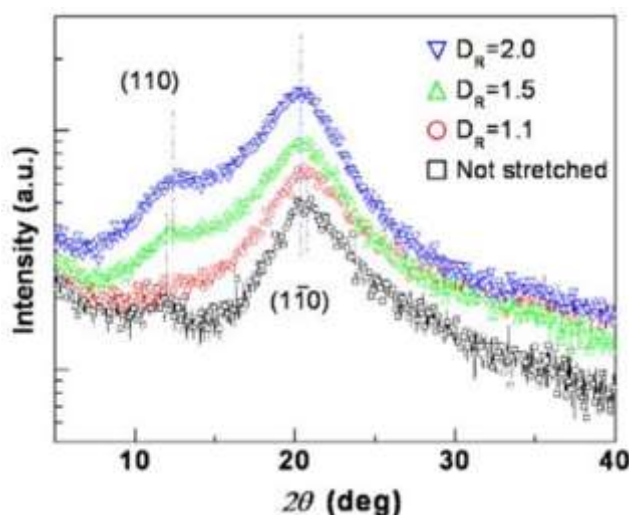
Figure 8. X-ray diffraction data of the stretched cellulose film with different stretching ratios [50].
