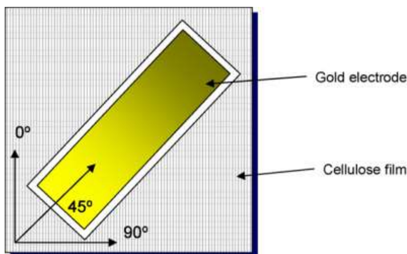
Figure 3. Orientation of cellulose film and schematic of EAPap [31].
