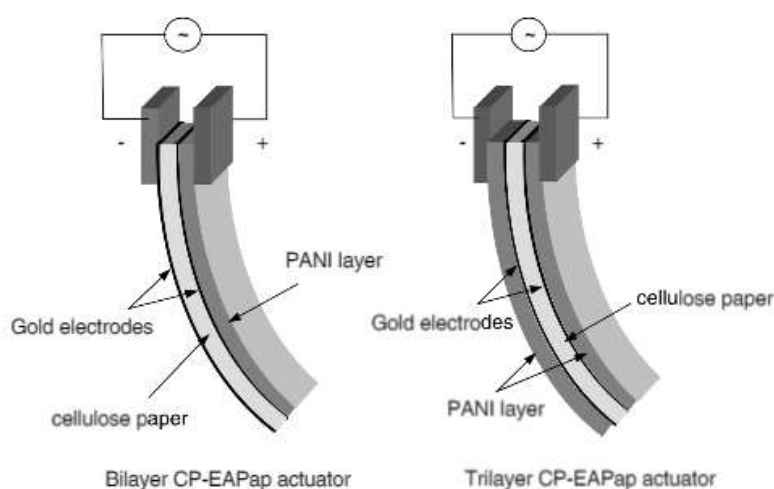
Figure 9. Schematic of bi-layer and tri-layer CP-EAPap actuators [51]. (PANI-polyaniline).
