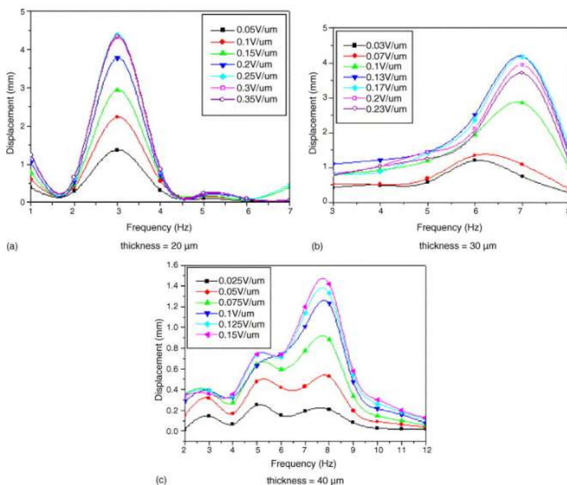
Figure 13. (a–c) Tip displacements of EAPap actuators with thickness variation [32].
