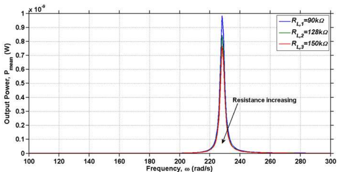
Figure 14. Mean power output of the EAPap-based energy harvester for a range of frequencies with different external resistive loads [79].
