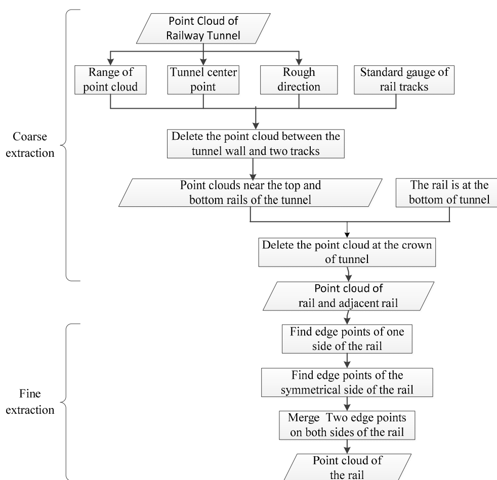
Figure 4. Flowchart of rail point cloud extraction.
