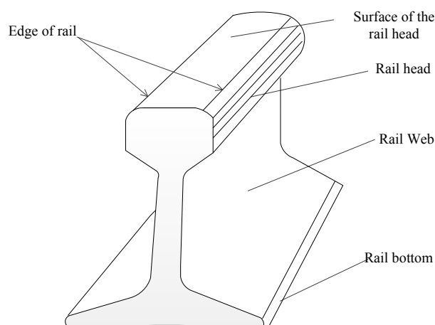
Figure 5. Rail section.
