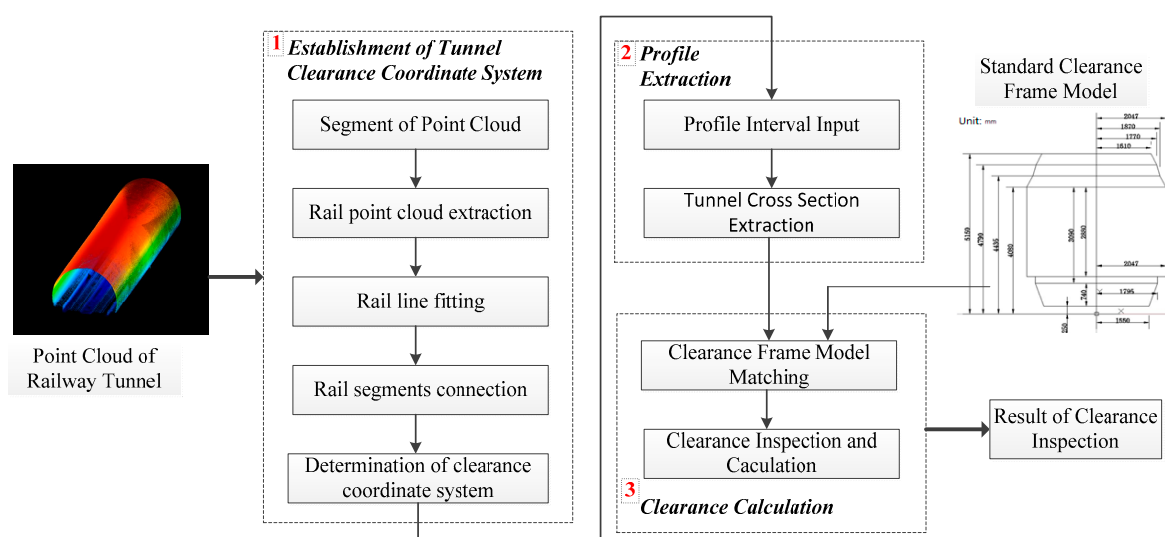
Figure 1. Technical flowchart of the proposed tunnel clearance inspection method.
