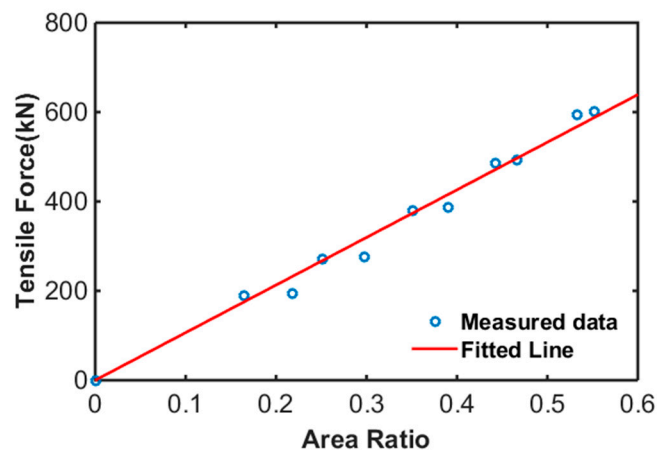
Figure 13. Relationship between area ratio and reference stress.
