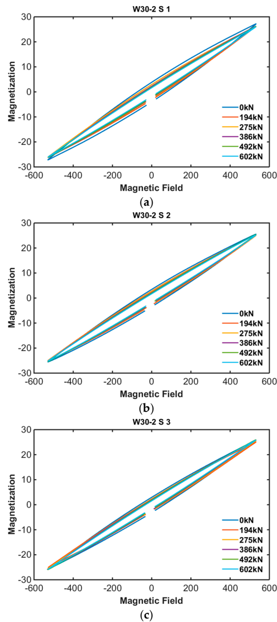
Figure 8. B-H loop of specimen 2: (a) Sensor no. 2-1; (b) Sensor no. 2-2; (c) Sensor no. 2-3.
