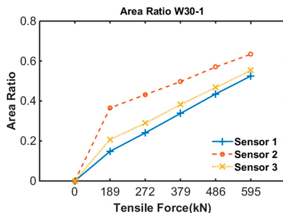
Figure 11. Area ratio of specimen 1.
