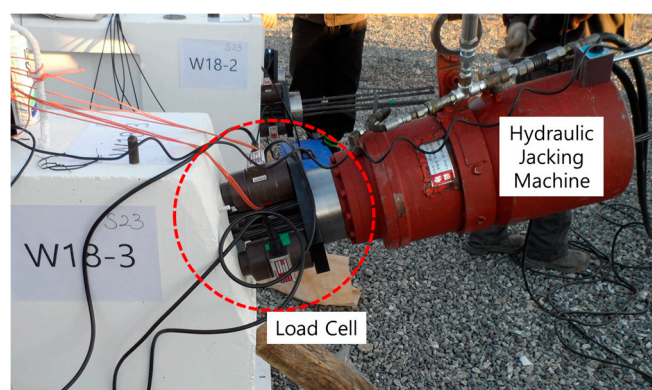
Figure 6. Installation of a load cell.
