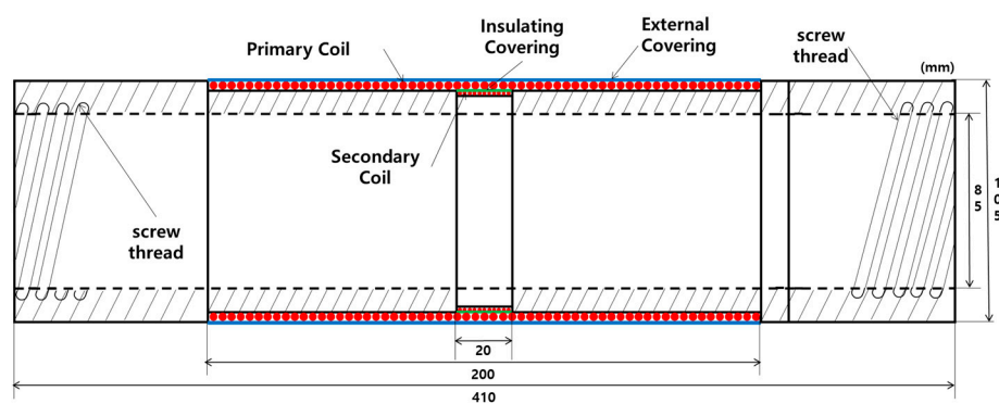
Figure 1. Schematic of the embedded EM sensor.
