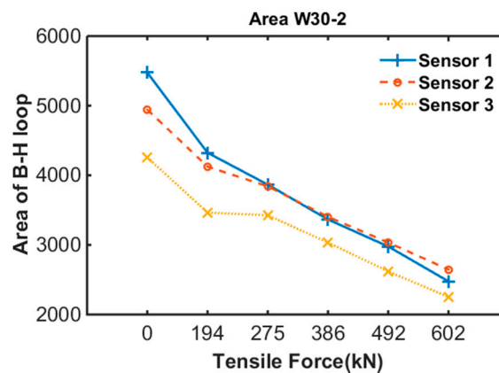
Figure 10. B-H loop of specimen 2.
