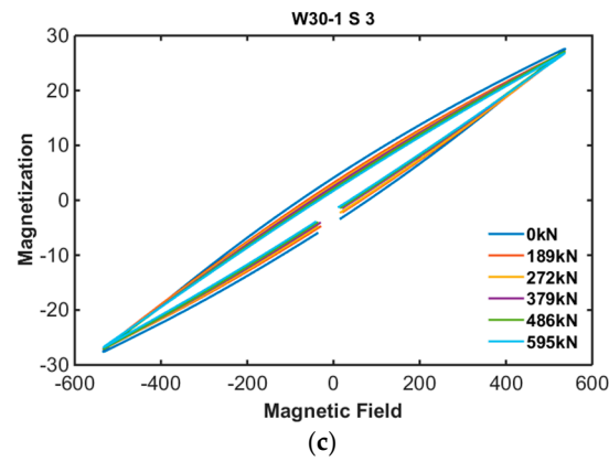
Figure 7. B-H loop of specimen 1: (a) Sensor no. 1-1; (b) Sensor no. 1-2; (c) Sensor no. 1-3.
