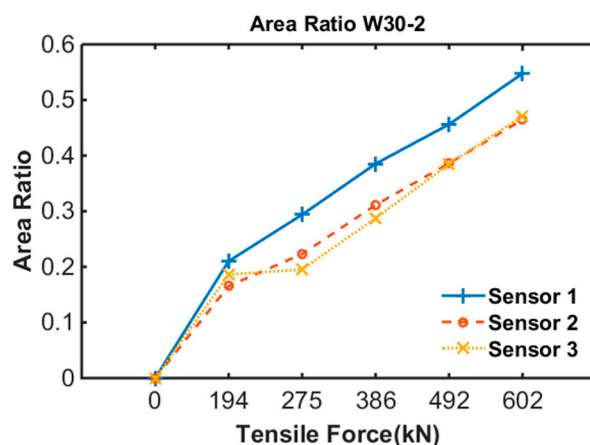
Figure 12. Area ratio of specimen 2.
