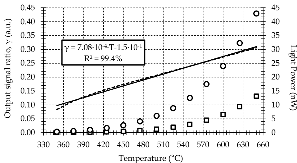
Figure 4. Calibration curve for: ( \square ) 1.3 \mu\text{m} ; ( \circ ) 1.55 \mu\text{m} ; (–) 1.3/1.55 \mu\text{m} .
