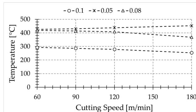
Figure 9. Temperature evolution of the new machined surface as a function of the feed rate: (*) 0.05 mm; (Δ) 0.08 mm; (○) 0.1 mm.
