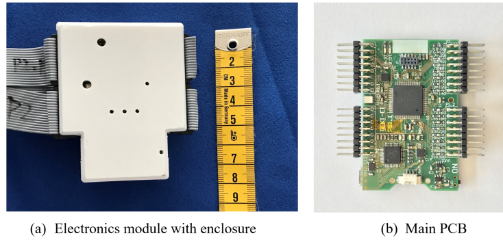
Figure 2. Electronic Hardware
