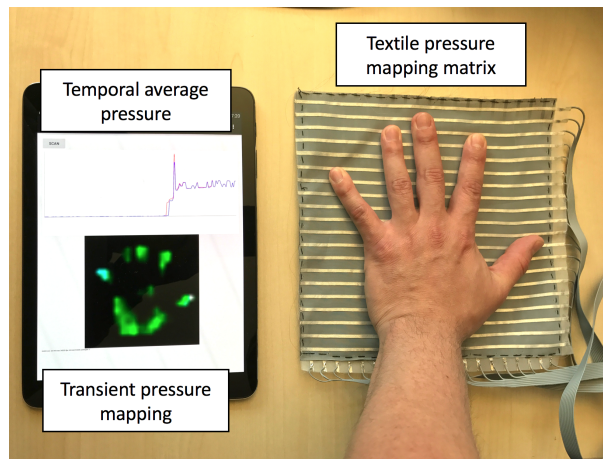
Figure 3. Realtime data visualization with a hand pressed on the textile pressure mapping matrix.
