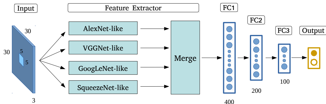
Figure 10. Ensemble Convolutional Neural Networks.
