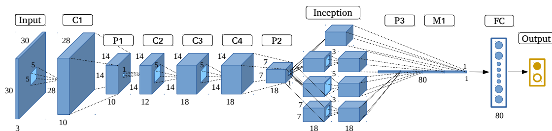
Figure 8. GoogleNet-like architecture.
