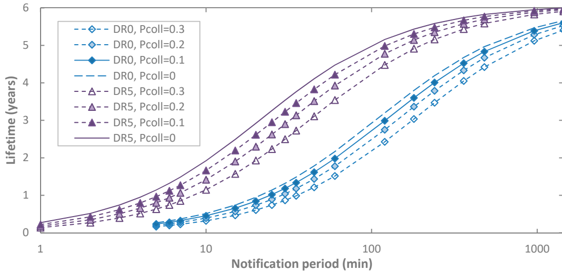
Figure 17. Impact of p_{coll} on end-device lifetime in acknowledged transmission, as a function of T_{Notif} , for different DR settings, and for BER = 0.
