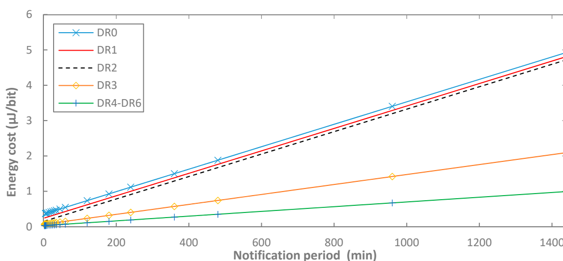
Figure 18. Energy cost of data delivery as a function of T_{Notif} , for different DR settings, and for BER = 0 and p_{coll} = 0 . Results for DR4, DR5 and DR6 overlap in the figure.
