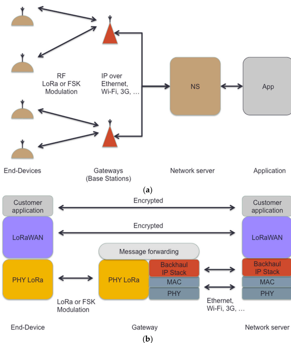
Figure 1. LoRaWAN (a) system and (b) protocol architecture.
