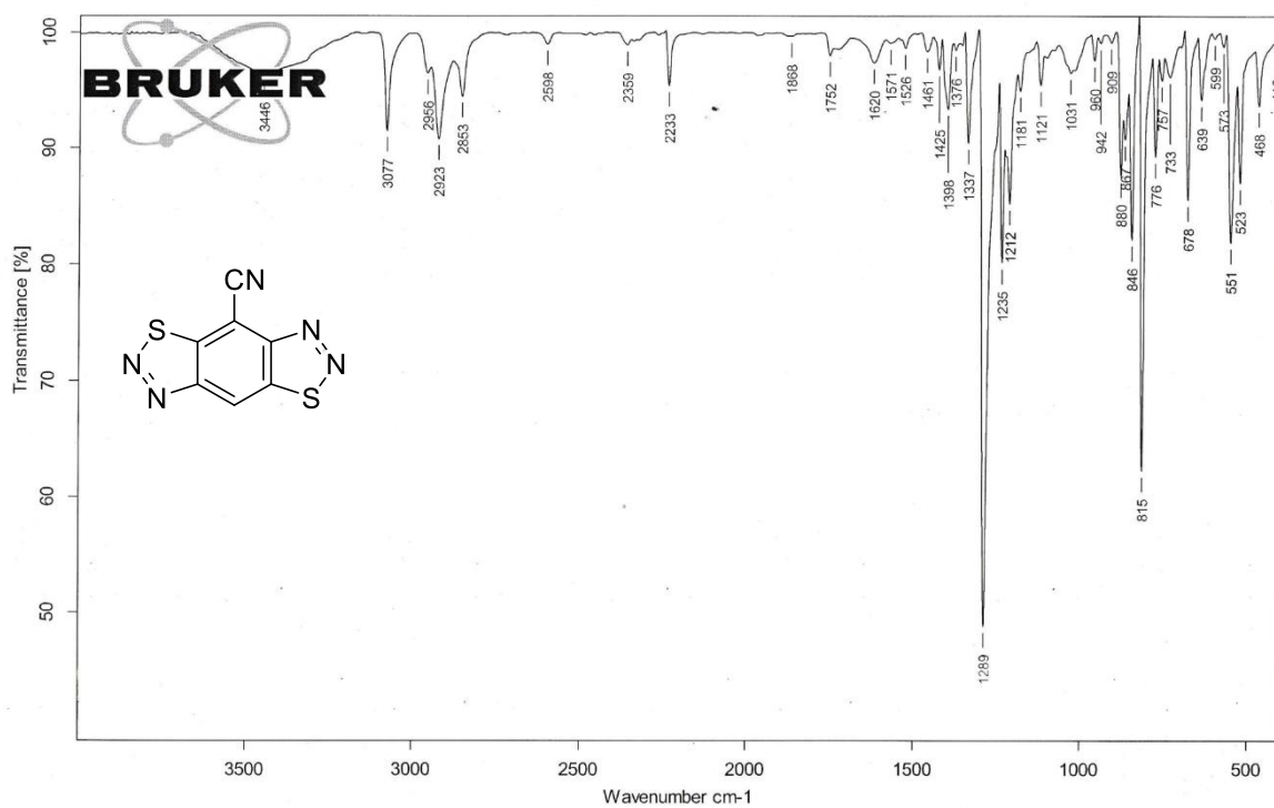
Figure S3. IR spectrum of benzo[1,2-d:4,5-d']bis([1,2,3]thiadiazole)-4-carbonitrile 1 .
