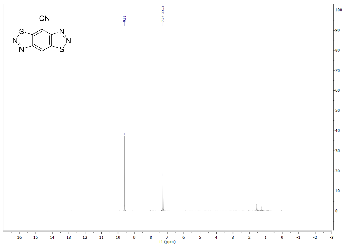
Figure S1. 1 H NMR spectrum of benzo[1,2- d :4,5- d' ]bis([1,2,3]thiadiazole)-4-carbonitrile 1 .
