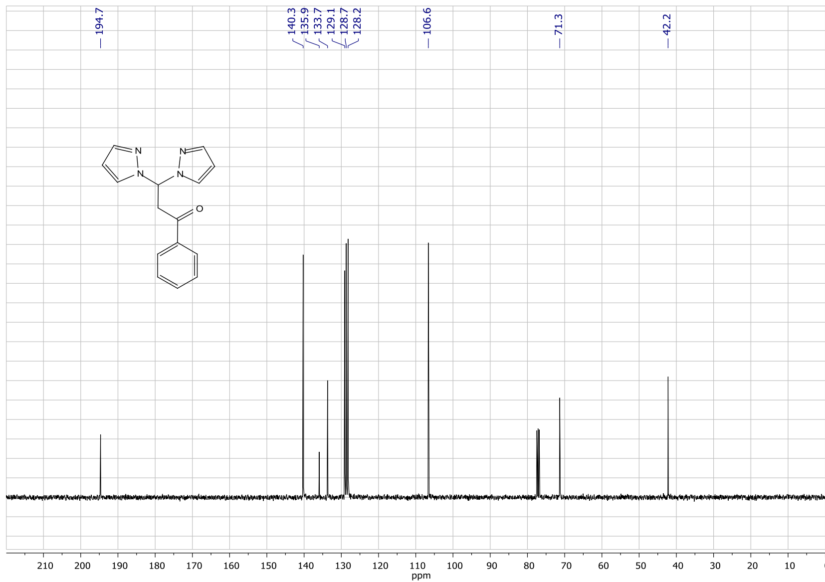
Figure S2. 13 C NMR spectrum of 1-phenyl-3,3-di(1H-pyrazol-1-yl)propan-1-one (3) in CDCl 3 .
