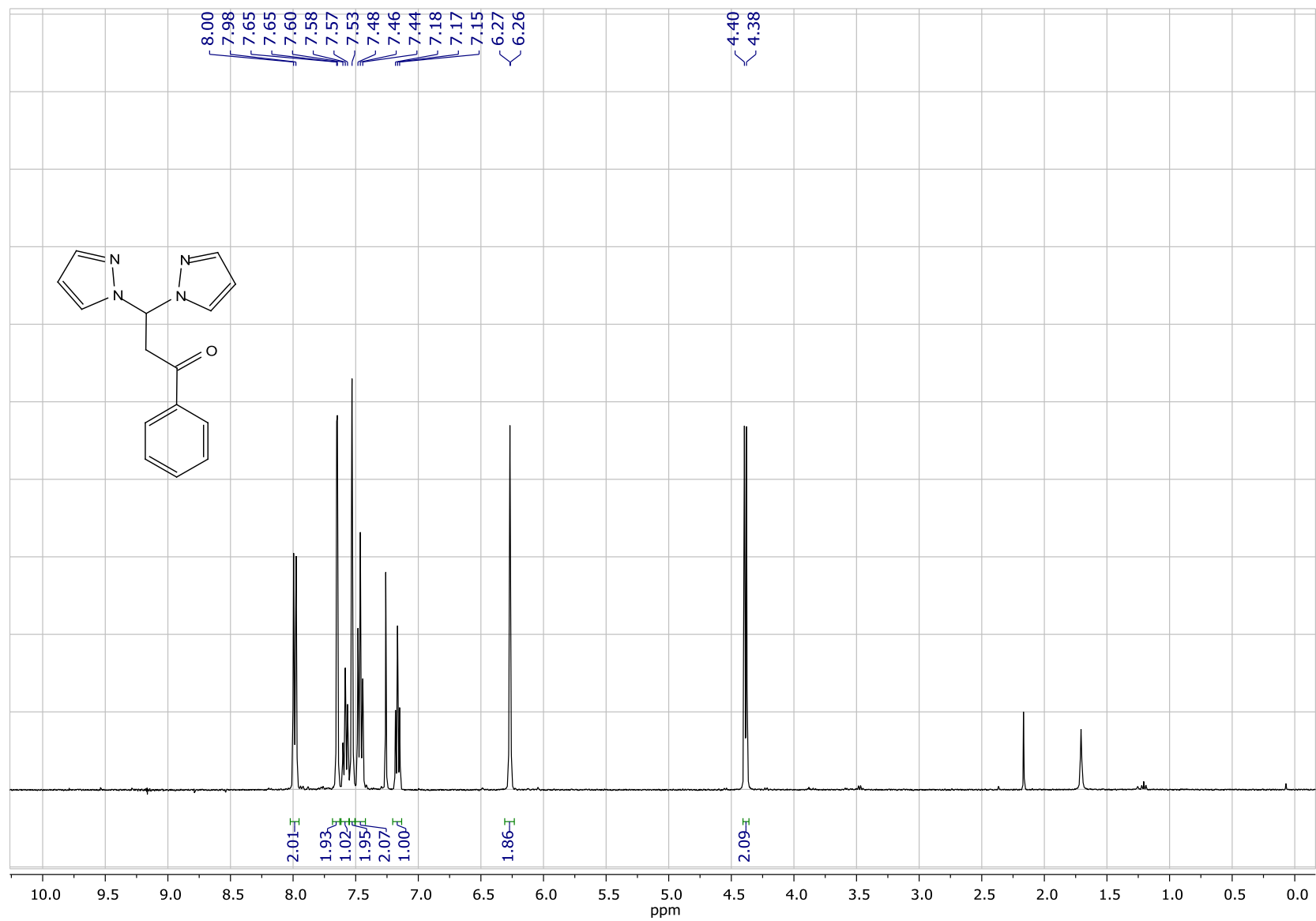
Figure S1. 1 H NMR spectrum of 1-phenyl-3,3-di(1H-pyrazol-1-yl)propan-1-one (3) in CDCl 3 .
