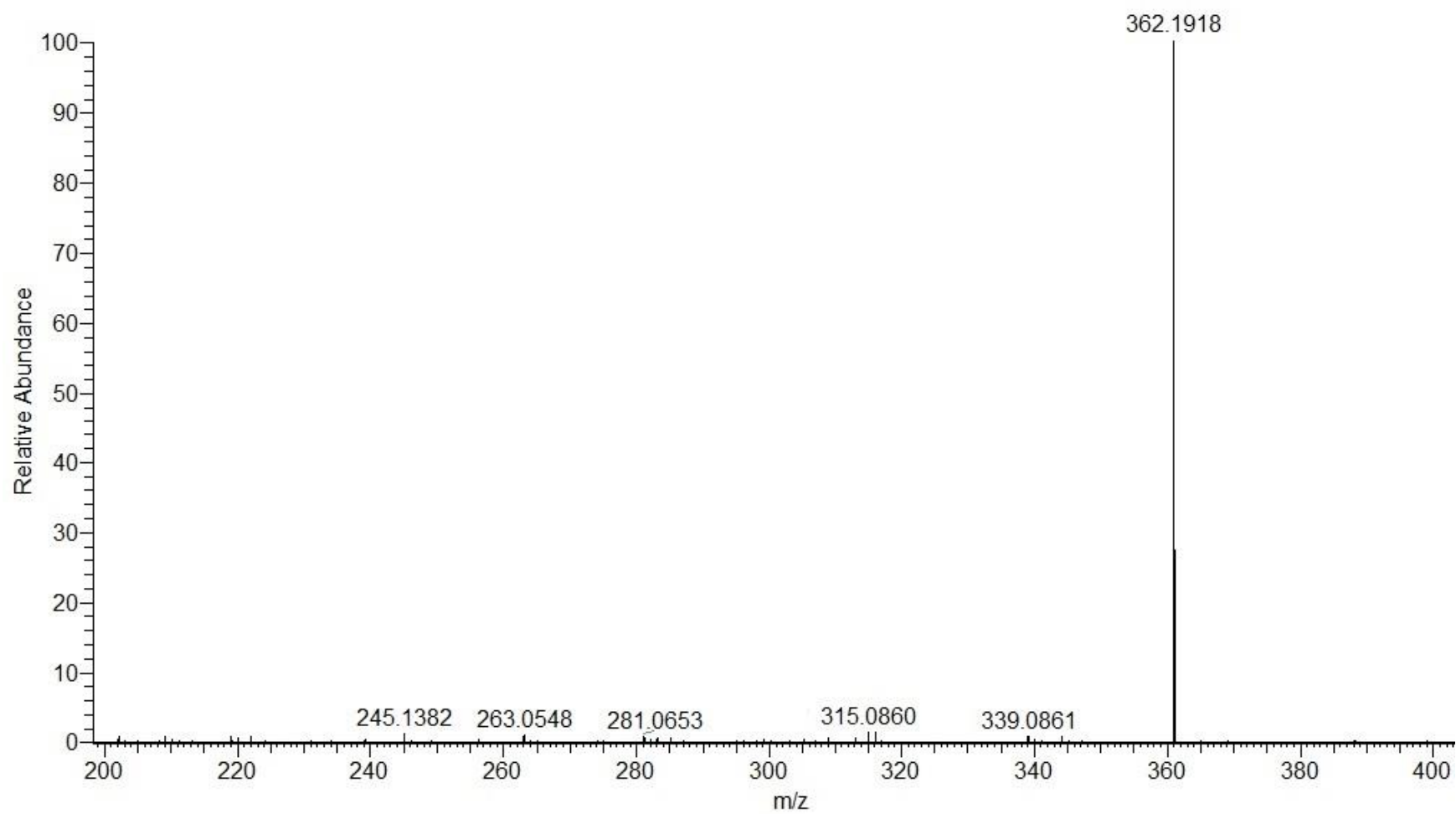
Figure S4. ESI-HRMS of compound 3 .
