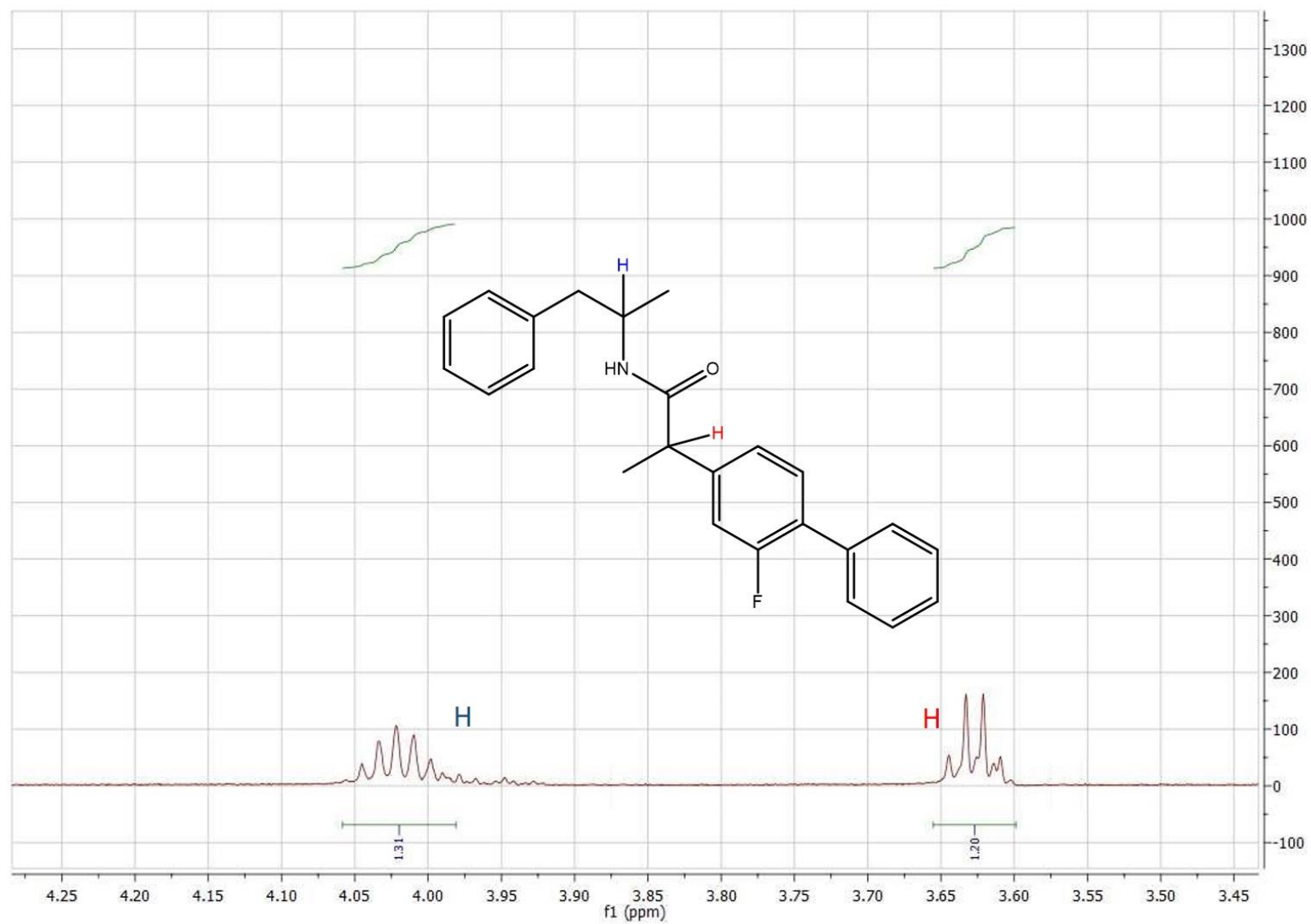
Figure S1b. Part of ^1\text{H} -NMR spectrum of compound 3 .
