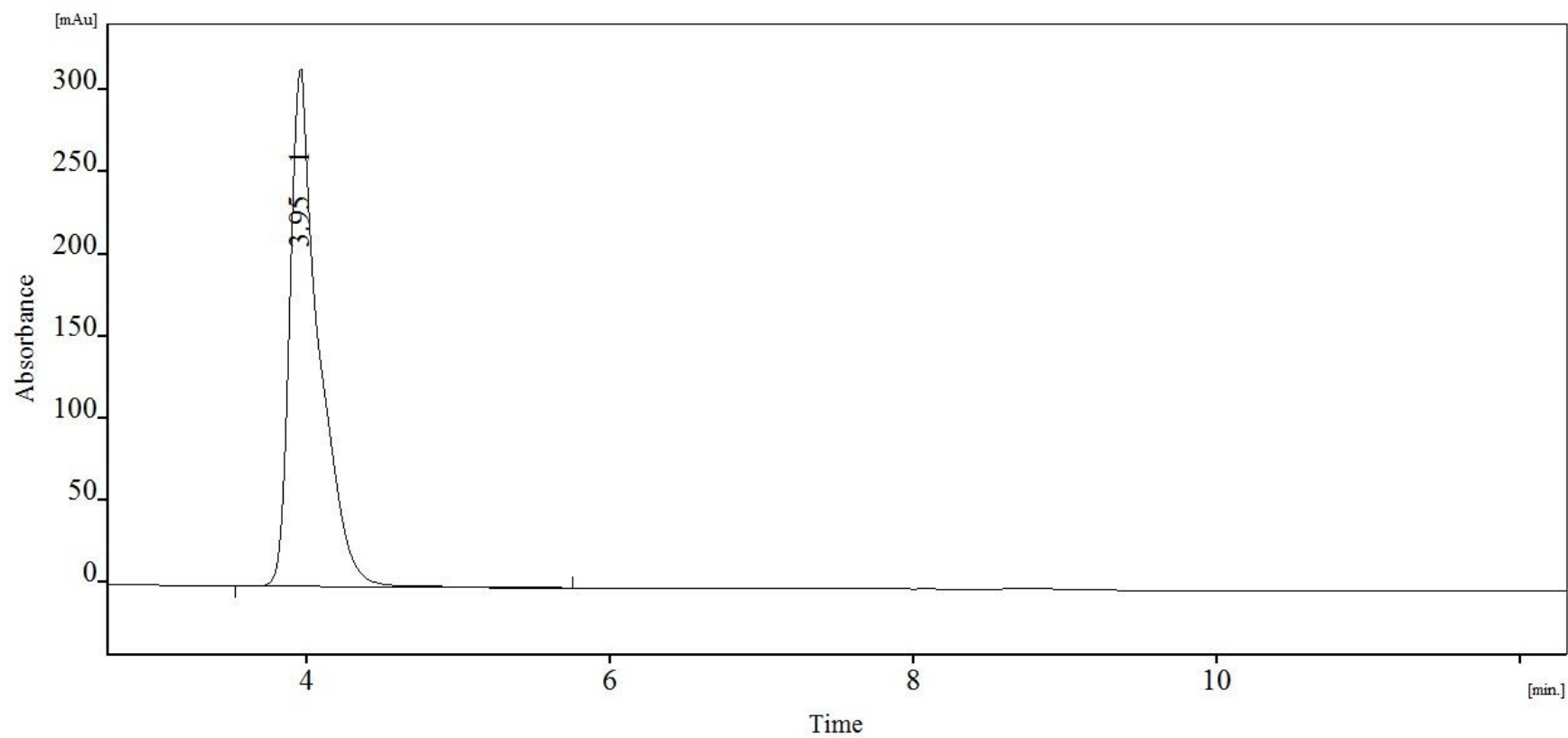
Figure S6. HPLC chromatogram of compound 3 .
