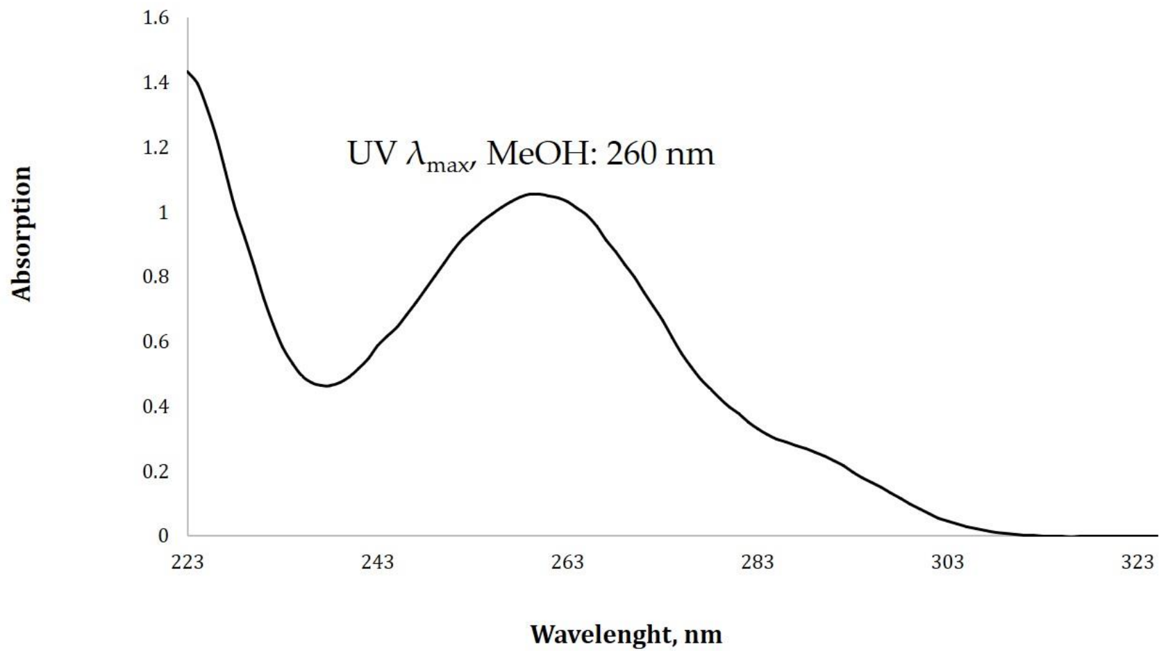
Figure S3. UV spectrum of compound 3.
