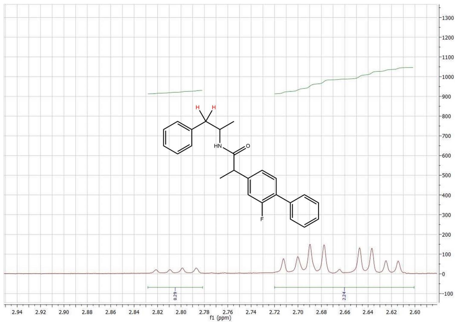
Figure S1a. Part of ^1\text{H} -NMR spectrum of compound 3 .
