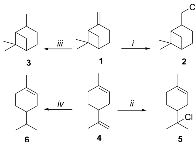
Scheme 1. (i) (1) \text{NaBH}_4 , \text{Me}_2\text{SO}_4 , THF, 24 h, rt. (2) \text{NaOH} , \text{H}_2\text{O}_2 , 12 h, rt. (3) \text{PPh}_3 , \text{CCl}_4 , 24 h, reflux; (ii) \text{SOCl}_2 , \text{SiO}_2 , \text{CH}_2\text{Cl}_2 , 12 h, rt; (iii) Pd/C, 2.75 MPa, rt; (iv) Pd/ \text{Al}_2\text{O}_3 , \text{H}_2\text{O} , 2.75 MPa, rt.
