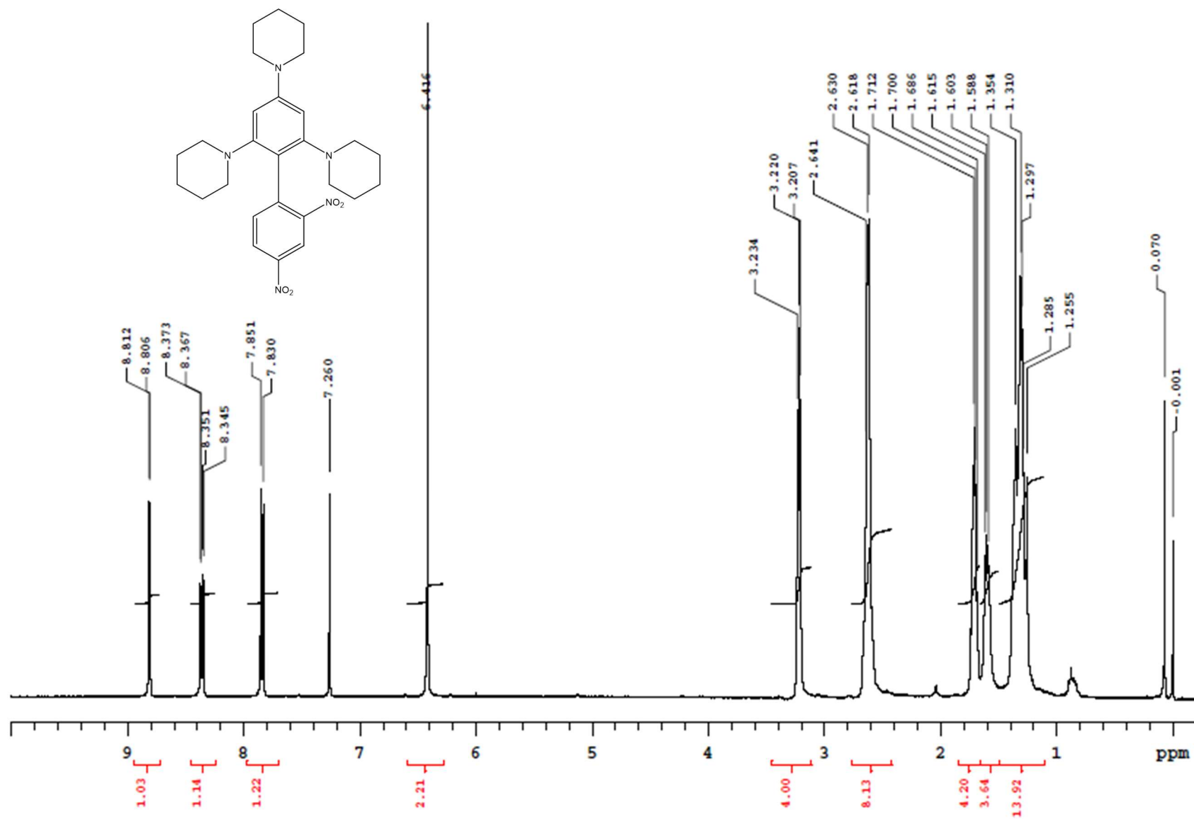
Figure S1. 1 H NMR spectrum in CDCl 3 of compound 4.
