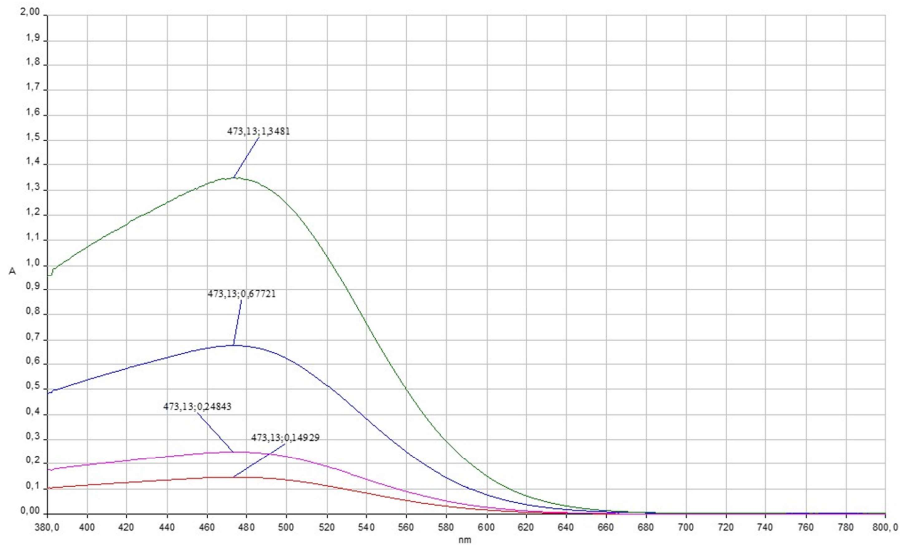
Figure S6. UV-Vis spectrum of compound 4 (at different concentrations).
