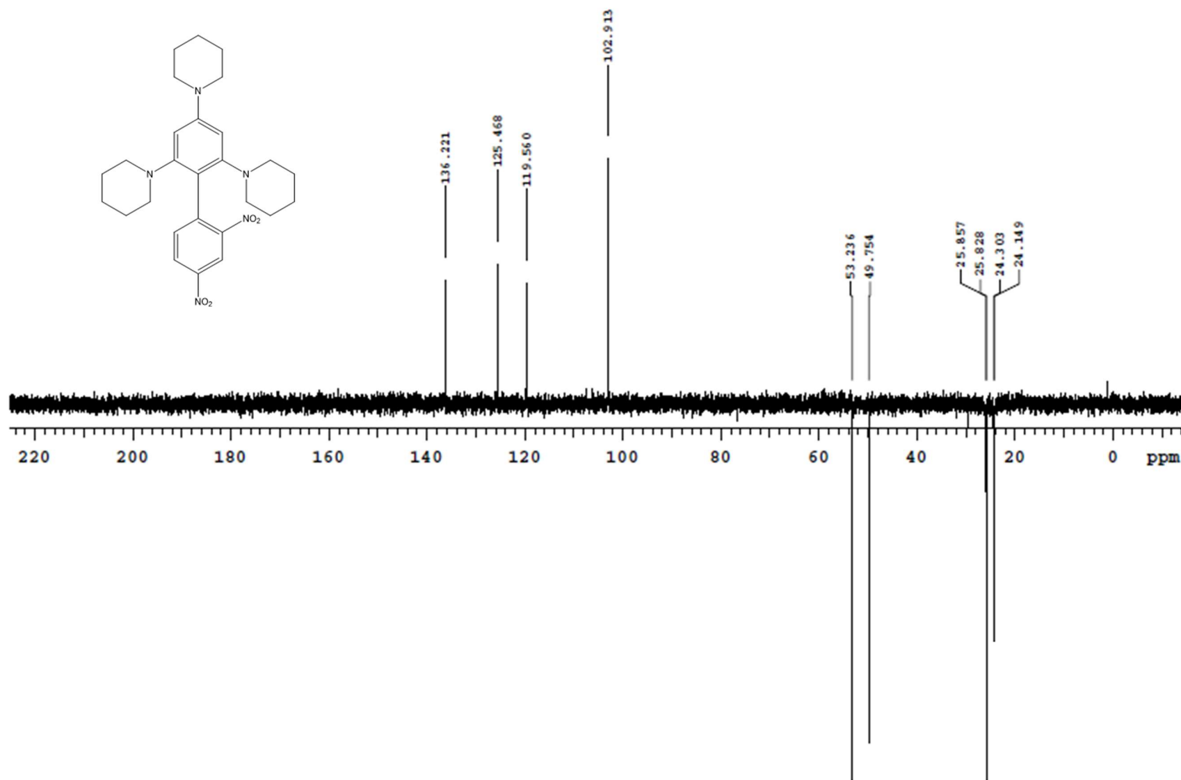
Figure S3. DEPT spectrum in CDCl 3 of compound 4.
