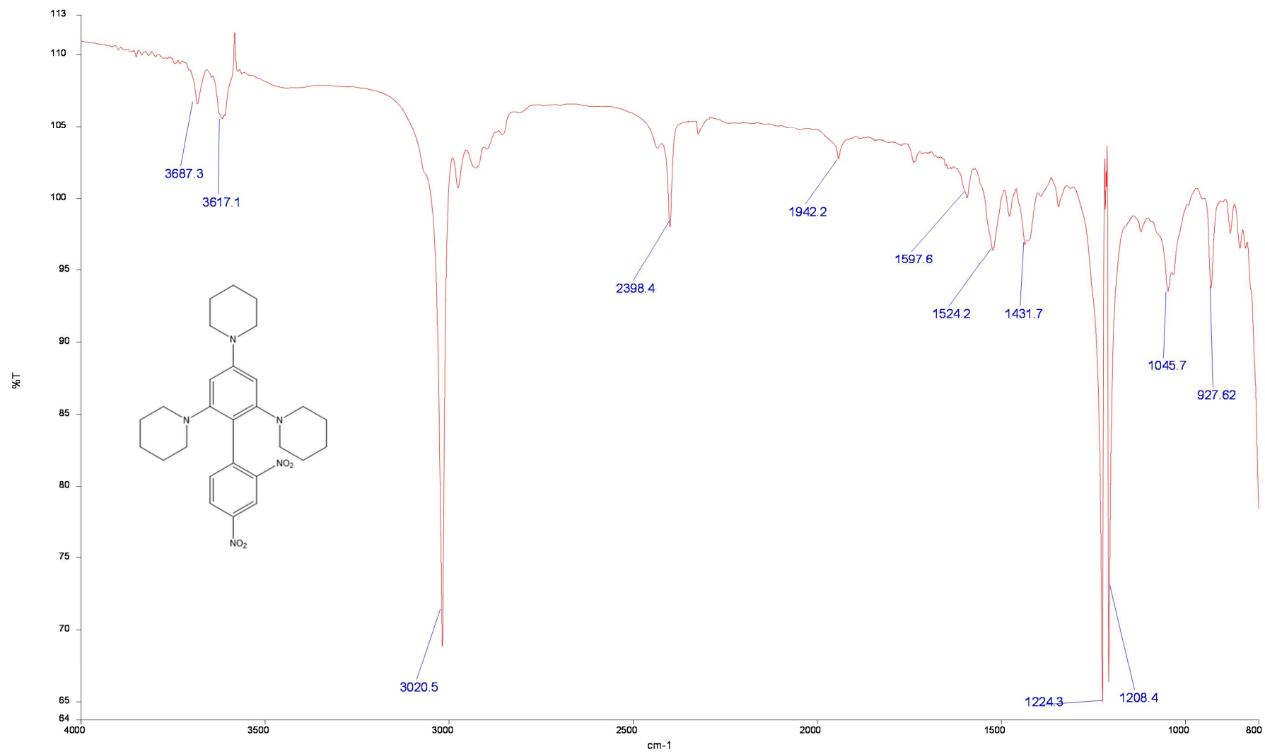
Figure S5. FT-IR spectrum of compound 4 .
