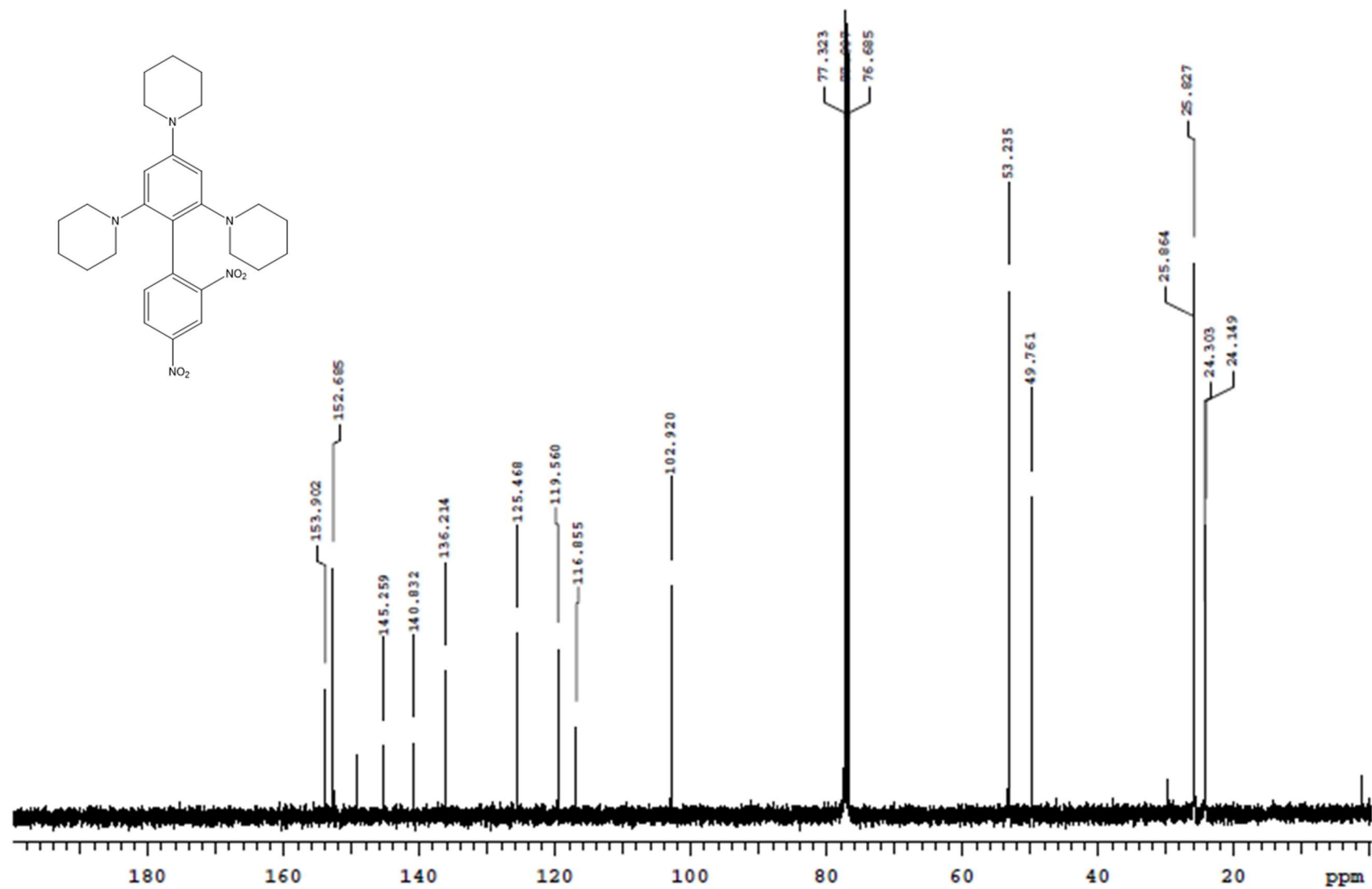
Figure S2. 13 C NMR spectrum in CDCl 3 of compound 4 .
