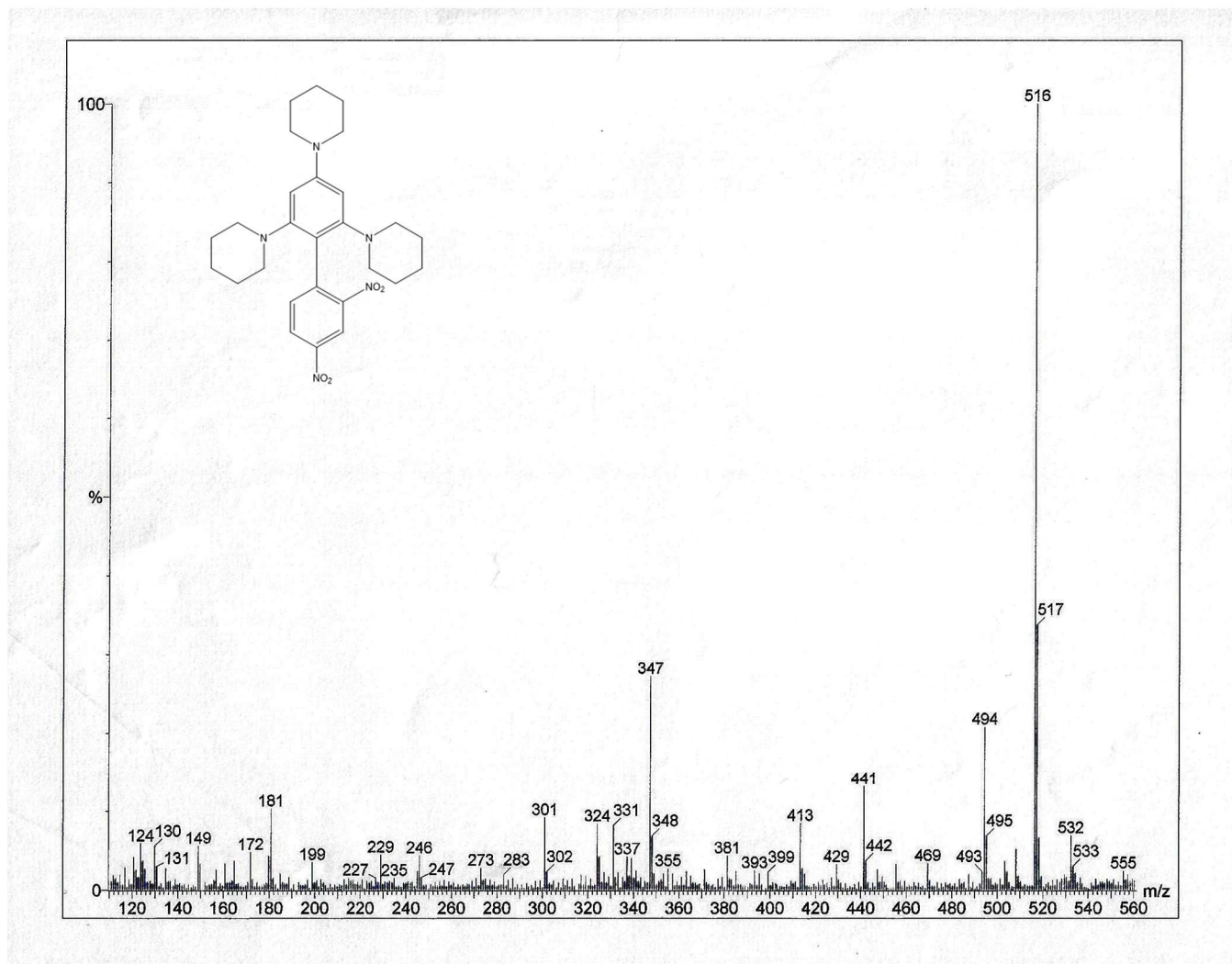
Figure S4. ESI-MS + spectrum of compound 4.
