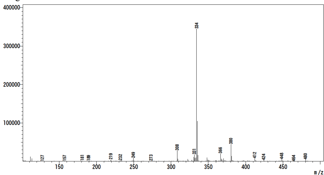
Figure S15 DUIS mass spectrum of 10 .
