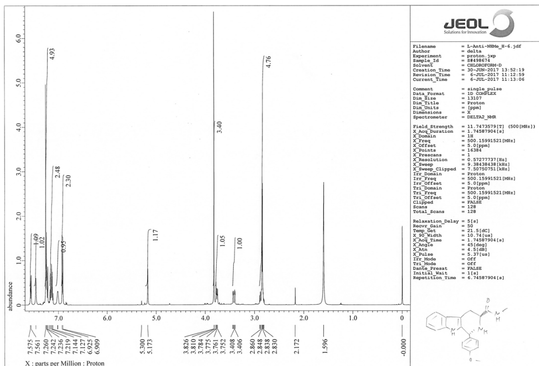
Figure S16 1 H-NMR spectrum of 11 .
