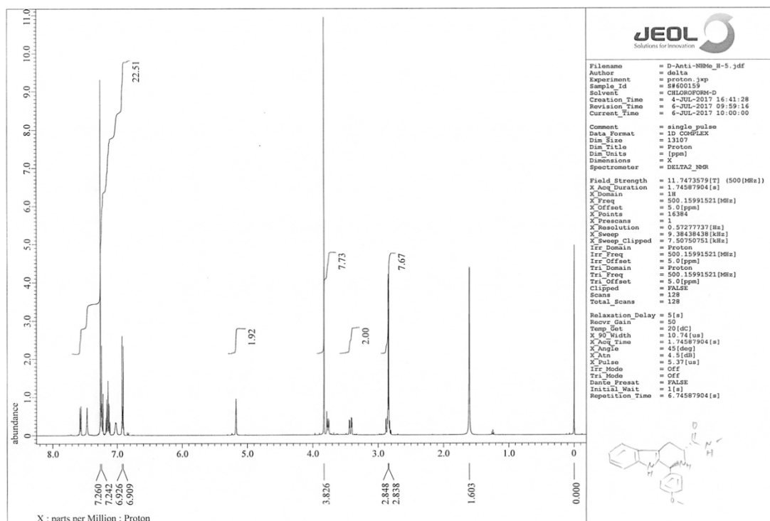
Figure S6 ^1\text{H} -NMR spectrum of 9 .
