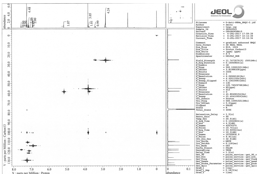
Figure S9 HMQC spectrum of 9 .
