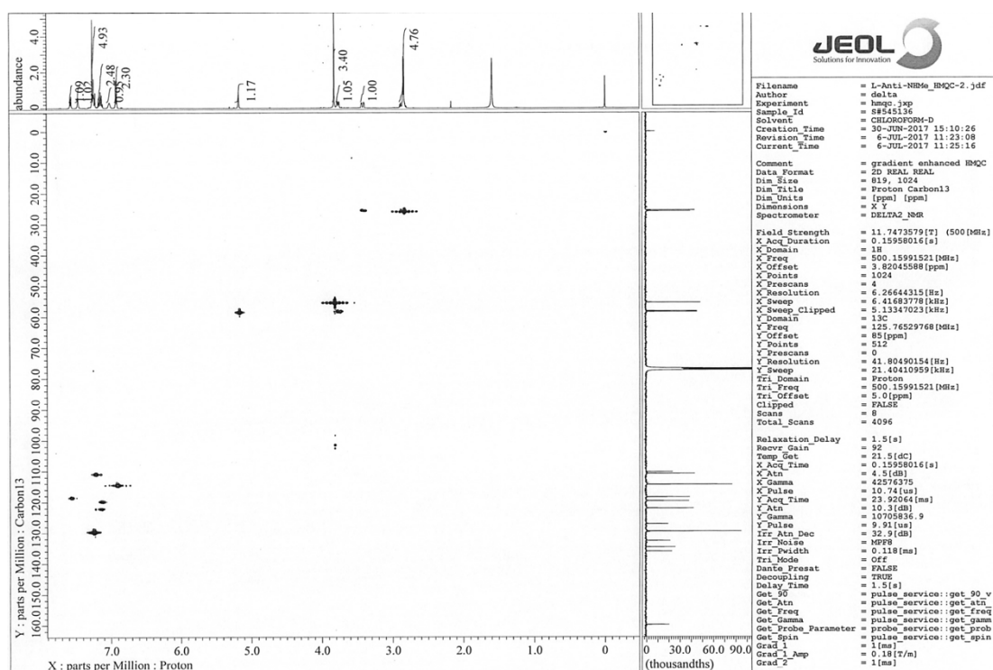
Figure S14 HMQC spectrum of 10 .
