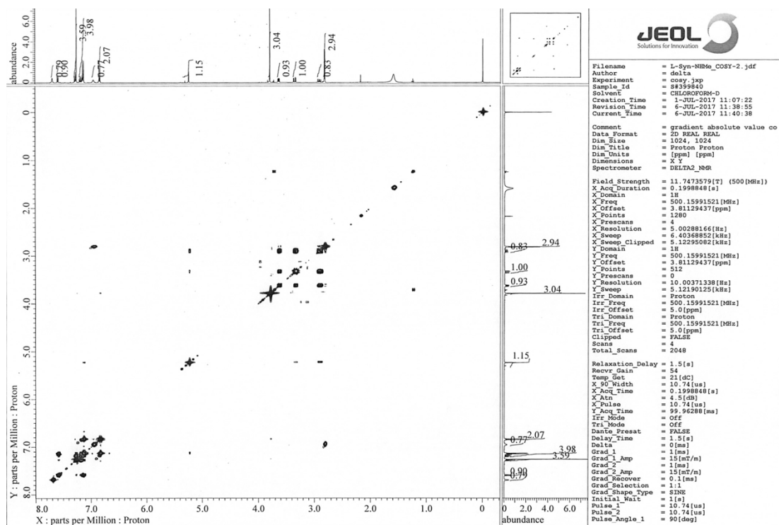
Figure S18 H-H-COSY spectrum of 11 .
