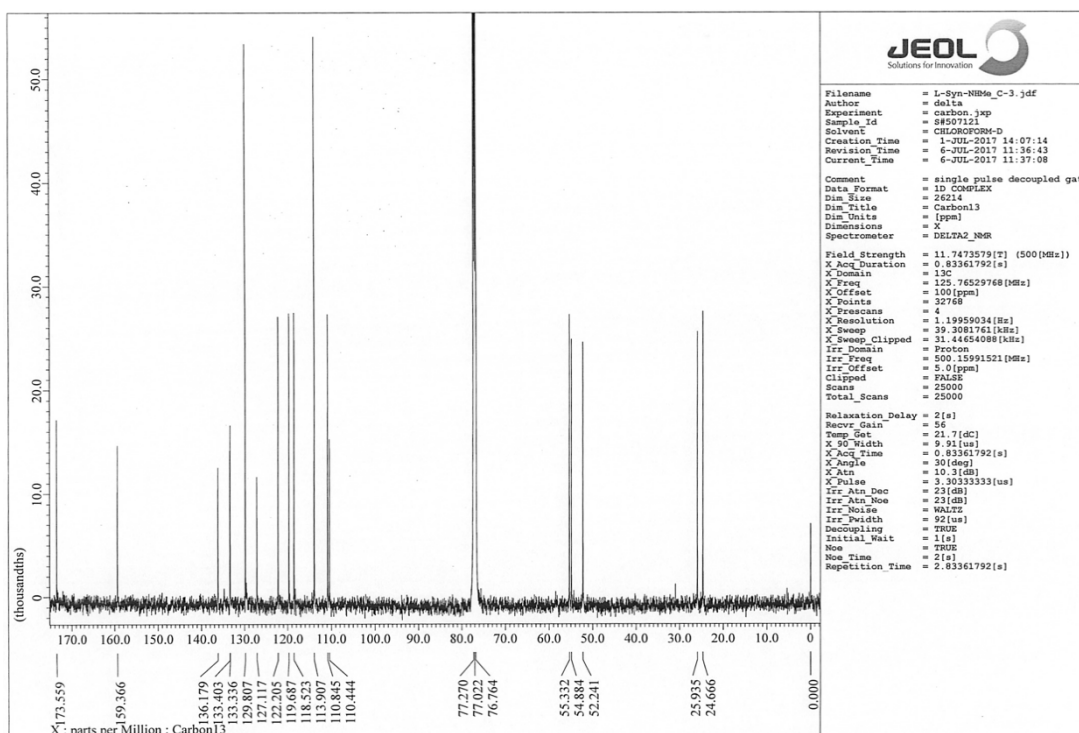
Figure S12 ^{13}\text{C} -NMR spectrum of 10 .
