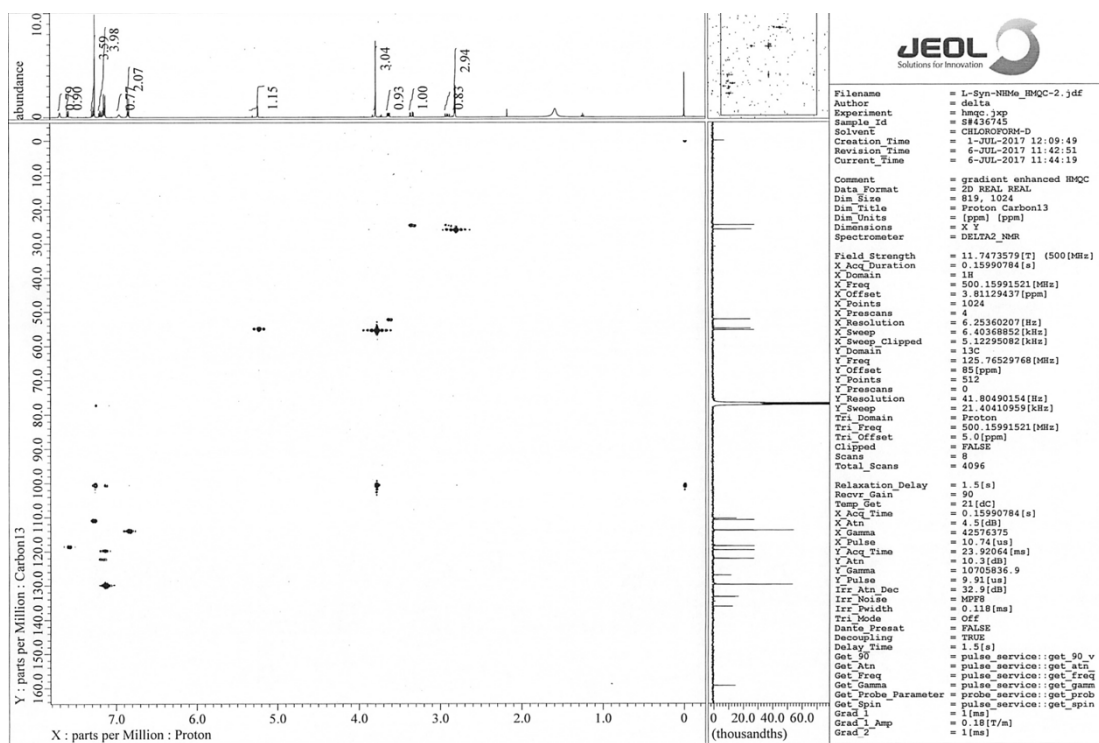
Figure S19 HMQC spectrum of 11 .
