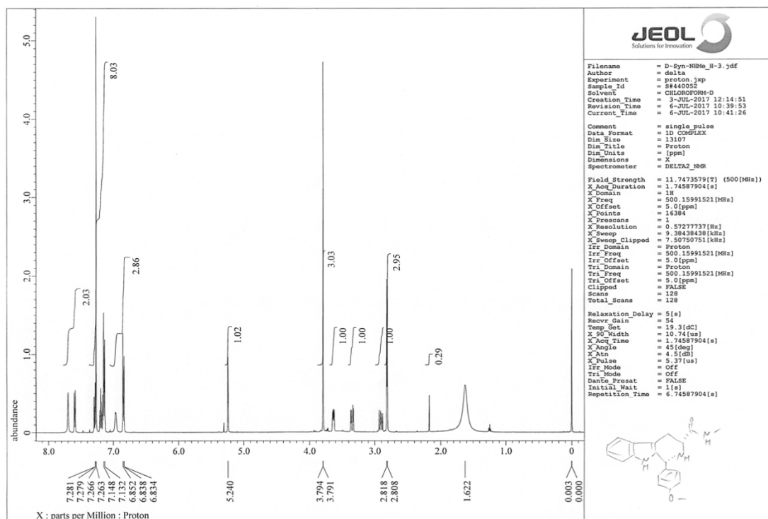
Figure S1 1 H-NMR spectrum of 8 .
