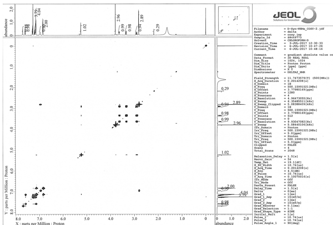
Figure S3 H-H-COSY spectrum of 8 .
