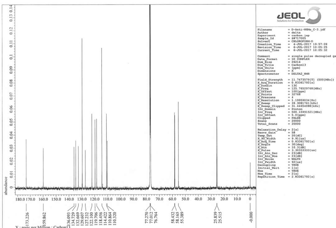
Figure S7 ^{13}\text{C} -NMR spectrum of 9 .
