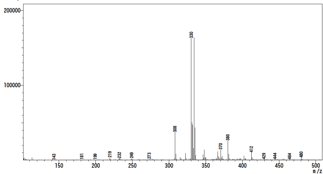
Figure S20 DUIS mass spectrum of 11 .
