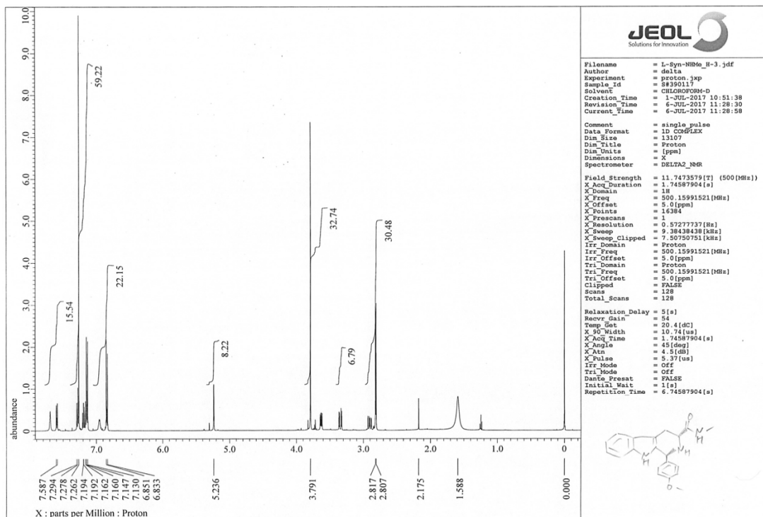
Figure S11 ^1\text{H} -NMR spectrum of 10 .
