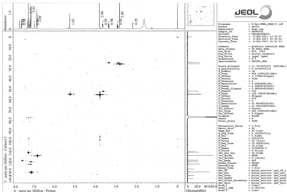
Figure S4 HMQC spectrum of 8 .
