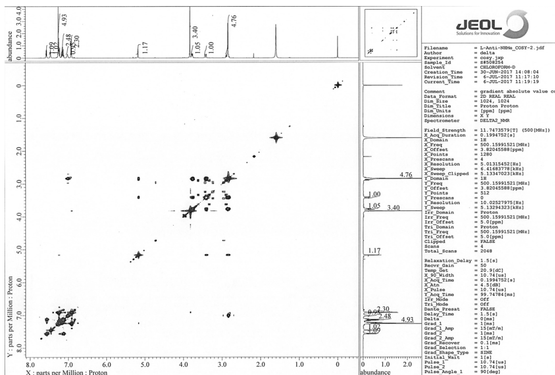
Figure S13 H-H-COSY spectrum of 10 .
