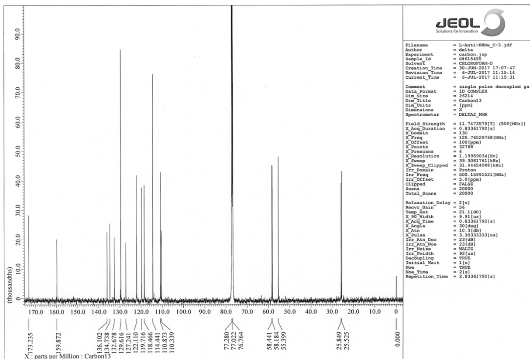
Figure S2 13 C-NMR spectrum of 8 .
