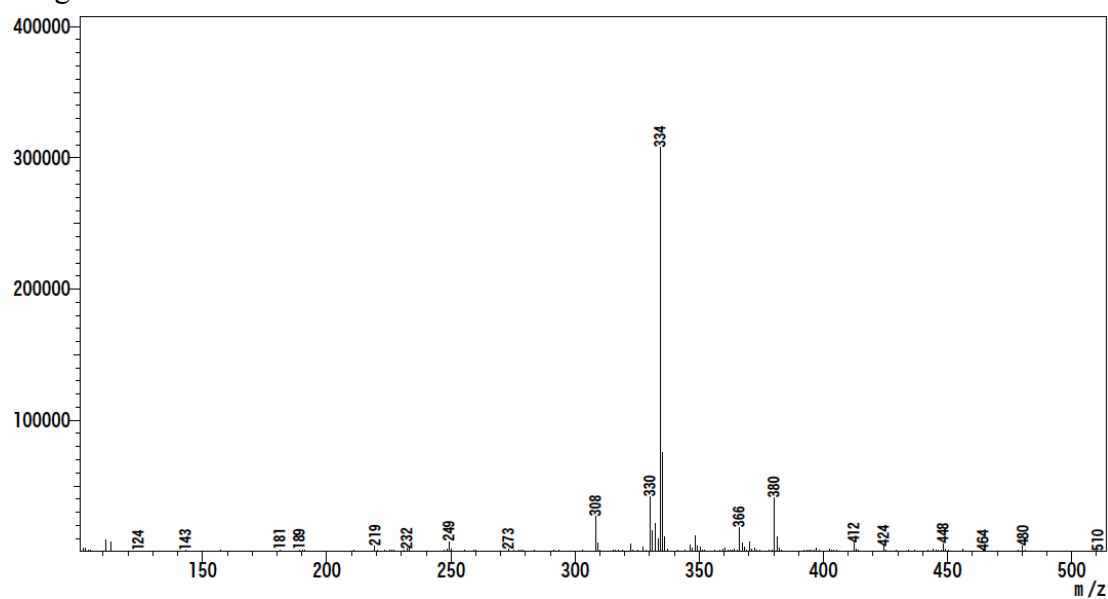
Figure S10 DUIS mass spectrum of 9 .
