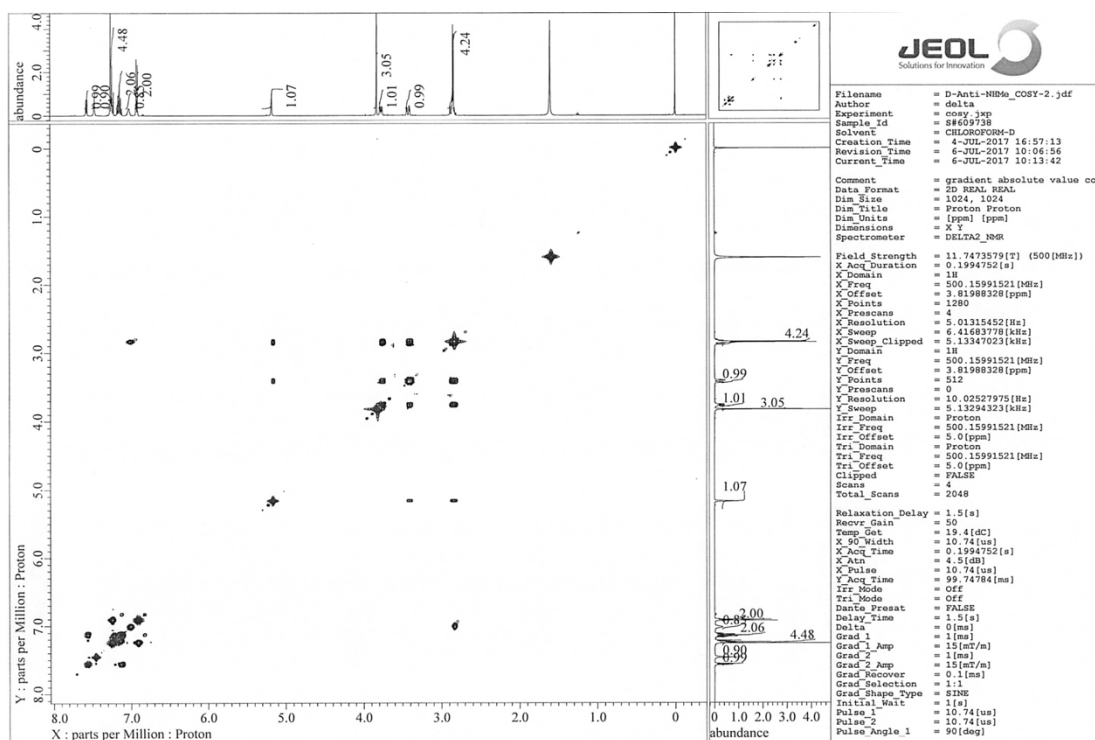
Figure S8 H-H-COSY spectrum of 9 .
