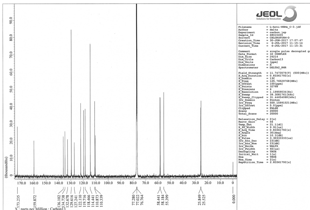
Figure S17 13 C-NMR spectrum of 11 .
