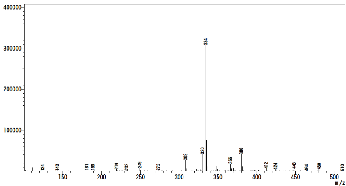
Figure S5 DUIS mass spectrum of 8 .
