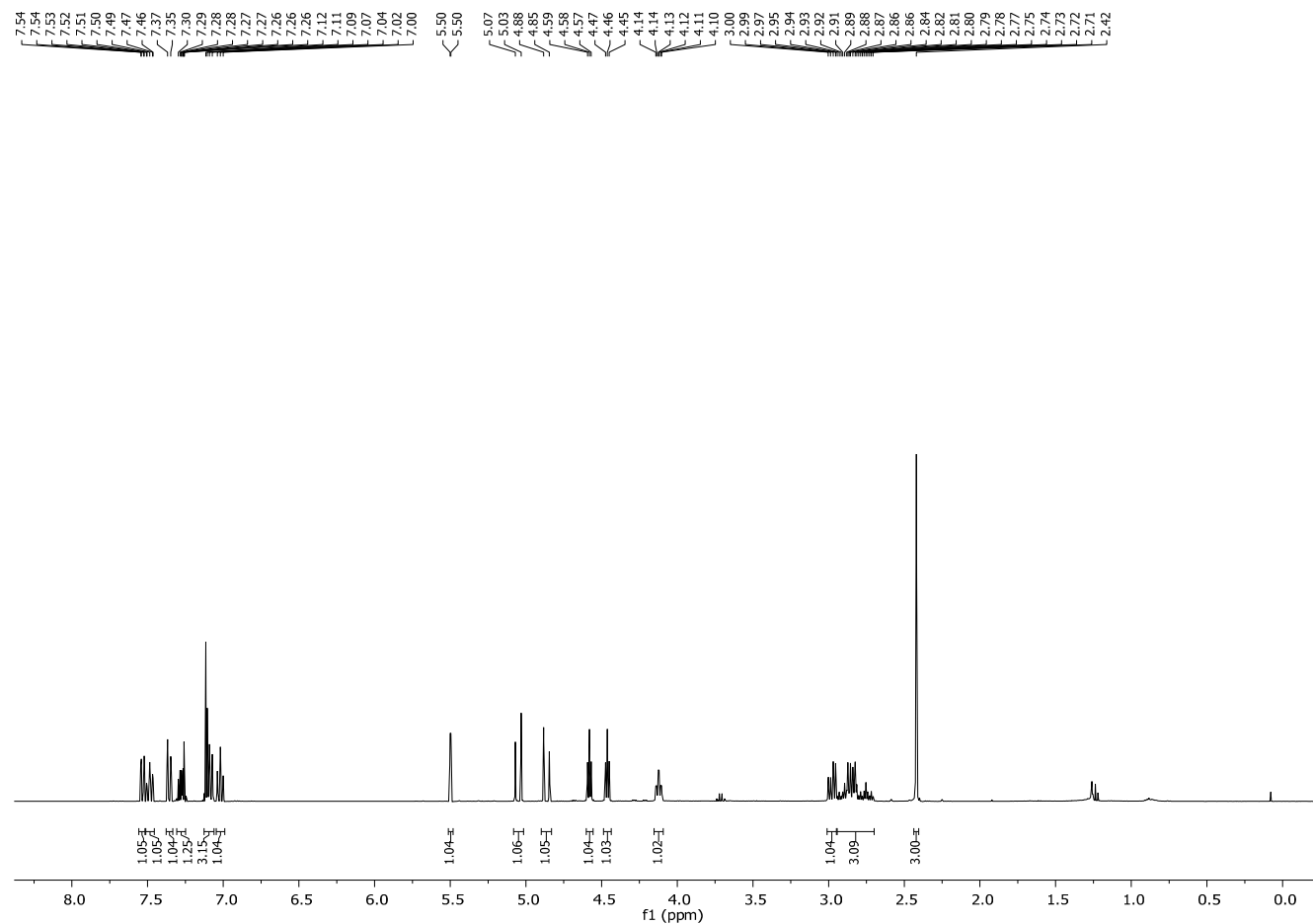
Figure S1. ^1\text{H} -NMR of 2-Fluoro- N -methyl- N -({(3 S ,4 S )-4-[2-(trifluoromethyl)phenoxy]-3,4-dihydro-1 H -isochromen-3-yl} methyl)ethanamine.
