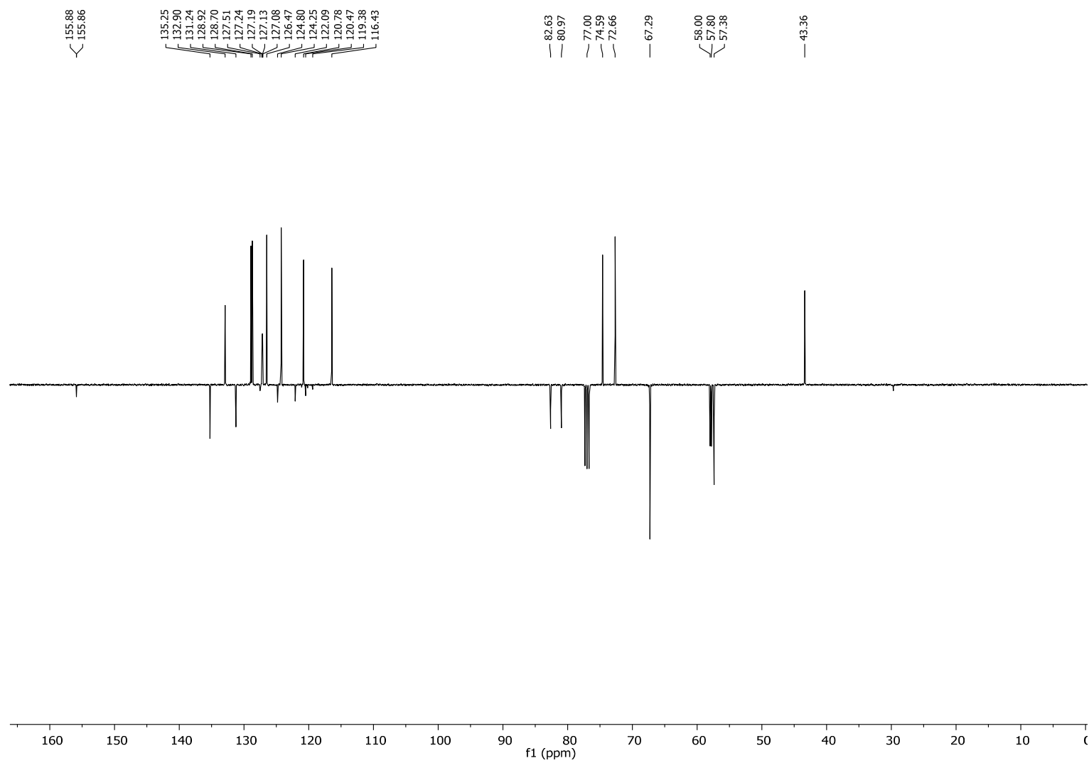
Figure S2. 13 C-NMR of 2-Fluoro-N-methyl-N-({(3S,4S)-4-[2-(trifluoromethyl)phenoxy]-3,4-dihydro-1H-isochromen-3-yl}methyl)ethanamine.
