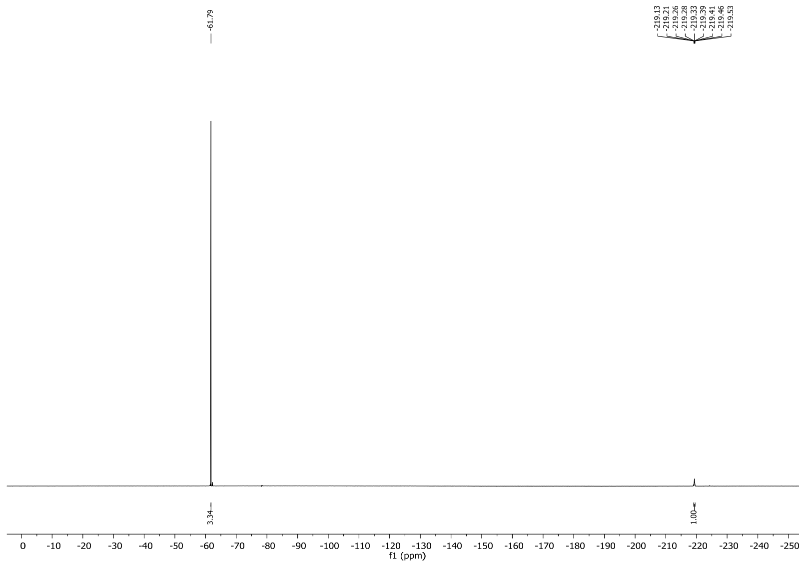
Figure S3. ^{19}\text{F} -NMR of 2-Fluoro- N -methyl- N -({(3 S ,4 S )-4-[2-(trifluoromethyl)phenoxy]-3,4-dihydro-1 H -isochromen-3-yl}methyl)ethanamine.
