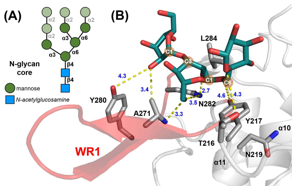
Figure 5. The \beta -wing region 1 (WR1) of CtGH76. (A) Diagram of the high-mannose core of fungal N-glycans, with \alpha 1,3- \alpha 1,6-mannotriose substructures highlighted in dark green. SNFG symbols in the bottom left corner denote its building blocks. (B) Stick model of \alpha 1,3- \alpha 1,6-mannotriose (green) and its interacting residues within CtGH76's structure. The WR1 region is highlighted in red, with the remaining structure in grey.
