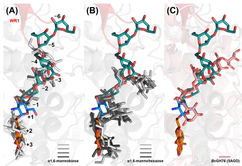
Figure 6. Comparison of predicted and observed CtGH76–glycan complex models. Superposition of predicted stick models for (A) \alpha 1,6-mannobioses (light to heavy grey), (B) \alpha 1,6-mannohexaoses (light to heavy grey), and observed (C) \alpha 1,6-mannopentaose (5AGD, pink) with the observed CtGH76–glycan complex (9R4R, blue; 9R4P and 9R4N, dark green; 9R4S, orange). The WR1 region is highlighted in red, with the remaining structure in grey.
