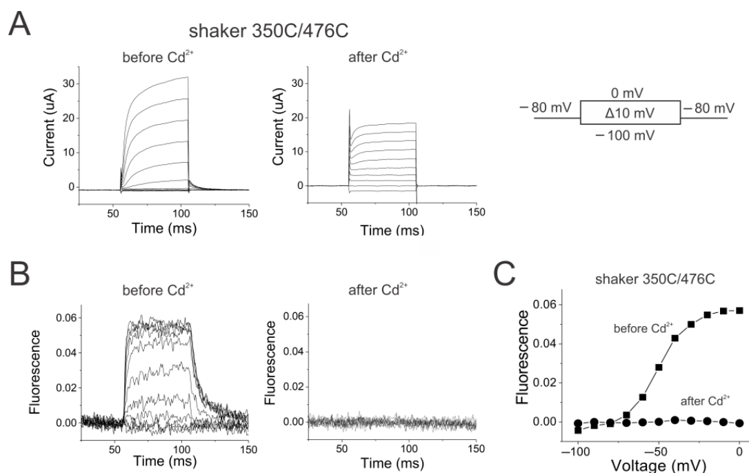
Figure 3. Locking the activation gate open in Shaker channels prevents S4 movement. (A) Shaker 350C/476C currents (left) before and (right) after injection of the oocyte with 50 nL of 10 \mu M CdCl 2 in response to voltage steps from -100 mV to 0 mV from a holding potential of -80 mV with a tail potential of -80 mV. (B) Shaker 350C/476C fluorescence (left) before and (right) after injection of the oocyte with 50 nL of 10 mM CdCl 2 in response to voltage steps in Figure 3A. (C) FV relations before (squares) and after (circles) locking the channels open by Cd 2+ application on shaker 350C/476C channels.
