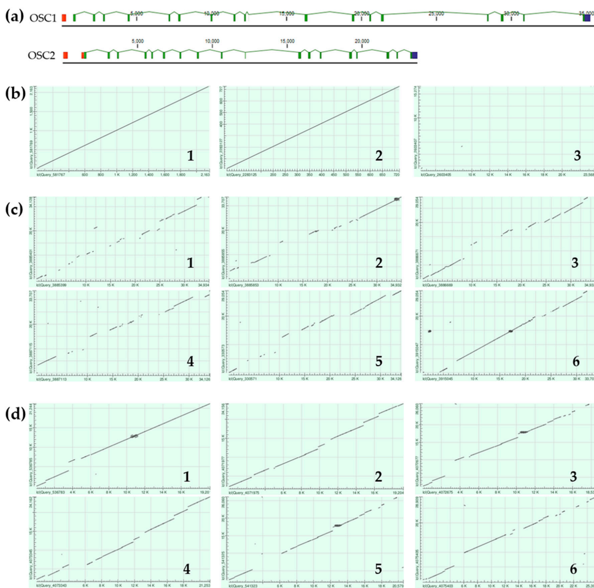
Figure 4. Comparison of E. fraudatrix OSCs gene structures and their haplotypes. (a) Gene structure schemes. (b) Scatter plots of OSC1 and OSC2 transcripts (1), deduced amino acid sequences (2), and
