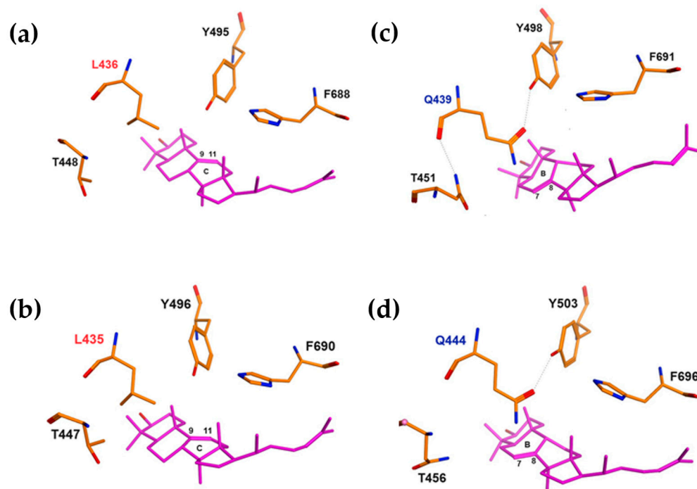
Figure 2. Molecular docking of triterpenoid in the active site of oxidosqualene cyclase. Functionally significant residues L436/L435 of Ef OSC1 (a) and Aj LAS1 (b) near the B and C rings of parkeol are shown in red. Functionally significant residues Q439/Q444 of Ef OSC2 (c) and Aj LAS2 (d) near the B ring of lanostadienol are shown by blue.
