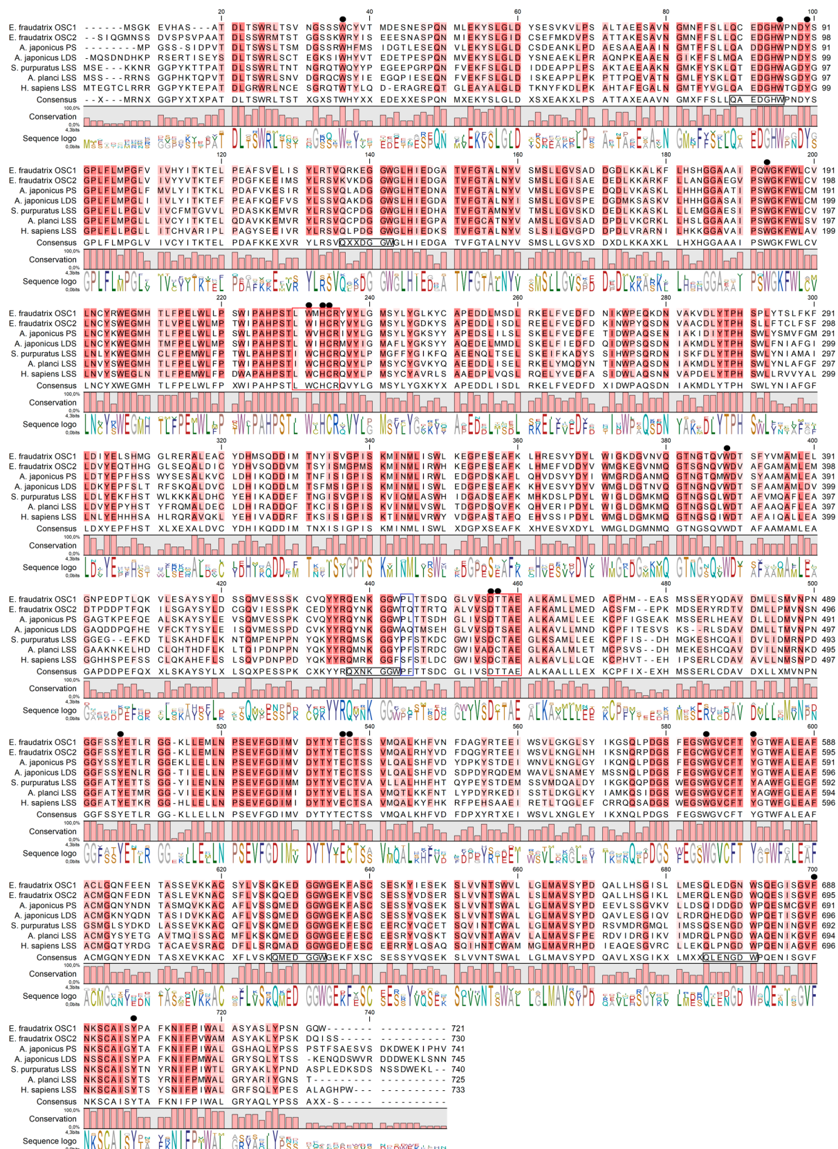
Figure 1. Alignment of OSCs proteins from sea cucumbers, sea urchin, starfish, and human. E. fraudatrix OSC1 and OSC2 (OR725688 and OR711403 in this study); A. japonicus LAS1 (PS) and LAS2 (LDS)
