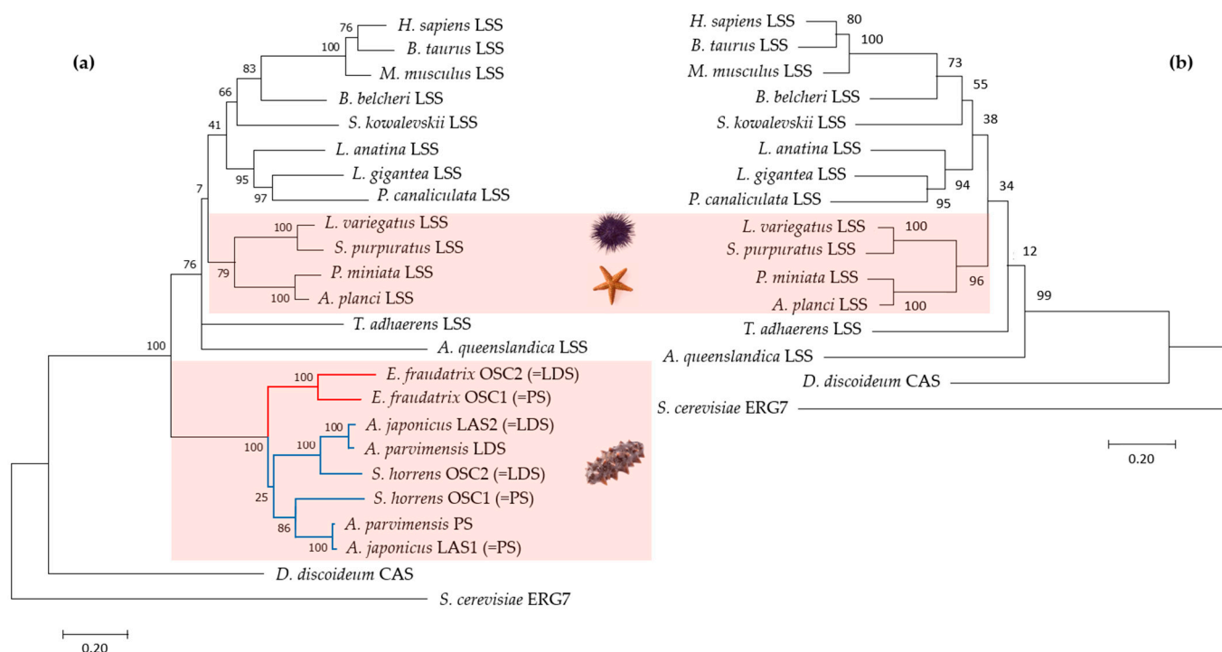
Figure 3. Maximum likelihood (ML) phylogenetic trees based on amino acid sequences of OSCs with (a) and without (b) sea cucumbers: H. sapiens (NM 002340.6), B. taurus (NM 001046564.1), M. musculus (XM 036155651.1), B. belcheri (XM 019790446.1), S. kowalevskii (XM 006825036.1), L. anatina (XM 013562424.1), L. gigantea (XM 009046756.1), P. canaliculata (XM 025240299.1), L. variegatus (XM 041622296.1), S. purpuratus (ON478349.1), P. miniata (ON478348.1), A. planci (XM 022227483.1), T. adhaerens (XM 002110738.1), A. queenslandica (XM 003383129.3), E. fraudatrix OSC1 (OR725688, this study), E. fraudatrix OSC2 (OR711403, this study), A. japonicus LAS1 (ON478352.1), A. japonicus LAS2 (ON478353.1), A. parvimensis PS (ON478351.1), A. parvimensis LDS (ON478350.1), S. horrens OSC1 [14], S. horrens OSC2 [14], D. discoideum (XM 641154.1), and S. cerevisiae (NP 011939.2).
