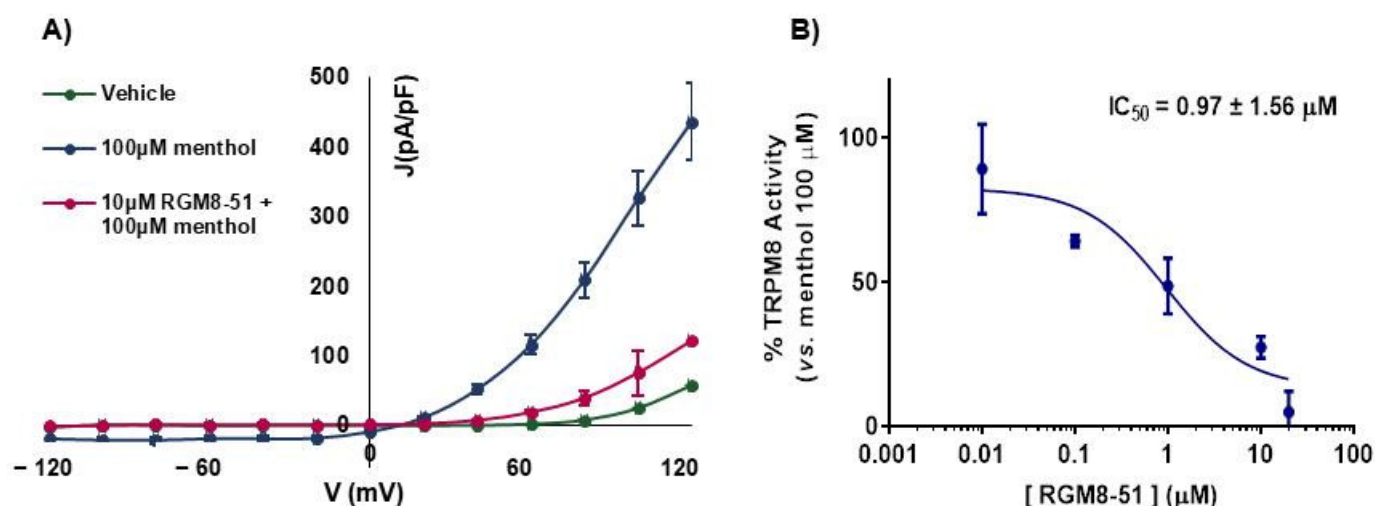
Figure 2. Compound 3 (RGM8-51) blocks TRPM8-mediated responses evoked by menthol in r TRPM8-expressing HEK293 cells. (A) IV curves obtained after exposure to vehicle solution (green trace), 100 \mu M menthol (blue trace), and 100 \mu M menthol + 10 \mu M RGM8-51 (red trace). Peak current data were expressed as pA/pF (to allow comparison among different size cells). Each point is the mean \pm SEM of n = 15 . (B) Concentration/response curves for r TRPM8 current blockade by RGM8-51, at a holding voltage of -60 mV. The solid line represents fits of the experimental data to the following binding isotherm: y = \max/(1 + x/IC_{50})^n , where x is the drug concentration and n the Hill coefficient. The fitted value for IC_{50} was 0.97 \pm 1.56 . Each point is the mean \pm SEM of n = 15 .
