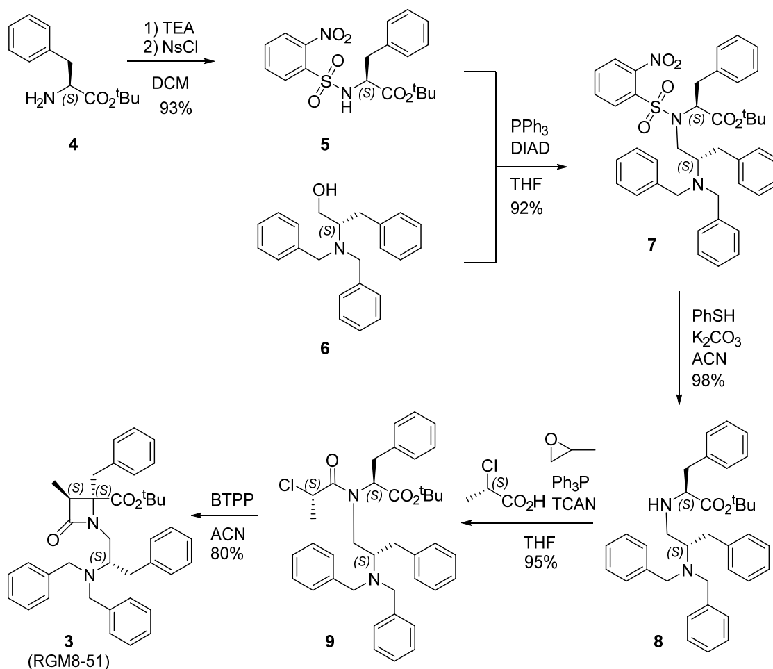
Scheme 1. Synthetic procedure for the preparation of β-lactam 3 (RGM8-51) from H-L-Phe-OtBu ( 4 ). Compounds 5–9 are the synthetic intermediates in the process.
