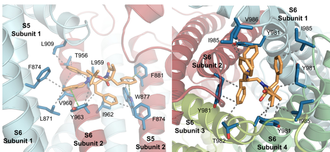
Figure 5. Interaction of \beta -lactam RGM8-51 (carbon atoms in wheat color) at subsite 1 (left) and subsite 2 (right). Channel residues involved in the interactions are shown in blue. VdW interactions are indicated by dotted gray lines, and \pi - \pi stacking by centroids and non-continuous pale green lines.
